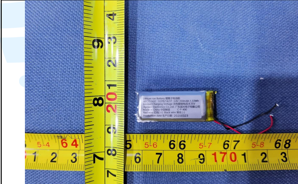
EUT Photo(AEC 751437)
