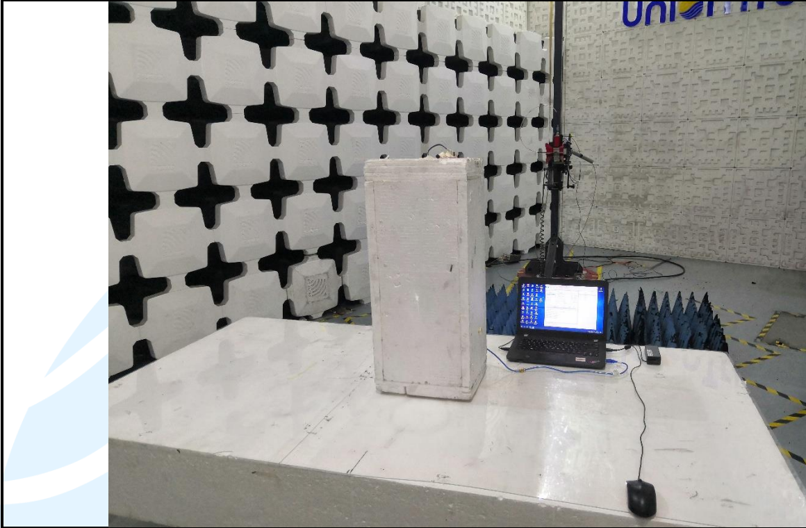
Radiated emission Test Setup (Above 1 GHz) -Left
