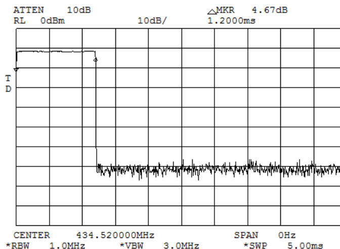
Plot 7.1.2 Transmission duration
