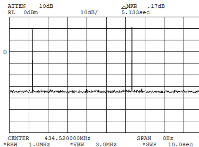
Plot 7.2.24 Transmission pulse period
