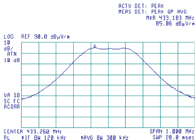
Plot 7.2.2 Radiated emission measurements at the fundamental frequency 433.26 MHz
