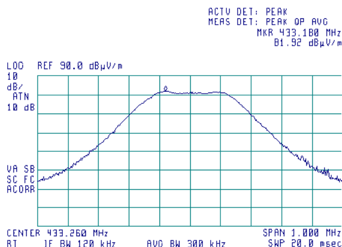
Plot 7.2.6 Radiated emission measurements at the fundamental frequency 433.26 MHz
