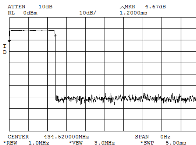
Plot 7.2.23 Transmission pulse duration
