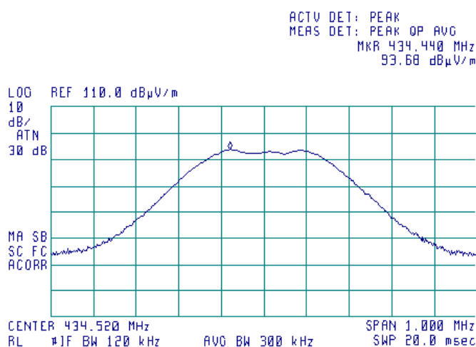
Plot 7.2.12 Radiated emission measurements at the fundamental frequency 434.52 MHz
