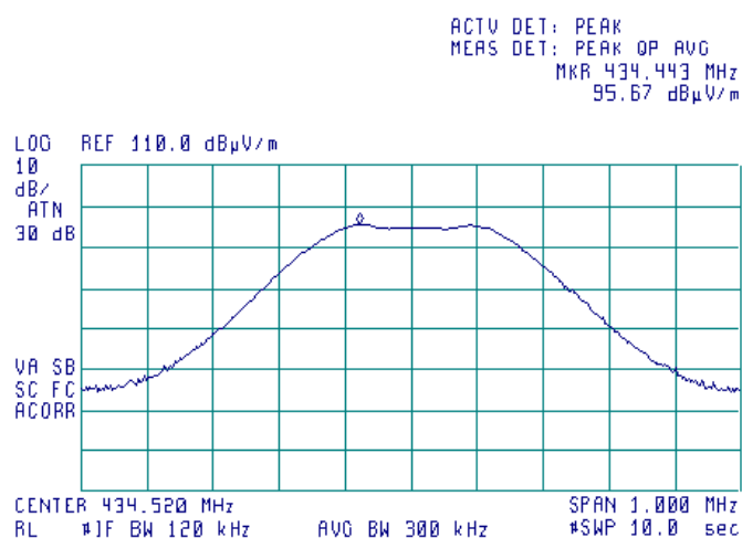
Plot 7.2.10 Radiated emission measurements at the fundamental frequency 434.52 MHz
