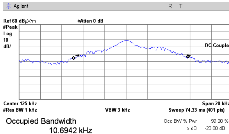
Plot 7.4.1 Occupied bandwidth test result
