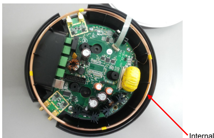
Photograph 7.6.1 Antenna view
