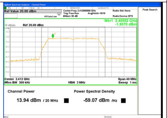
Test Mode: 802.11g---Low
