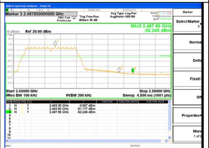
Test Mode: 802.11g---High
