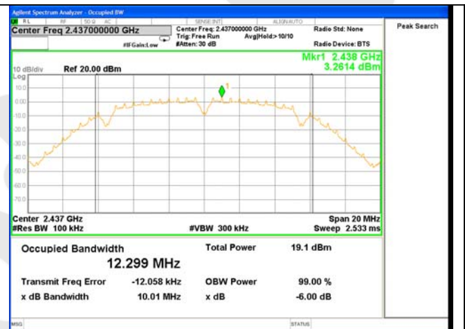
Test Mode: 802.11b---Mid
