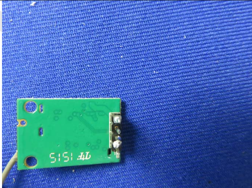
8. Figure PCB of the RF board-Back View
