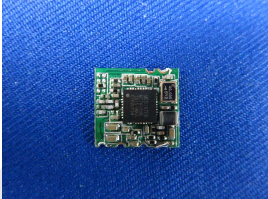
9. Figure PCB of the RF board-Front View
