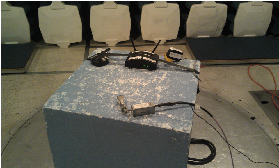
Radiated Emissions Measurements – Above 18GHz
