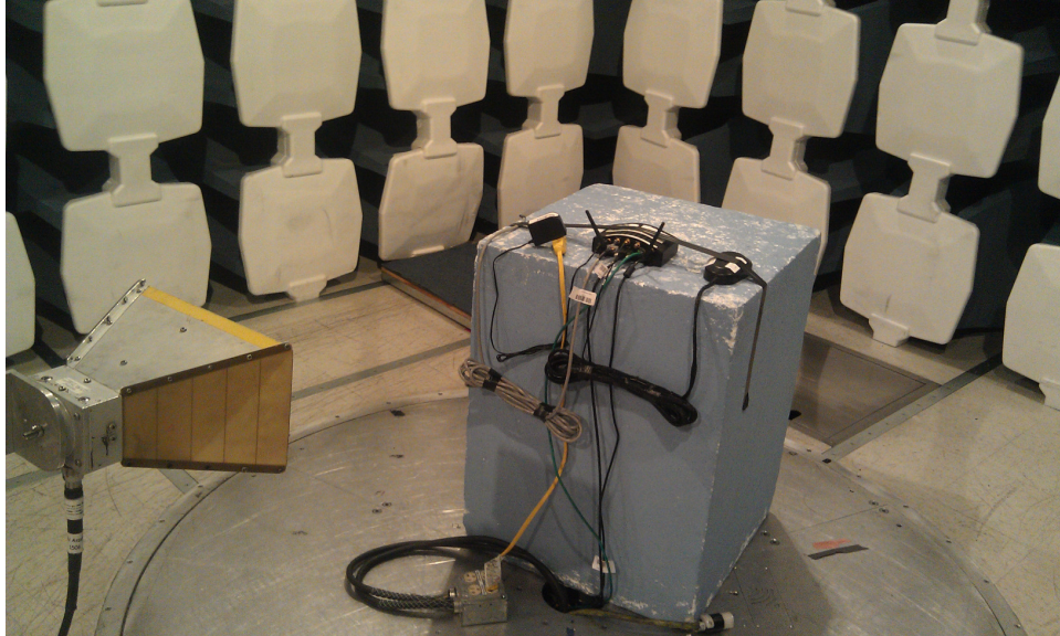
Radiated Emissions Measurements – Above 1GHz - Rear
