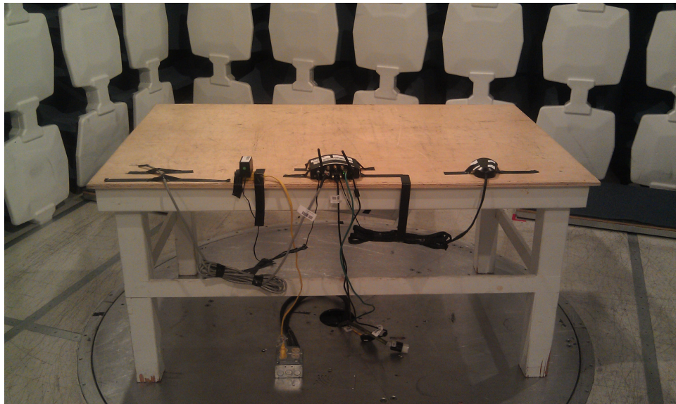
Radiated Emissions Measurements – Below 1GHz - Rear
