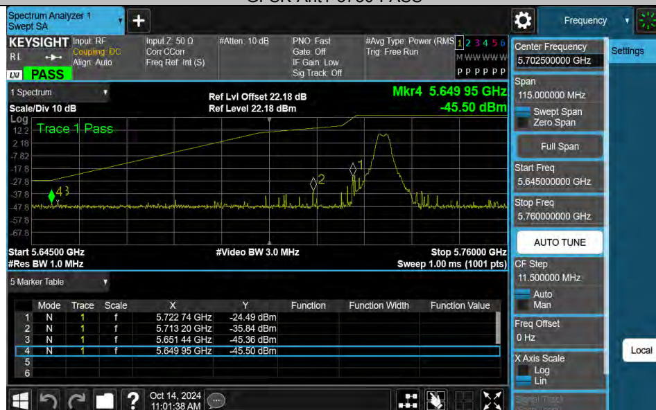
GFSK-Ant2-5730-PASS
