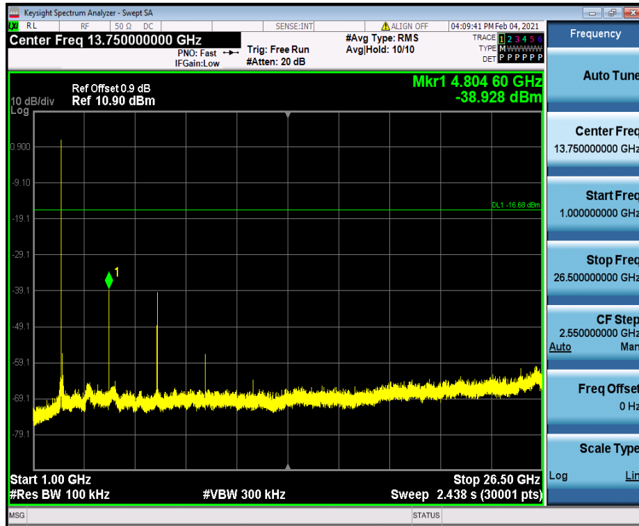
DH5_Ant1_2441_0~Reference
