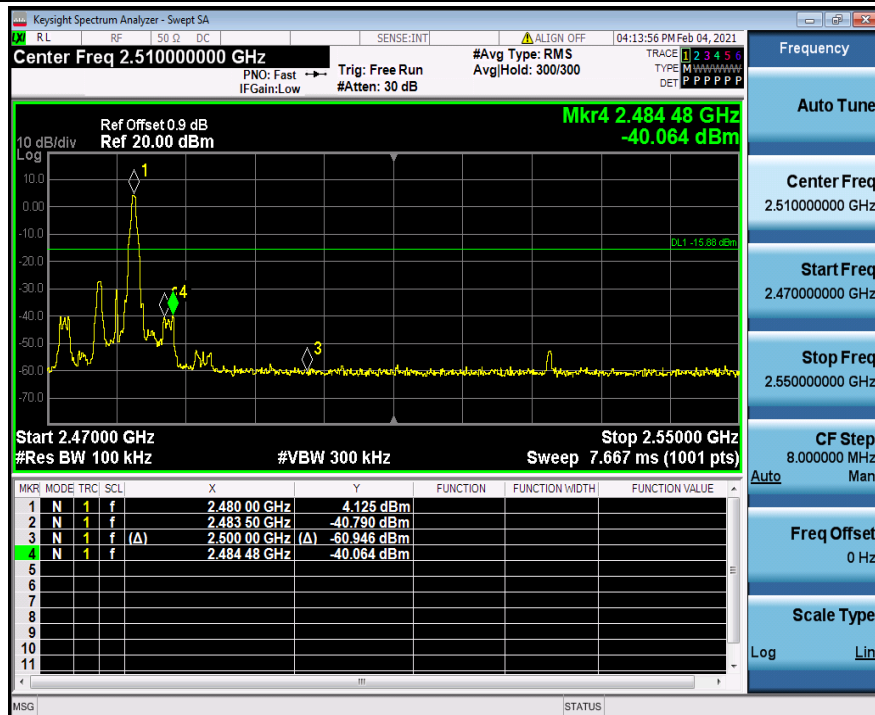
DH5_Ant1_High_2480
