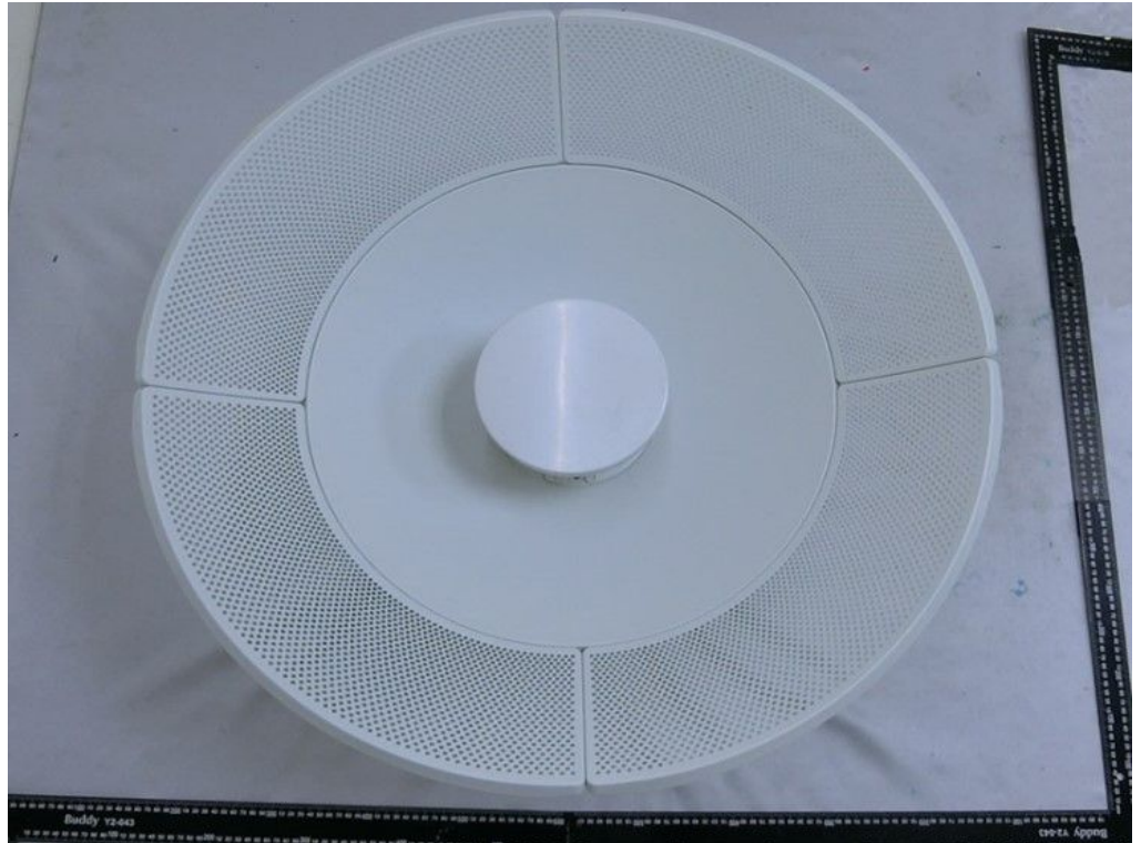
EUT with reflector antenna
