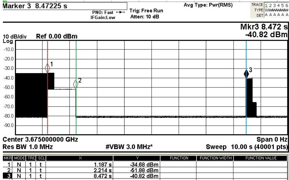
Figure 1-4: TX of at 3675 MHz for 15 MHz channel
