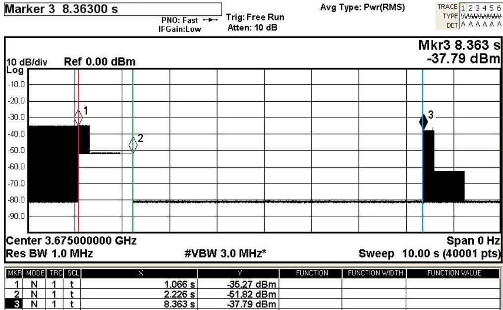
Red line – Interferer is on; Green line – Interferer is off; Blue line – TX is back on Figure 1-2: TX of at 3675 MHz for 7 MHz channel
