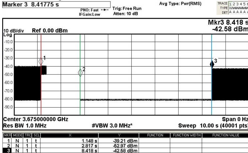
Figure 1-6: TX of at 3675 MHz for 30 MHz channel
