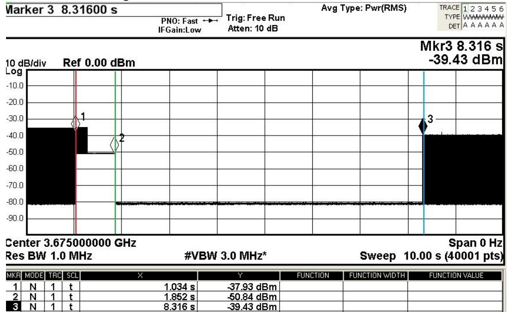
Red line – Interferer is on; Green line – Interferer is off; Blue line – TX is back on Figure 1-3: TX of at 3675 MHz for 10 MHz channel
