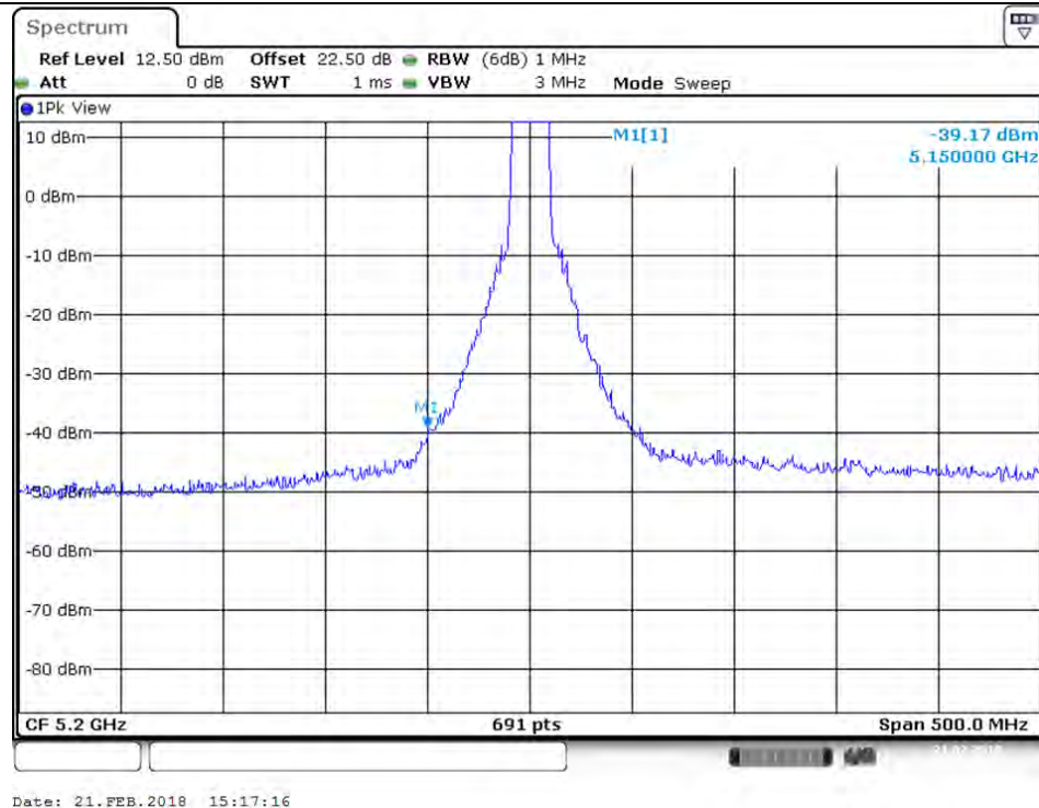
Plot on Configuration VHT20 / 5200 MHz / Peak / Port 2 (TX2)
