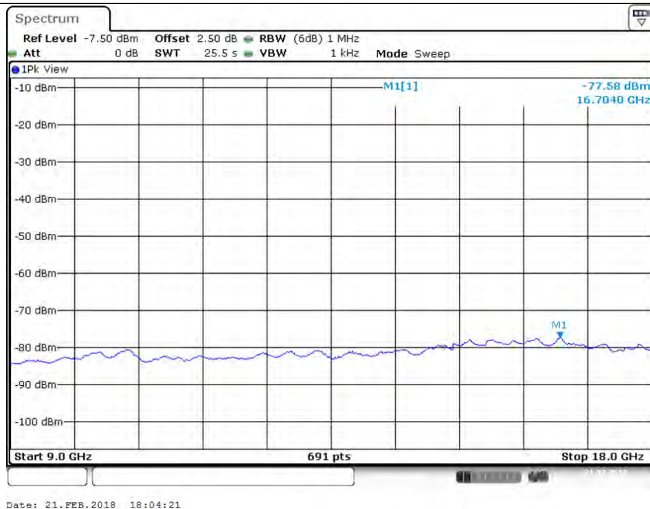
Plot on Configuration VHT20 / 5180 MHz / Average / Port 2 / 9GHz~18GHz
