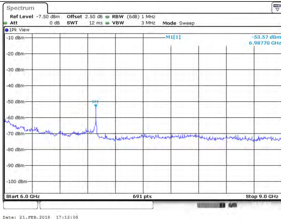
Plot on Configuration VHT20 / 5240 MHz / Peak / Port 2 / 6GHz~9GHz
