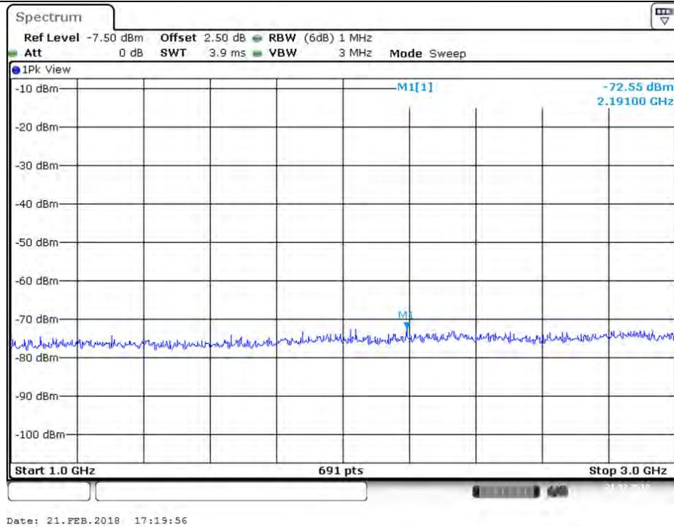
Plot on Configuration VHT20 / 5200 MHz / Peak / Port 2 / 1GHz~3GHz
