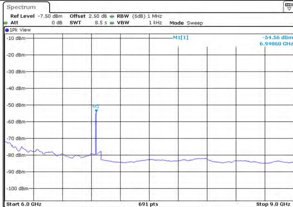
Plot on Configuration VHT80 / 5210 MHz / Average / Port 2 / 6GHz~9GHz
