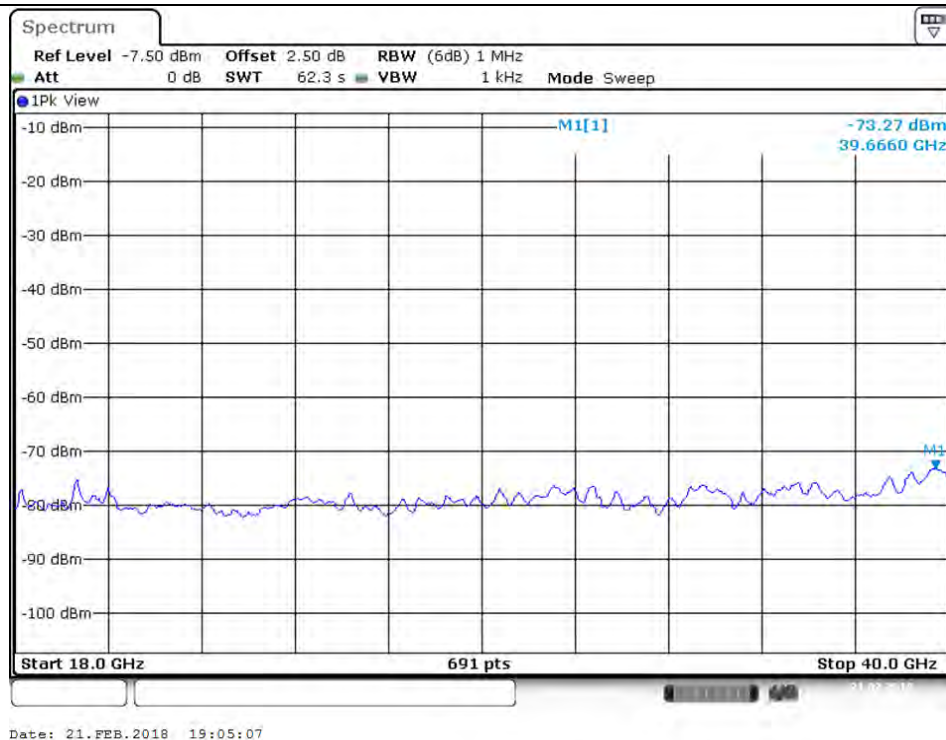
Plot on Configuration VHT20 / 5180 MHz / Average / Port 2 / 18GHz~40GHz
