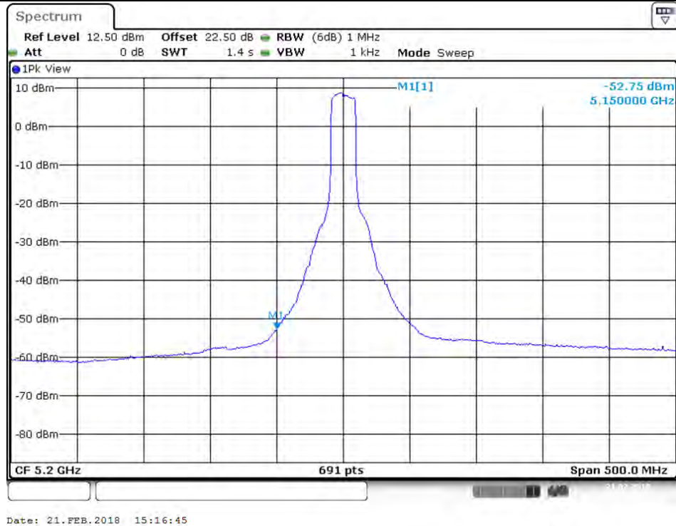
Plot on Configuration VHT20 / 5200 MHz / Average / Port 2 (TX2)
