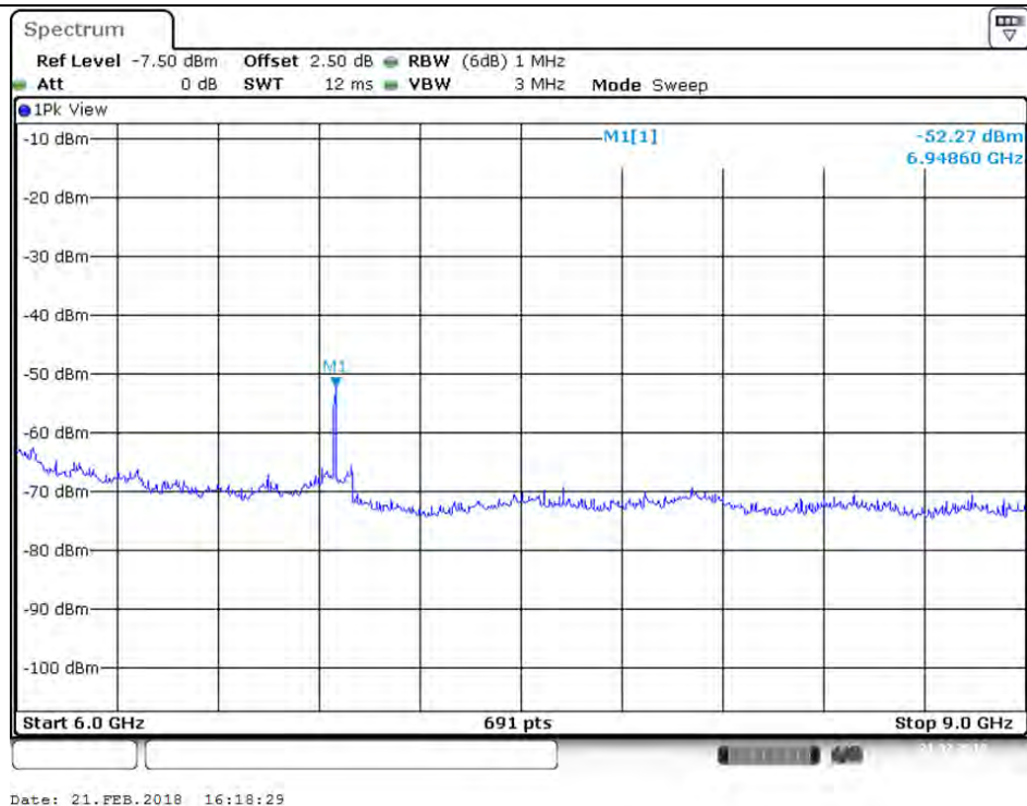
Plot on Configuration VHT80 / 5210 MHz / Peak / Port 2 / 6GHz~9GHz
