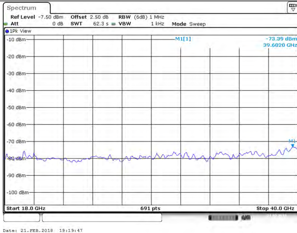
Plot on Configuration VHT80 / 5210 MHz / Average / Port 2 / 18GHz~40GHz
