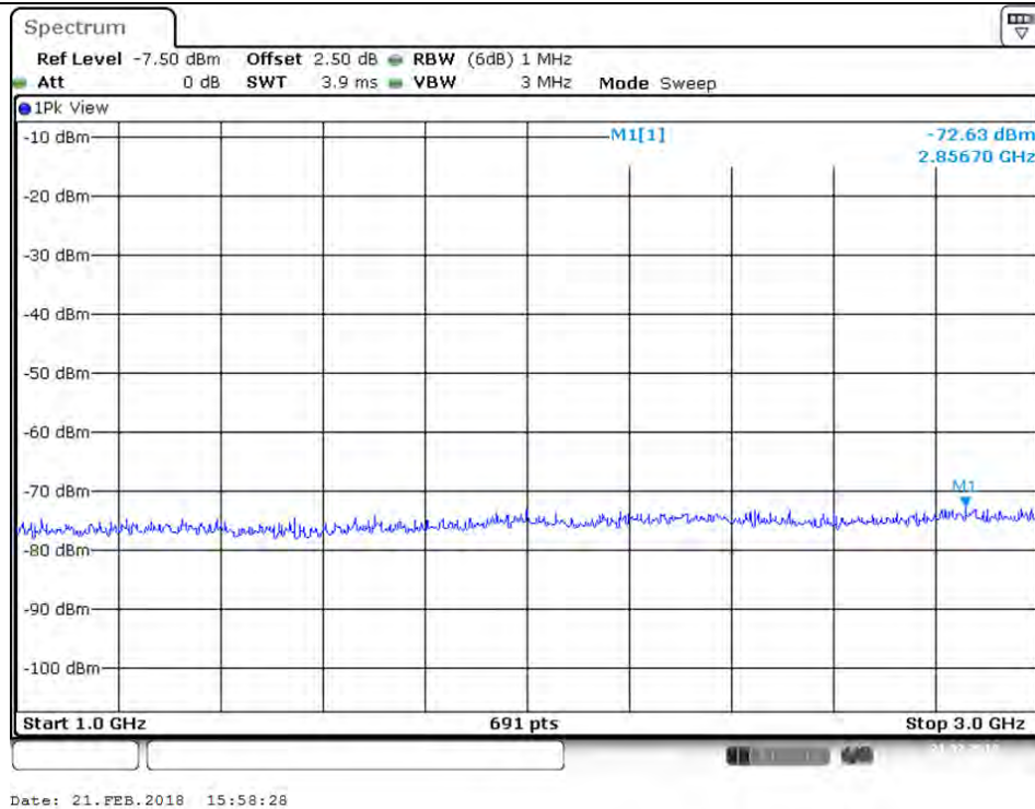
Plot on Configuration VHT80 / 5210 MHz / Peak / Port 2 / 1GHz~3GHz
