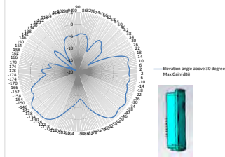
Elevation angle above 30 degree Max Gain(dBi)
