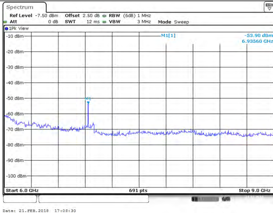
Plot on Configuration VHT20 / 5200 MHz / Peak / Port 2 / 6GHz~9GHz
