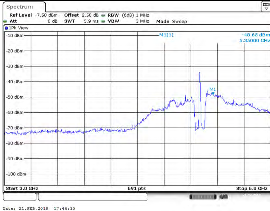
Plot on Configuration VHT20 / 5200 MHz / Peak / Port 2 / 3GHz~6GHz
