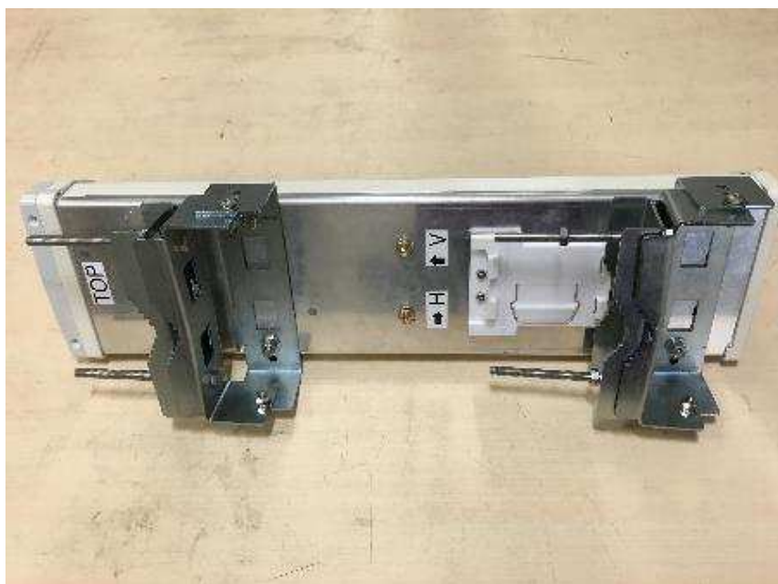
Figure 4: Photograph of 17 dBi Transmitter Antenna-Back view
