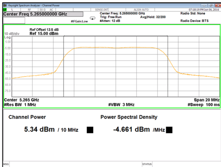
Figure 46: 10 MHz, 17 dBi, Low channel: Power spectral density measured at Ch. 1 – 5265 MHz
