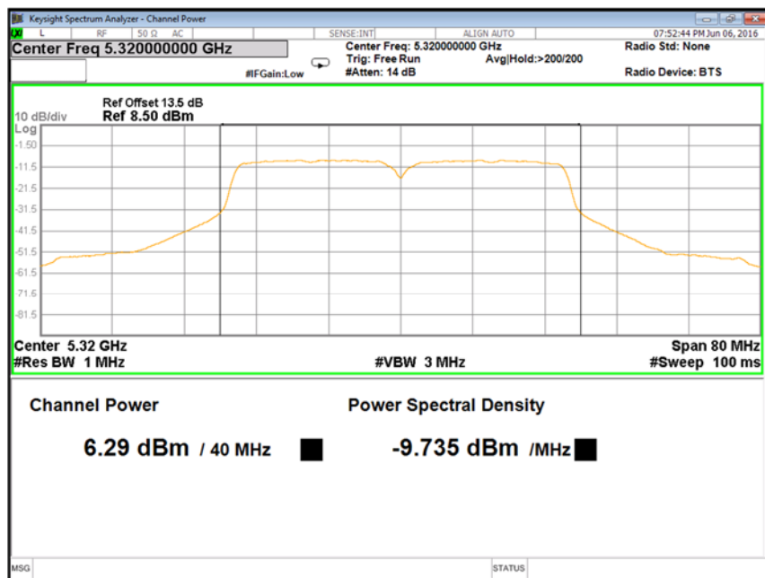
Figure 44: 40 MHz, 17 dBi, High channel: Power spectral density measured at Ch. 1 – 5320 MHz
