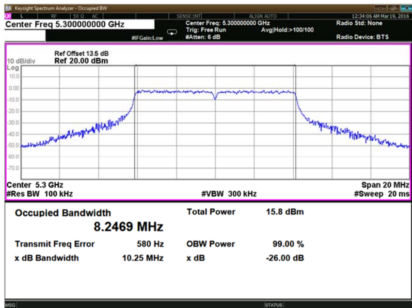
Figure 15: 10 MHz, 17 dB, Mid channel: 26 dB bandwidth measured at Ch.1 - 5300 MHz
