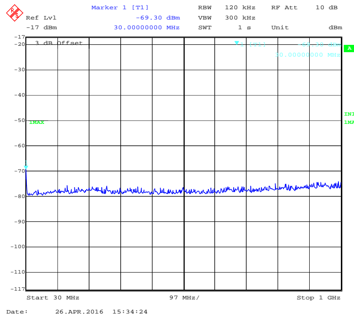
Figure 63: 40 MHz, 17 dBi, Low channel: Peak emission from 30 MHz to 1 GHz at Ch. 1 –5280 MHz
