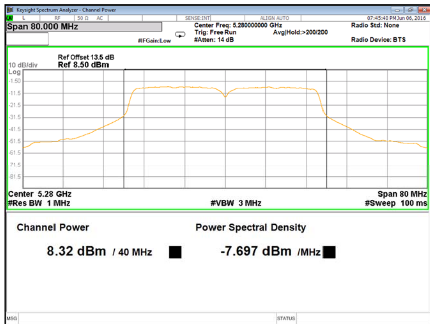
Figure 40: 40 MHz, 17 dBi, Low channel: Power spectral density measured at Ch. 1 – 5280 MHz
