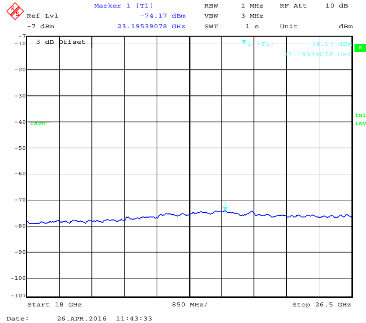
Figure 74: 40 MHz, 17 dBi, Mid channel: Average emission from 18 GHz to 26.5 GHz at Ch. 0 -5300 MHz
