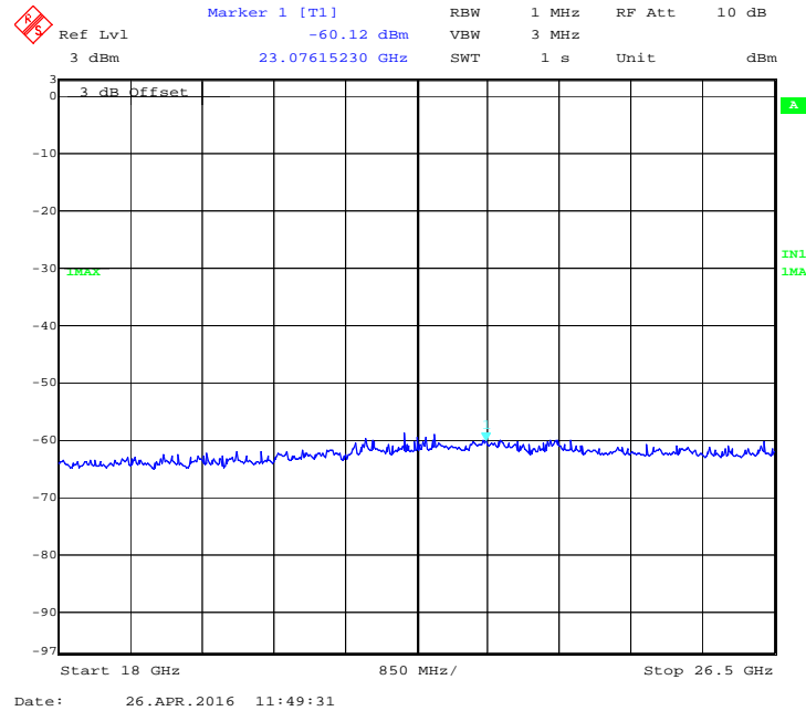
Figure 68: 40 MHz, 17 dBi, Low channel: Peak emission from 18 GHz to 26.5 GHz at Ch. 1 -5280 MHz
