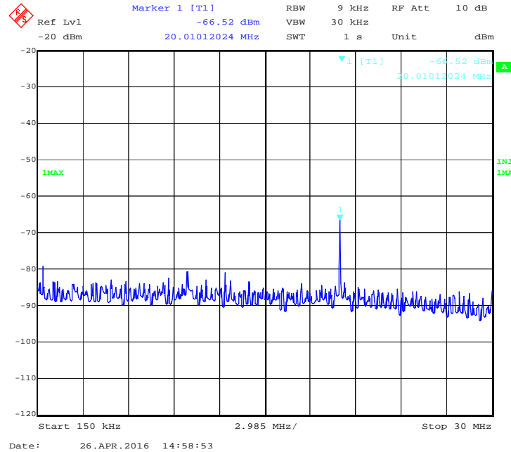
Figure 62: 40 MHz, 17 dBi, Low channel: Peak emission from 150 kHz to 30 MHz at Ch. 1 –5280 MHz
