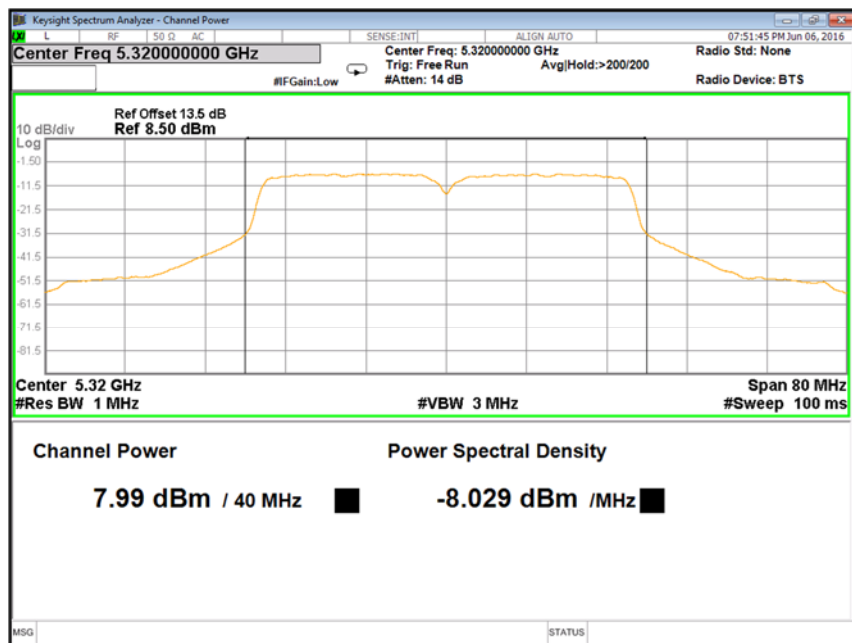
Figure 43: 40 MHz, 17 dBi, High channel: Power spectral density measured at Ch. 0 – 5320 MHz
