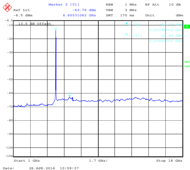
Figure 55: 40 MHz, 17 dBi, Low channel: Average emission from 1 GHz to 18 GHz at Ch. 0 -5280 MHz
