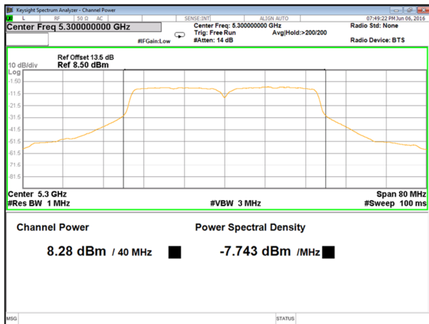
Figure 41: 40 MHz, 17 dBi, Mid channel: Power spectral density measured at Ch. 0 – 5300 MHz
