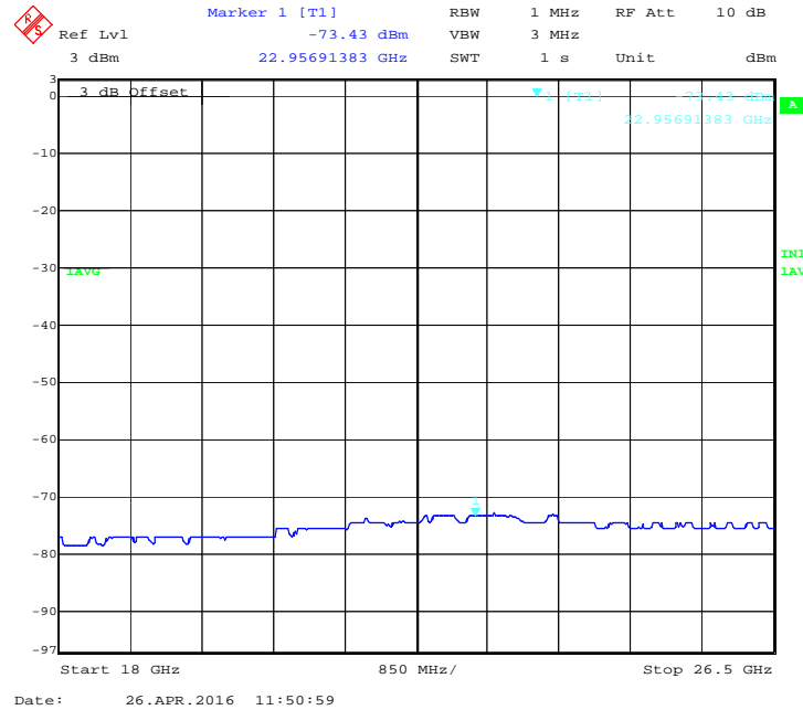
Figure 56: 40 MHz, 17 dBi, Low channel: Average emission from 18 GHz to 26.5 GHz at Ch. 0 –5280 MHz
