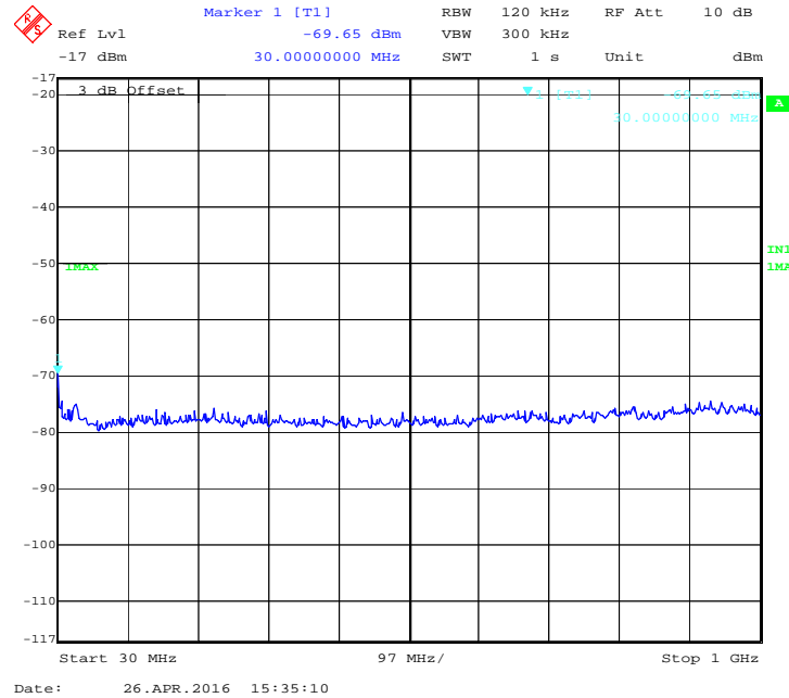
Figure 72: 40 MHz, 17 dBi, Mid channel: Peak emission from 30 MHz to 1 GHz at Ch. 0 -5300 MHz
