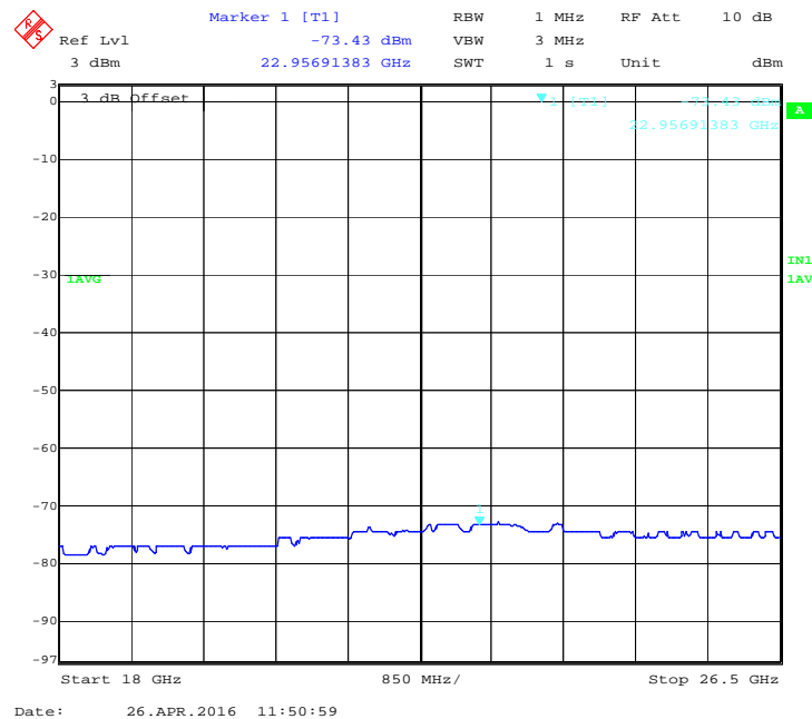
Figure 65: 40 MHz, 17 dBi, Low channel: Average emission from 18 GHz to 26.5 GHz at Ch. 1 -5280 MHz
