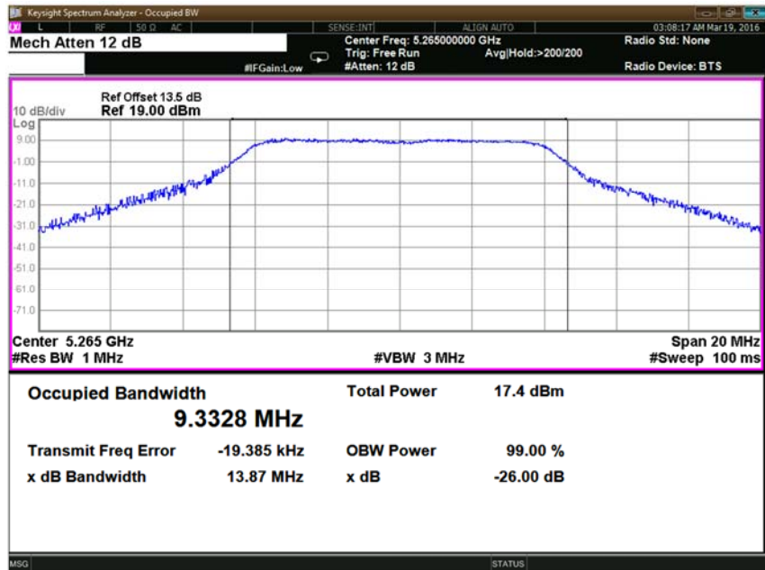
Figure 25: 10 MHz, 17 dB, Low channel: 99% OBW measured at Ch.0 – 5265 MHz
