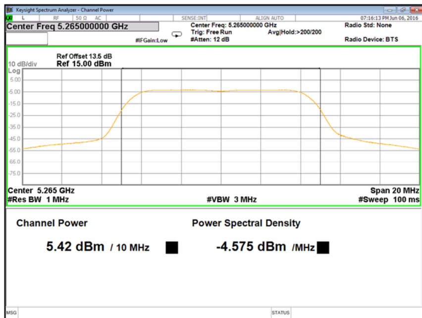
Figure 45: 10 MHz, 17 dBi, Low channel: Power spectral density measured at Ch. 0 – 5265 MHz
