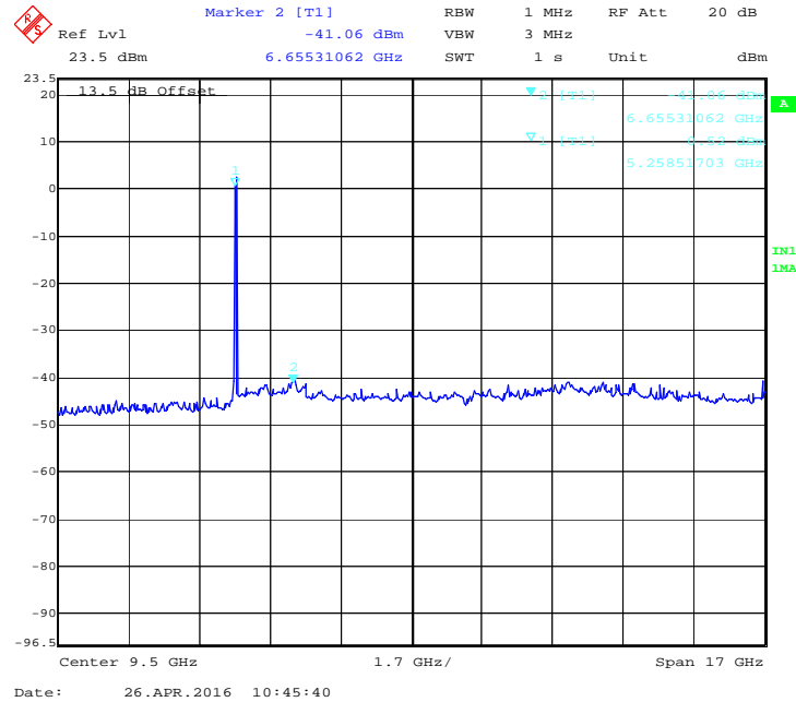
Figure 58: 40 MHz, 17 dBi, Low channel: Peak emission from 1 GHz to 18 GHz at Ch. 0 -5280 MHz
