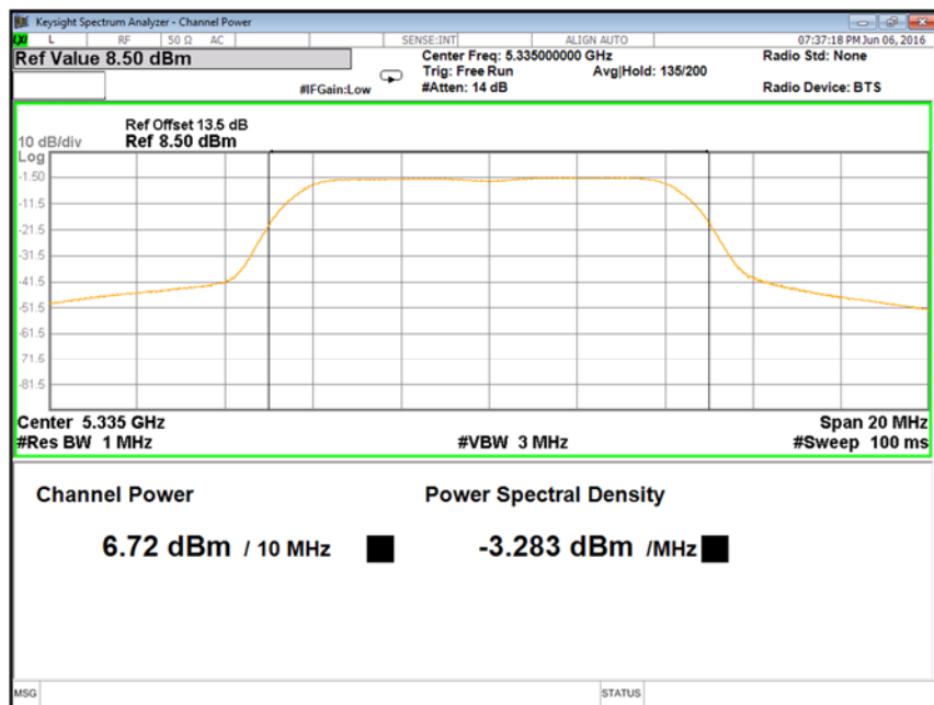
Figure 49: 10 MHz, 17 dBi, High channel: Power spectral density measured at Ch. 0 – 5335 MHz
