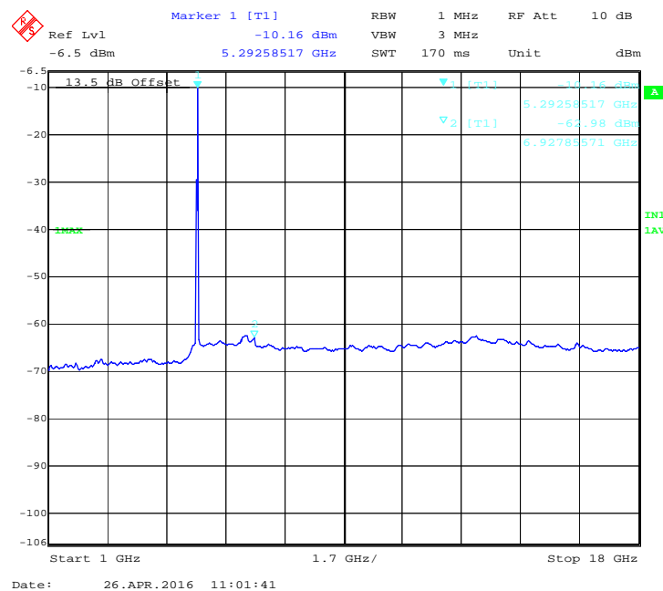
Figure 73: 40 MHz, 17 dBi, Mid channel: Average emission from 1 GHz to 18 GHz at Ch. 0 -5300 MHz
