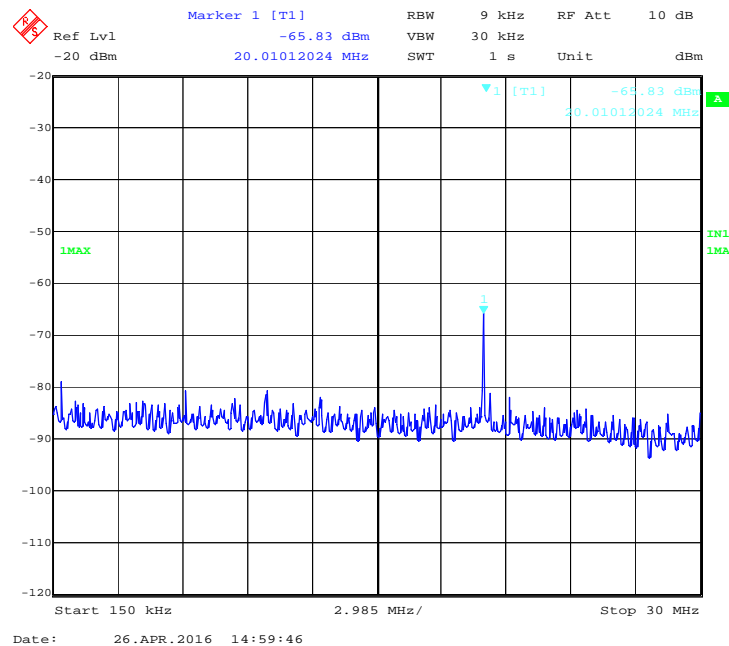
Figure 71: 40 MHz, 17 dBi, Mid channel: Peak emission from 150 kHz to 30 MHz at Ch. 0 –5300 MHz
