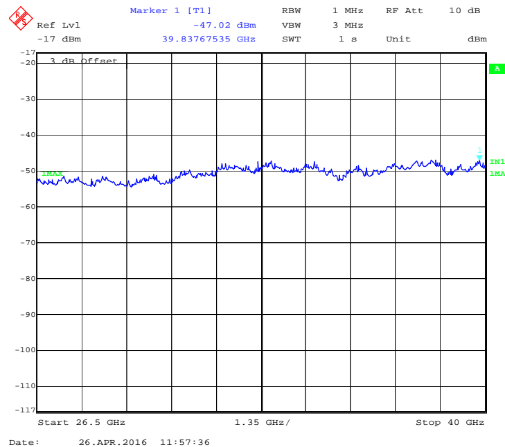
Figure 69: 40 MHz, 17 dBi, Low channel: Peak emission from 26.5 GHz to 40 GHz at Ch. 1 -5280 MHz
