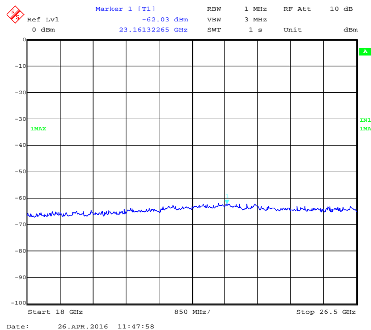
Figure 59: 40 MHz, 17 dBi, Low channel: Peak emission from 18 GHz to 26.5 GHz at Ch. 0 -5280 MHz
