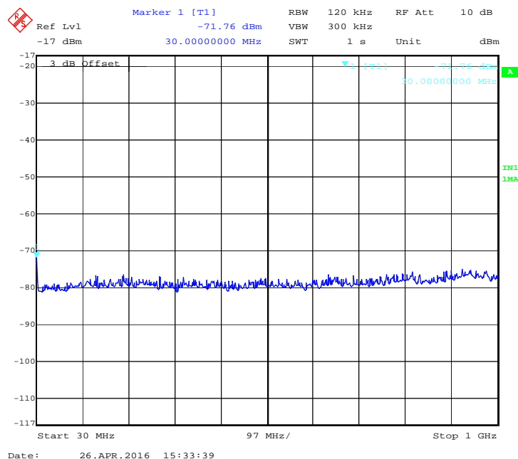
Figure 54: 40 MHz, 17 dBi, Low channel: Peak emission from 30 MHz to 1 GHz at Ch. 0 -5280 MHz
