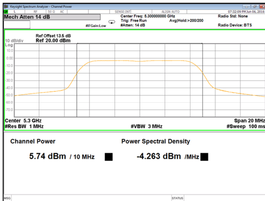
Figure 48: 10 MHz, 17 dBi, Mid channel: Power spectral density measured at Ch. 1 – 5300 MHz
