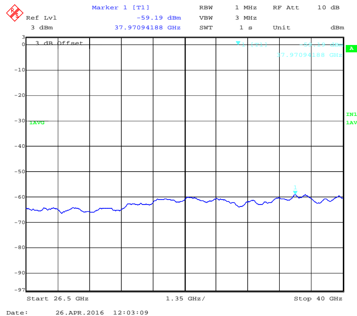
Figure 75: 40 MHz, 17 dBi, Mid channel: Average emission from 26.5 GHz to 40 GHz at Ch. 0 -5300 MHz
