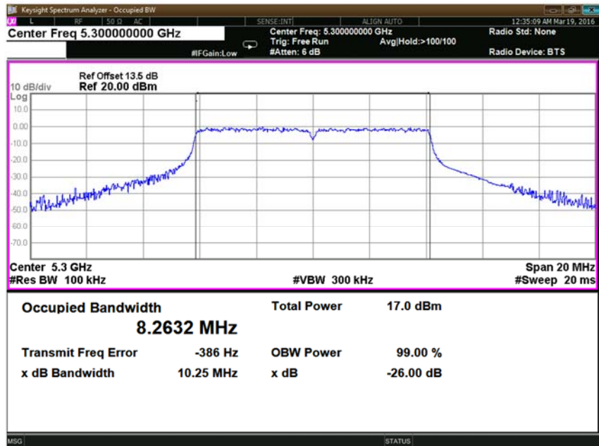
Figure 14: 10 MHz, 17 dB, Mid channel: 26 dB bandwidth measured at Ch.0 - 5300 MHz
