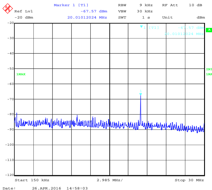
Figure 53: 40 MHz, 17 dBi, Low channel: Peak emission from 150 kHz to 30 MHz at Ch. 0 – 5280 MHz
