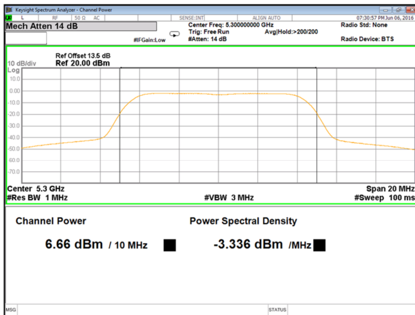
Figure 47: 10 MHz, 17 dBi, Mid channel: Power spectral density measured at Ch. 0– 5300 MHz
