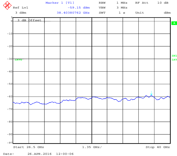
Figure 66: 40 MHz, 17 dBi, Low channel: Average emission from 26.5 GHz to 40 GHz at Ch. 1 –5280 MHz
