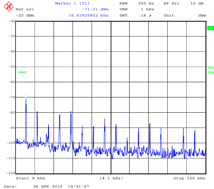
Figure 70: 40 MHz, 17 dBi, Mid channel: Peak emission from 9 kHz to 150 kHz at Ch. 0 –5300 MHz
