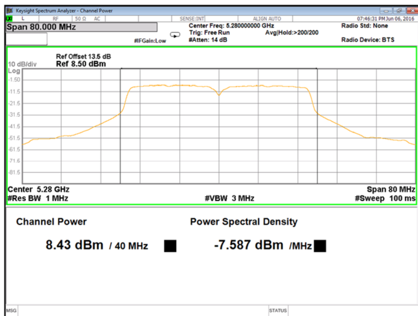
Figure 39: 40 MHz, 17 dBi, Low channel: Power spectral density measured at Ch. 0 – 5280 MHz
