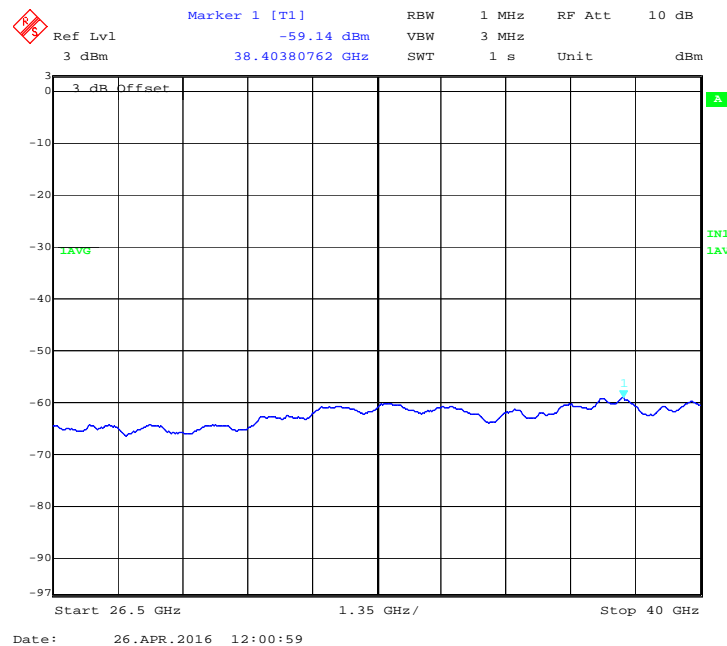
Figure 57: 40 MHz, 17 dBi, Low channel: Average emission from 26.5 GHz to 40 GHz at Ch. 0 –5280 MHz
