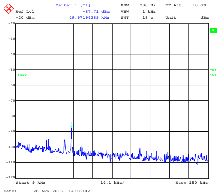
Figure 52: 40 MHz, 17 dBi, Low channel: Peak emission from 9 kHz to 150 kHz at Ch. 0 – 5280 MHz
