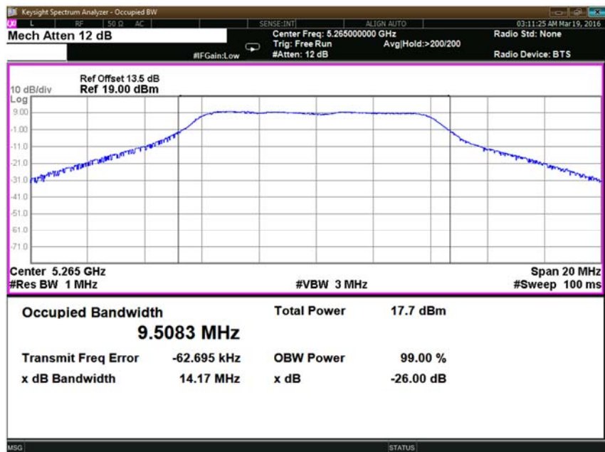
Figure 26: 10 MHz, 17 dB, Low channel: 99% OBW measured at Ch.1 – 5265 MHz
