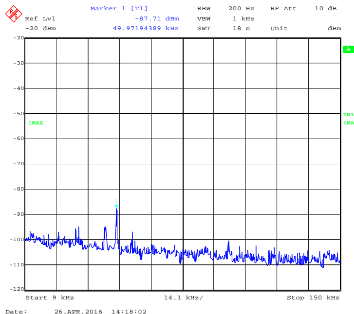
Figure 61: 40 MHz, 17 dBi, Low channel: Peak emission from 9 kHz to 150 kHz at Ch. 1 -5280 MHz
