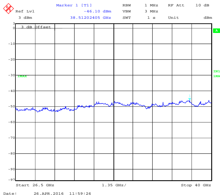
Figure 60: 40 MHz, 17 dBi, Low channel: Peak emission from 26.5 GHz to 40 GHz at Ch. 0 -5280 MHz
