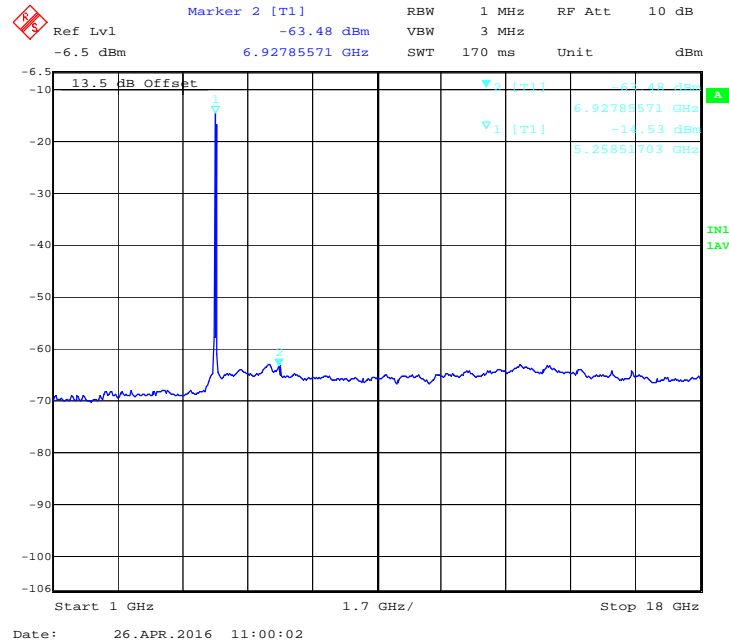
Figure 64: 40 MHz, 17 dBi, Low channel: Average emission from 1 GHz to 18 GHz at Ch. 1 -5280 MHz
