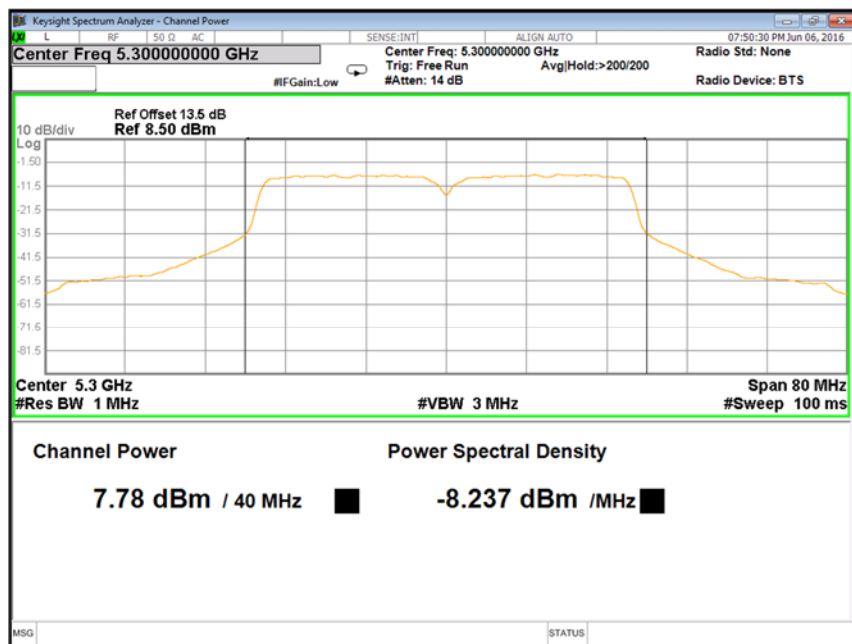
Figure 42: 40 MHz, 17 dBi, Mid channel: Power spectral density measured at Ch. 1 – 5300 MHz
