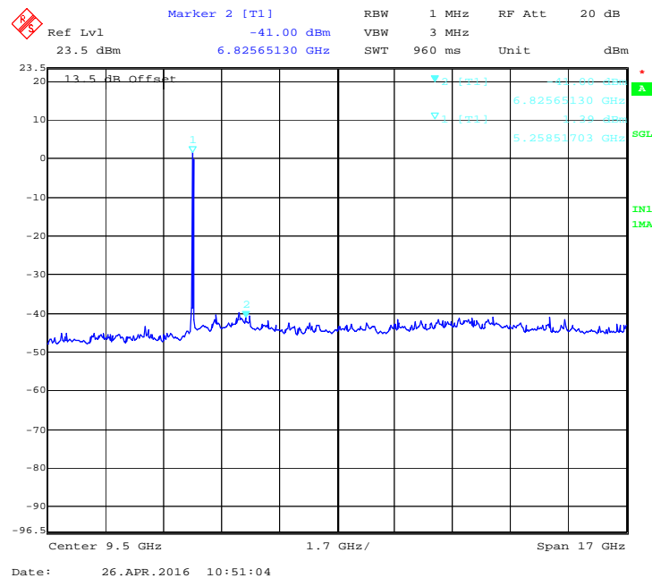
Figure 67: 40 MHz, 17 dBi, Low channel: Peak emission from 1 GHz to 18 GHz at Ch. 1 –5280 MHz
