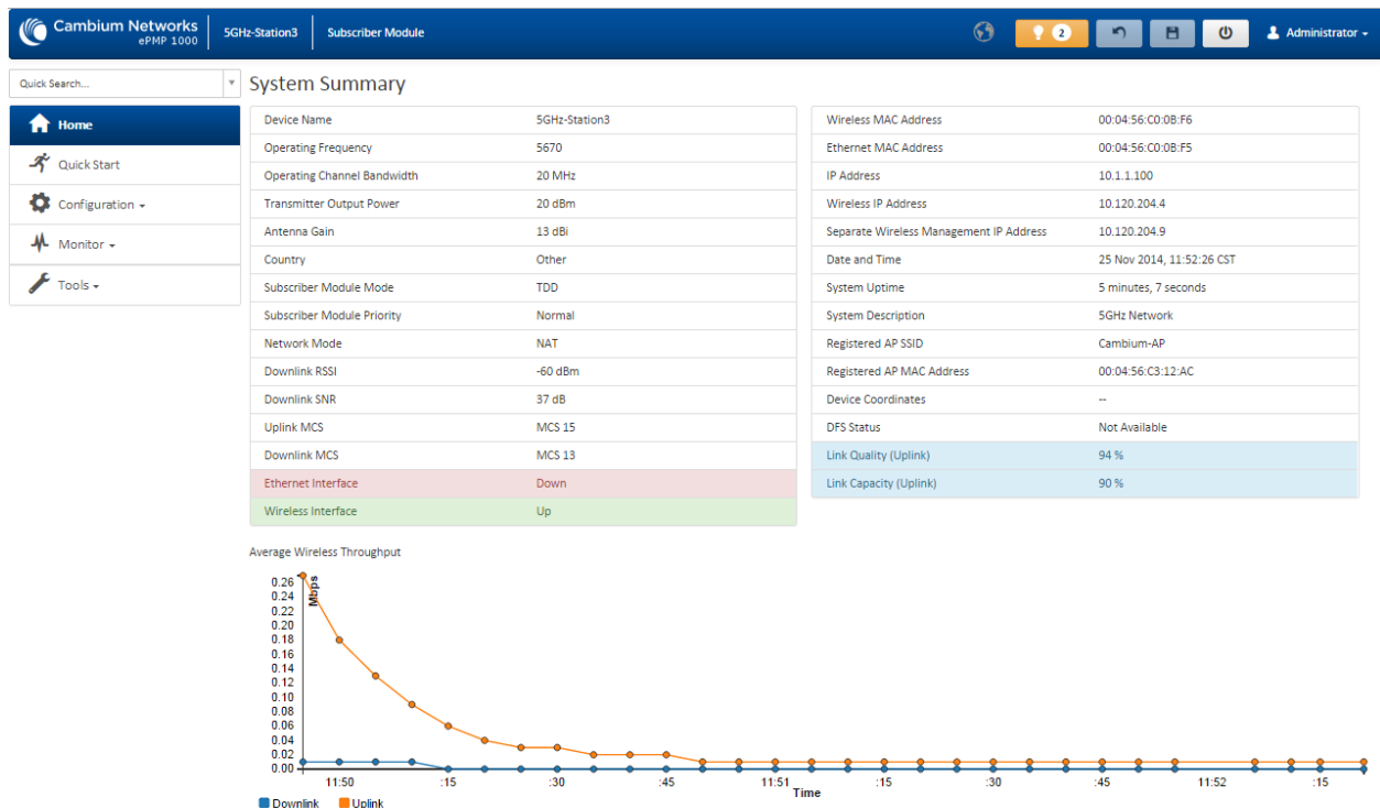
Figure 14 SM Dashboard
