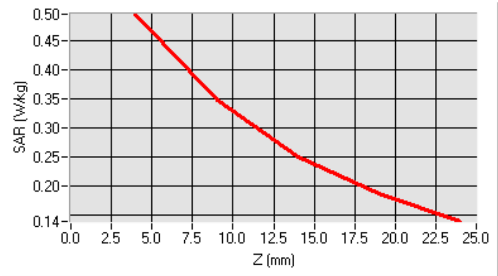
SAR, Z Axis Scan (X = -30, Y = -16)
