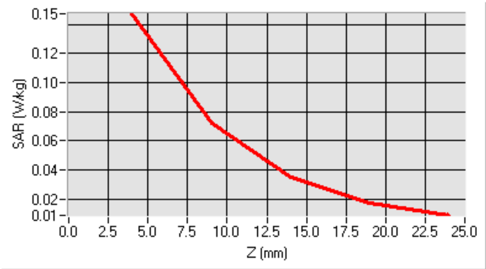
SAR, Z Axis Scan (X = -57, Y = -55)
