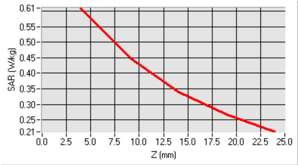
SAR, Z Axis Scan (X = -42, Y = -26)
