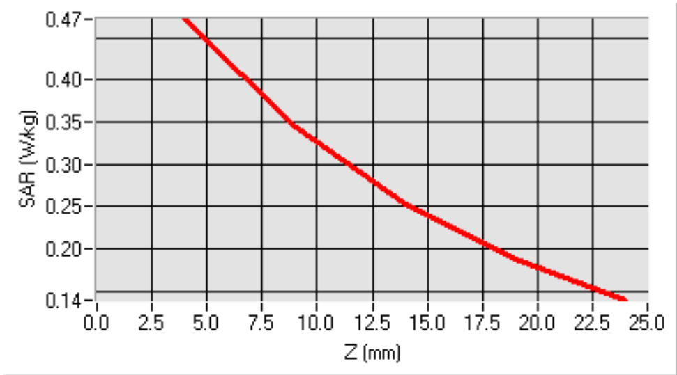
SAR, Z Axis Scan (X = 0, Y = -48)
