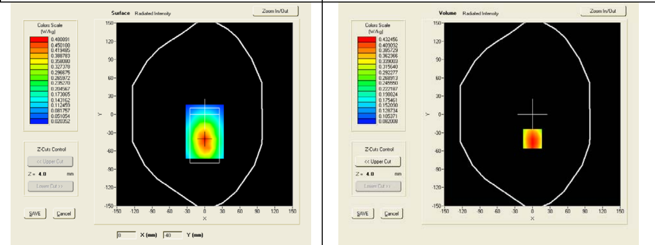
SAR, Z Axis Scan (X = 0, Y = -40)
