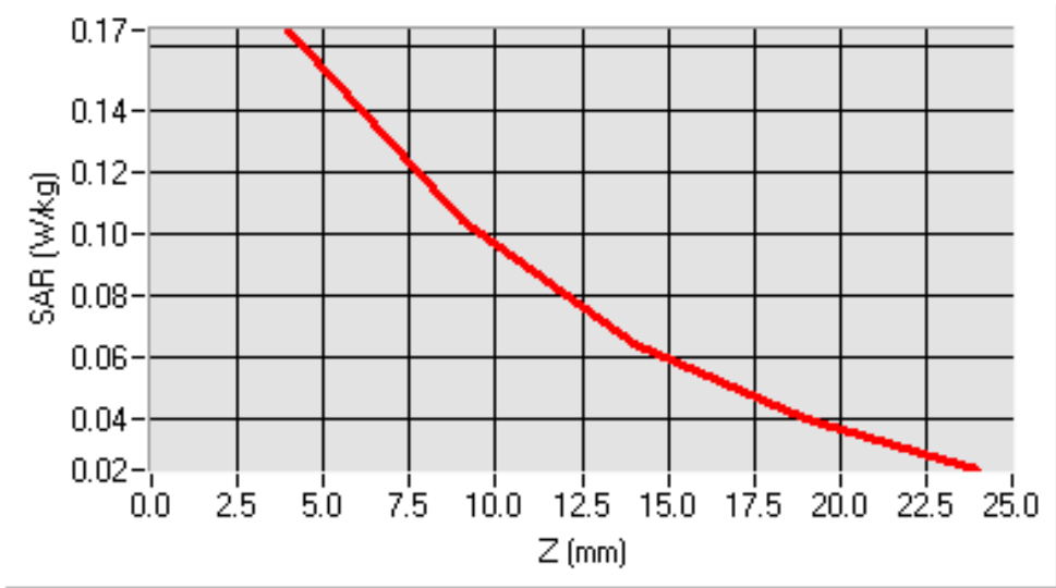
SAR, Z Axis Scan (X = 2, Y = -62)
