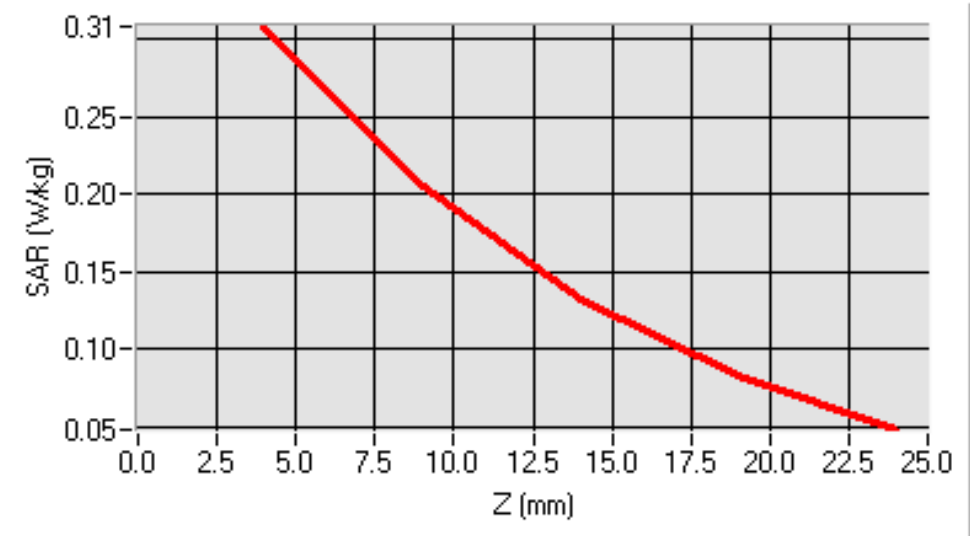
SAR, Z Axis Scan (X = -53, Y = -46)
