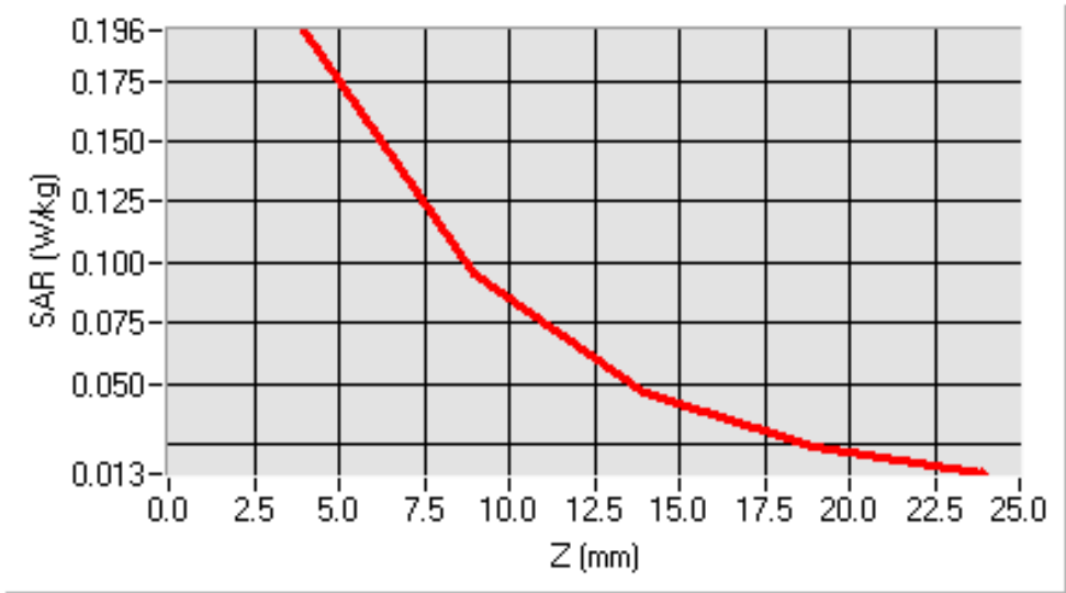
SAR, Z Axis Scan (X = -55, Y = -47)
