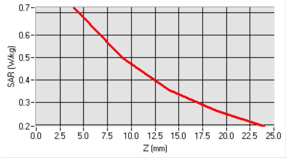
SAR, Z Axis Scan (X = -39, Y = -24)
