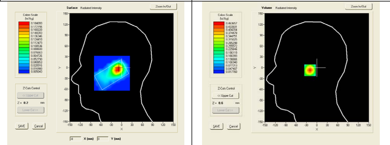
SAR, Z Axis Scan (X = -10, Y = -5)
