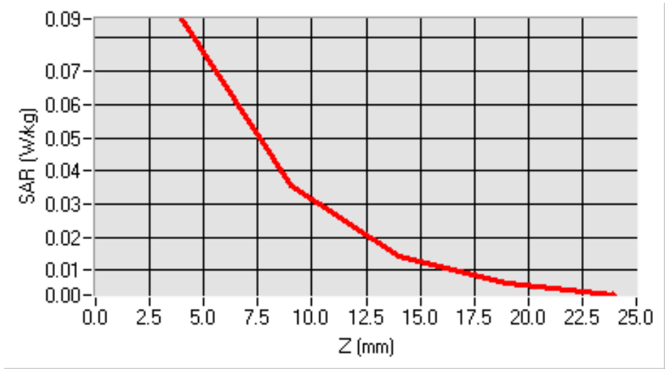
SAR, Z Axis Scan (X = -3, Y = -32)
