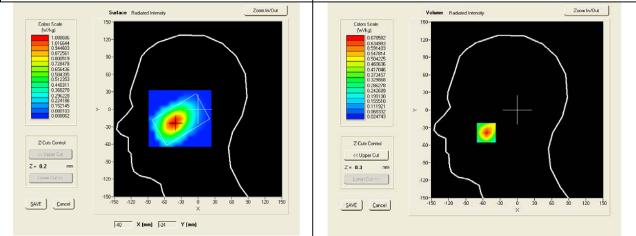
SAR, Z Axis Scan (X = -43, Y = -24)
