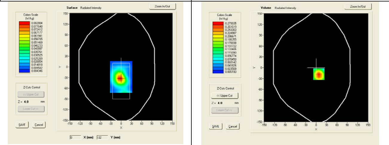
SAR, Z Axis Scan (X = -3, Y = -32)
