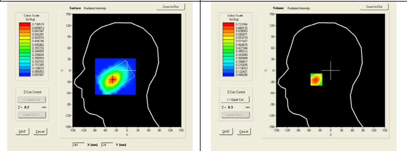
SAR, Z Axis Scan (X = -39, Y = -24)
