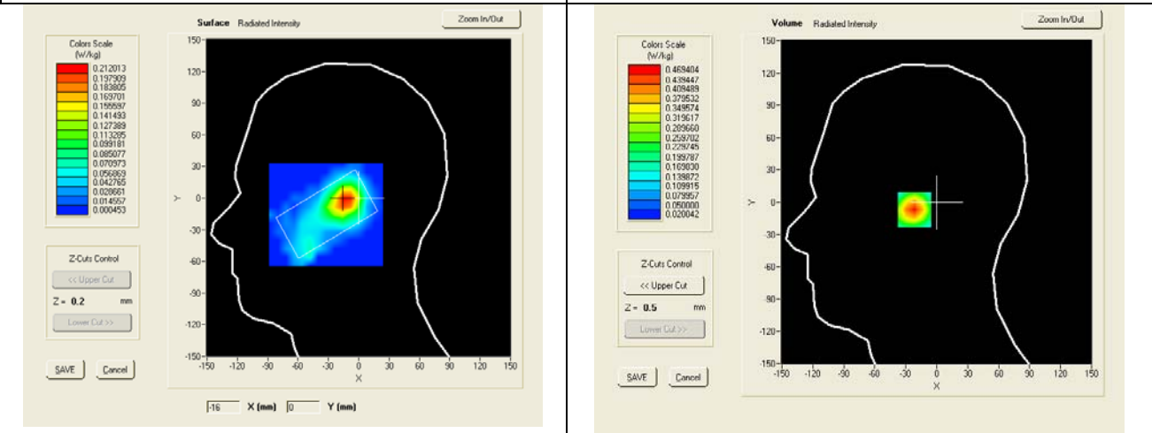
SAR, Z Axis Scan (X = -14, Y = -1)
