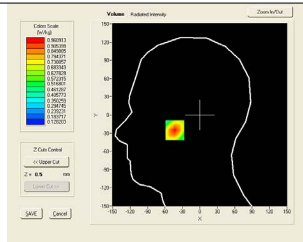
SAR, Z Axis Scan (X = -43, Y = -25)
