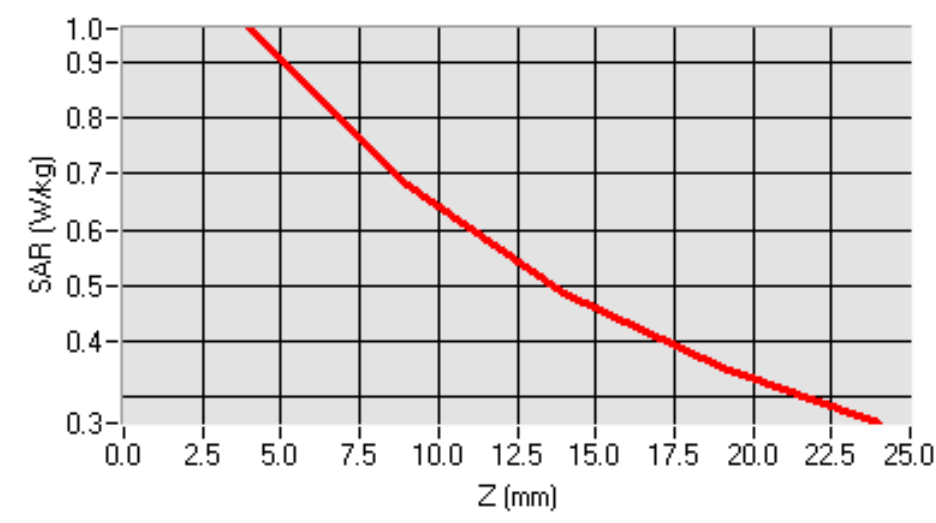
SAR, Z Axis Scan (X = -43, Y = -25)
