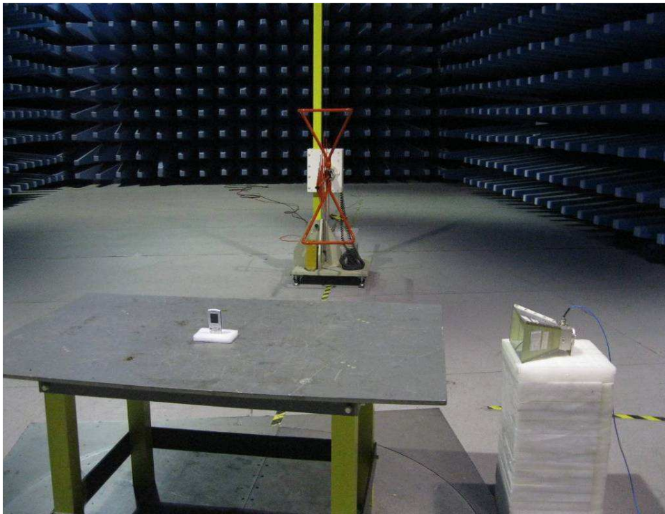
Below 1GHz: Radiated Emissions - Front View
