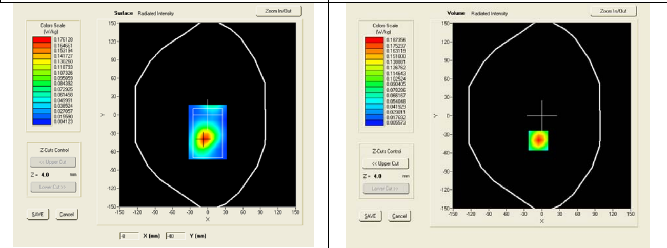
SAR, Z Axis Scan (X = -6, Y = -40)
