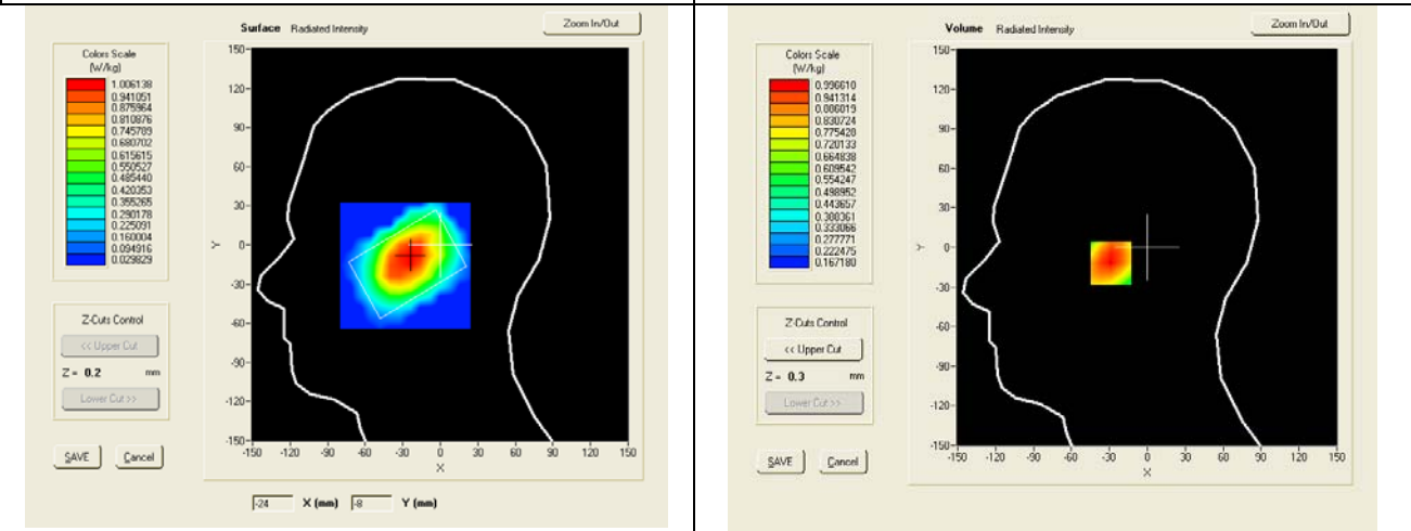
SAR, Z Axis Scan (X = -25, Y = -12)
