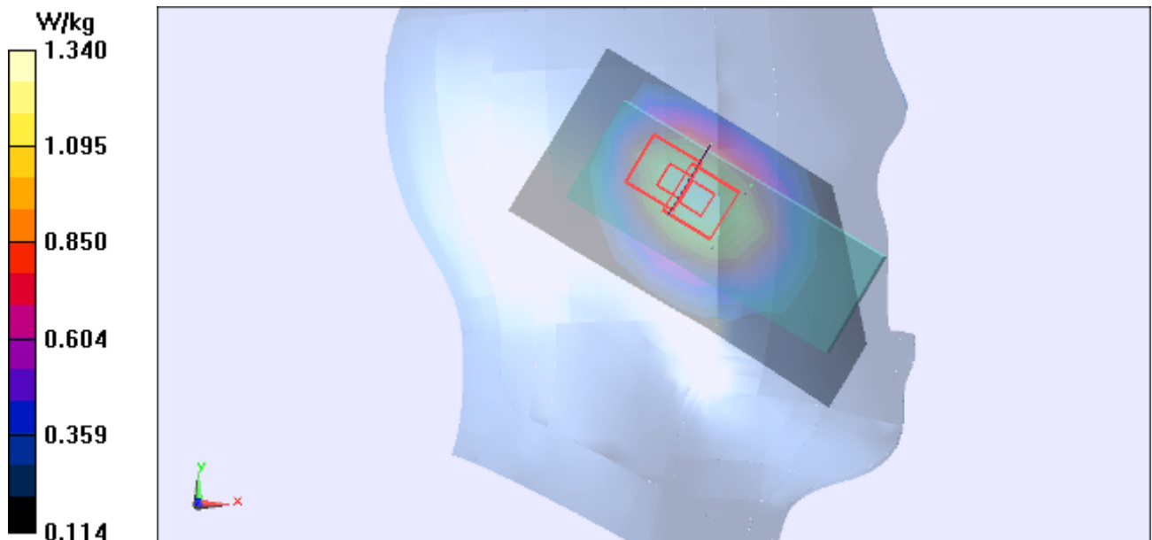
Figure 11 Left Hand Touch Cheek GSM 850 Channel 251
