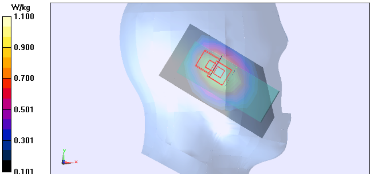
Figure 13 Left Hand Touch Cheek GSM 850 Channel 128
