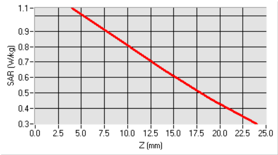
SAR, Z Axis Scan (X = -2, Y = -9)
