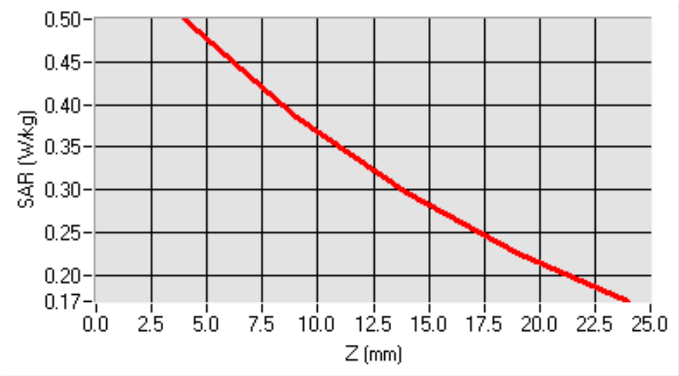
SAR, Z Axis Scan (X = -23, Y = -16)
