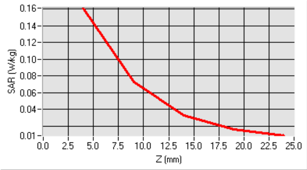
SAR, Z Axis Scan (X = -1, Y = 2)
