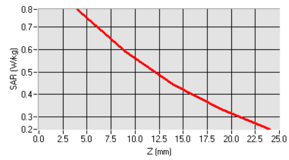
SAR, Z Axis Scan (X = -21, Y = -15)
