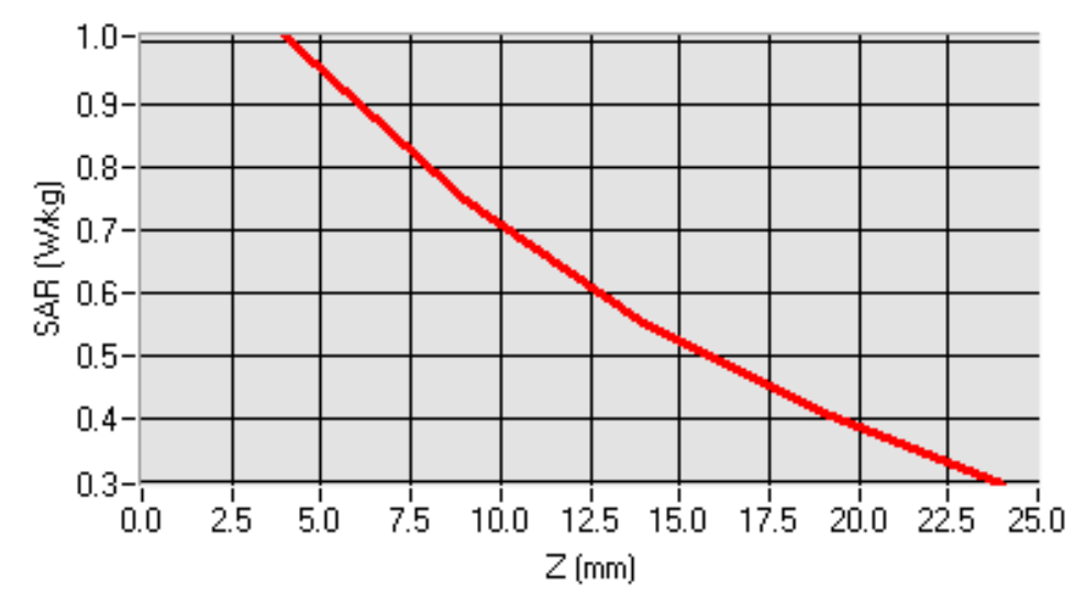
SAR, Z Axis Scan (X = -24, Y = -16)
