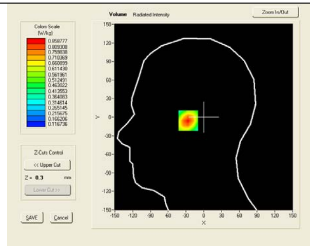
SAR, Z Axis Scan (X = -23, Y = -6)
