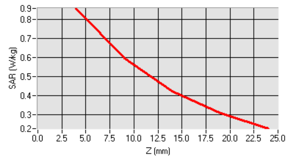
SAR, Z Axis Scan (X = -23, Y = -6)
