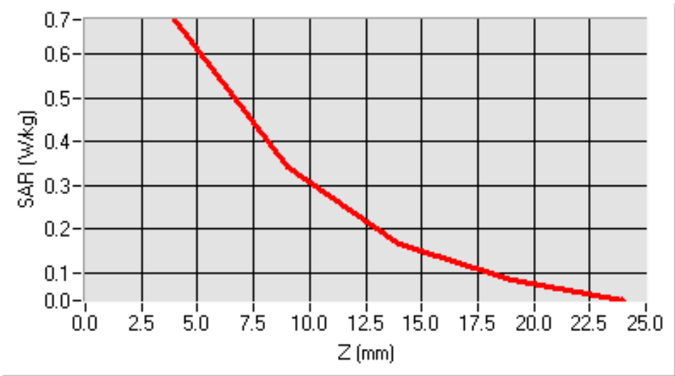
SAR, Z Axis Scan (X = -14, Y = 5)
