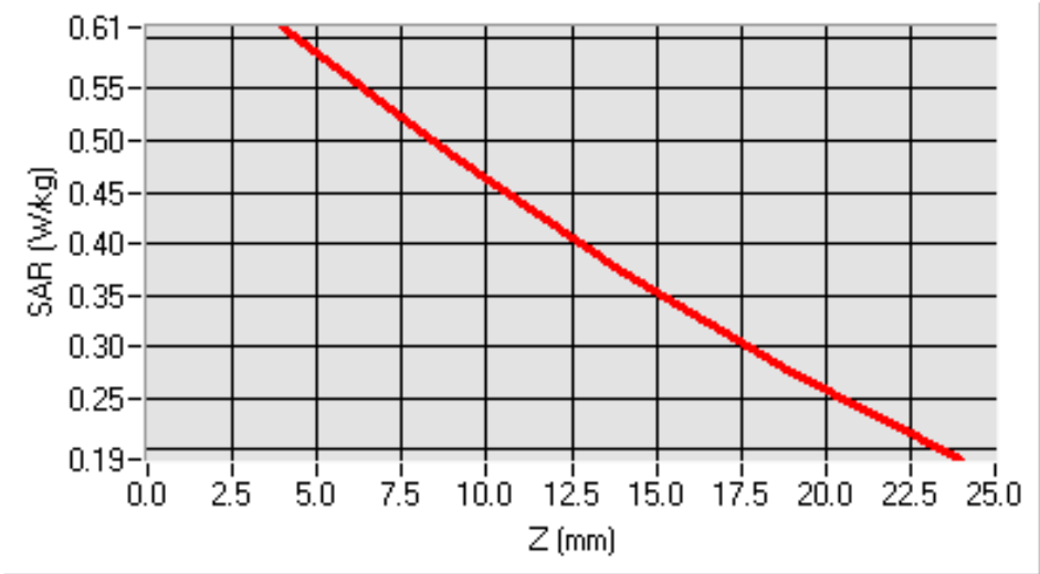
SAR, Z Axis Scan (X = 0, Y = -15)
