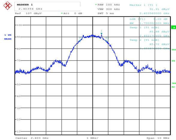
Plot 8.2-2: 6 dB bandwidth – Mid channel, Ant 1
