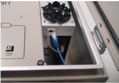
Figure 3-6 Power cable connection (PoE type)
