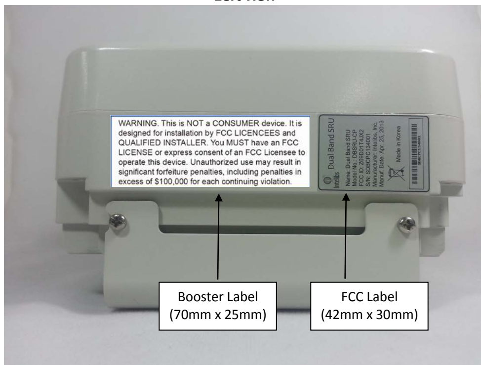
Left view
