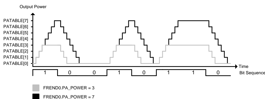
Figure 32: Shaping of ASK Signal
