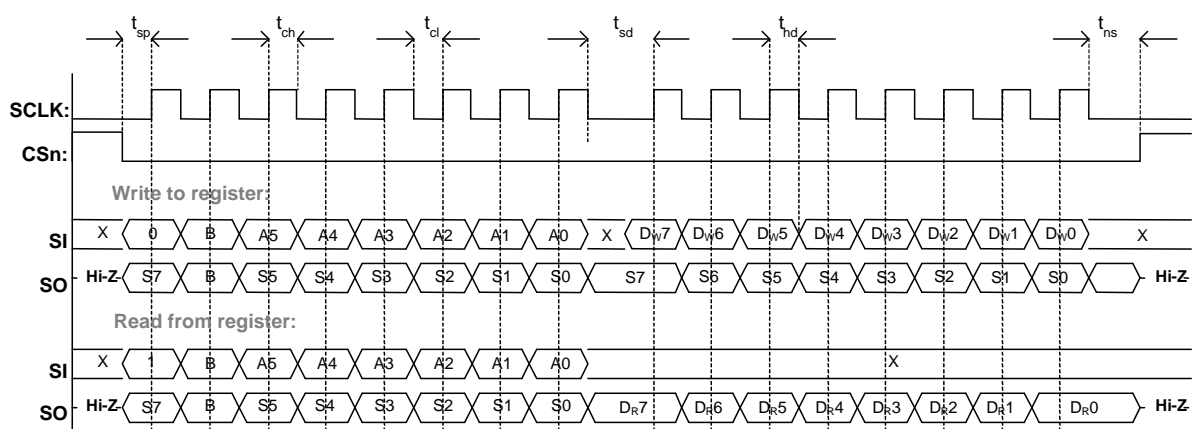
Figure 15: Configuration Registers Write and Read Operations
