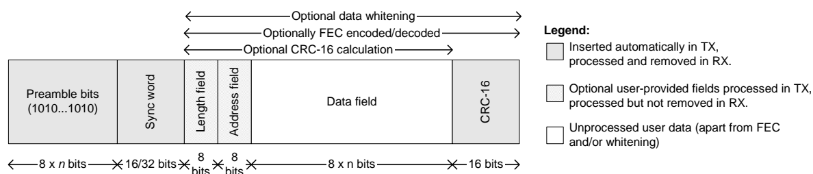
Figure 19: Packet Format
