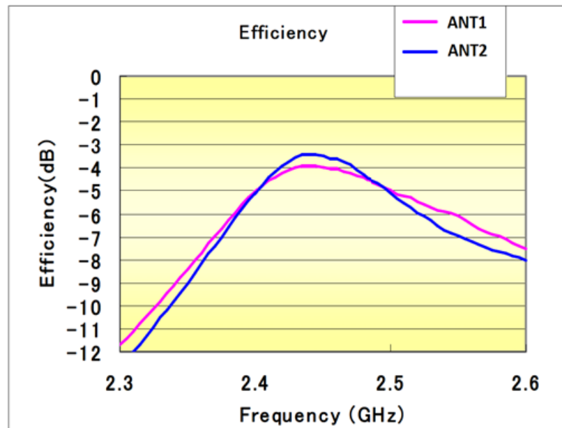
Figure 5. Antenna Efficiency
