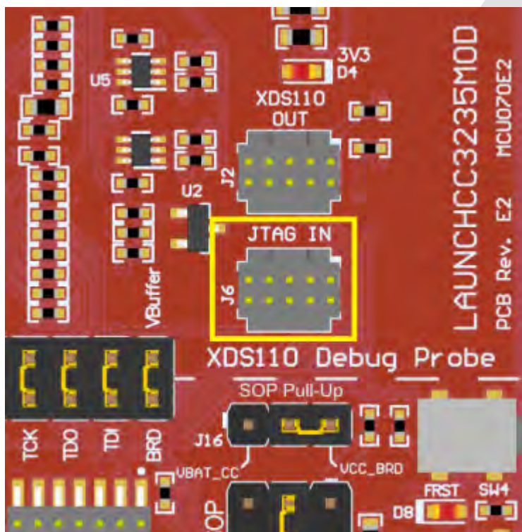
Figure 8. JTAG IN Connector (J6)
