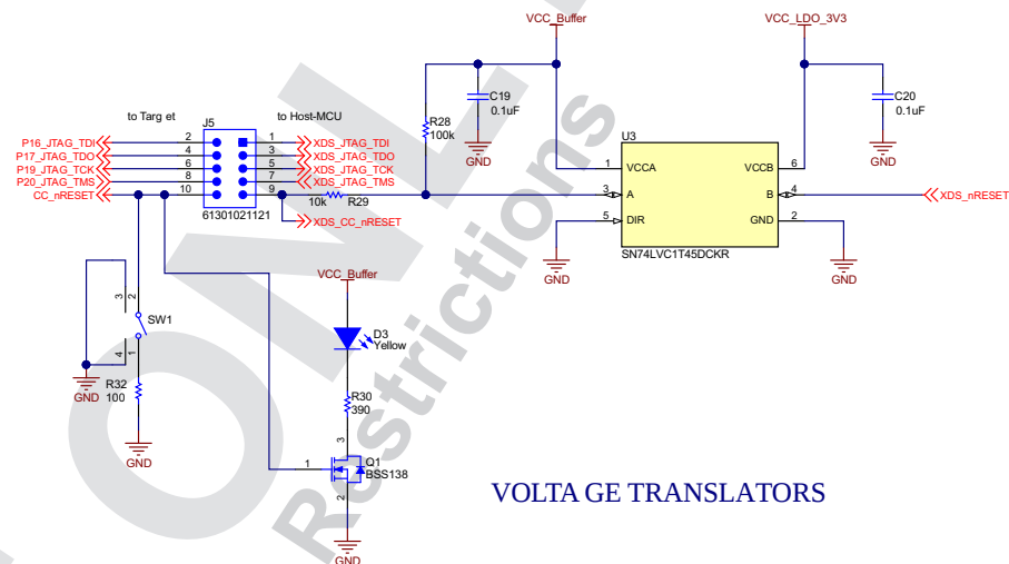
Figure 33. Schematics (2 of 5)
