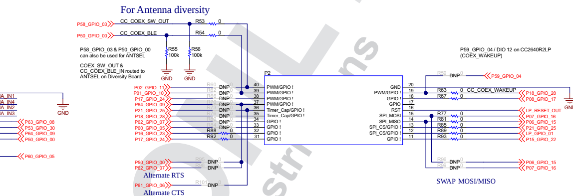
Figure 36. Schematics (5 of 5)
