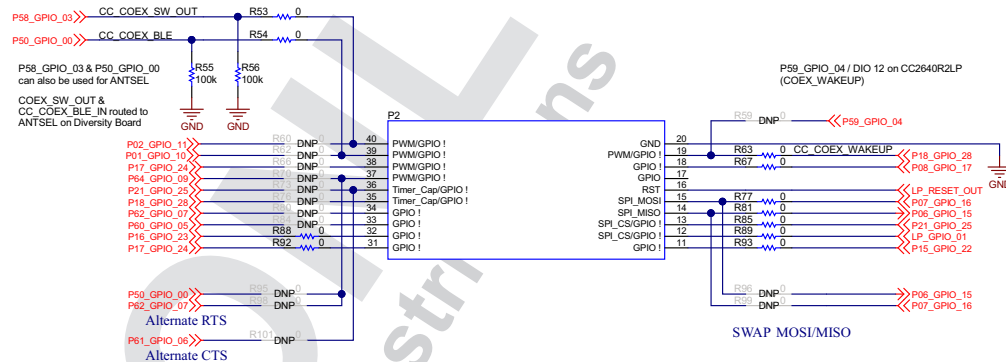
Figure 33. Schematics (5 of 5)
