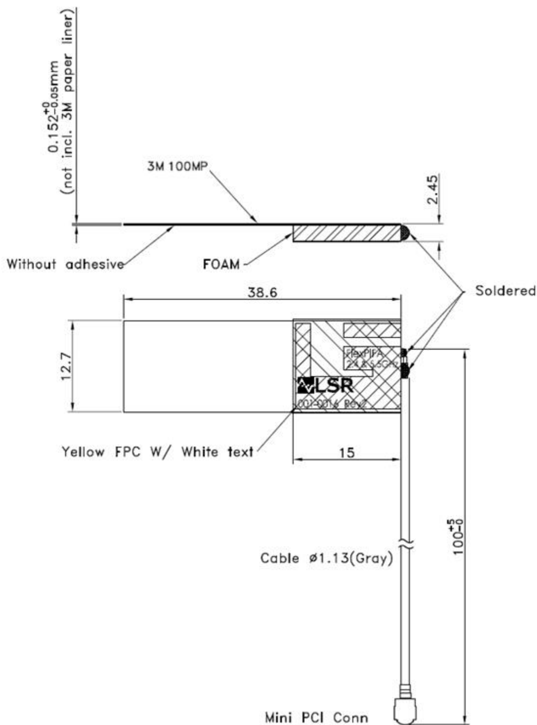
Figure 1 Physical Dimensions
