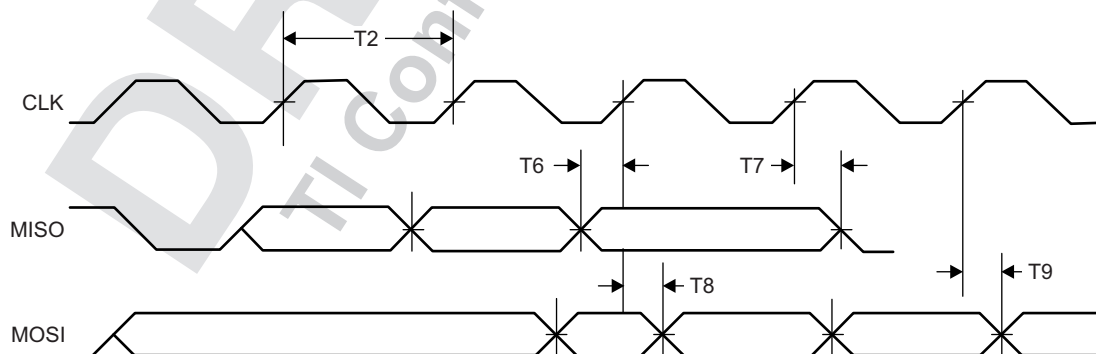
Figure 5-9. Host SPI Timing
