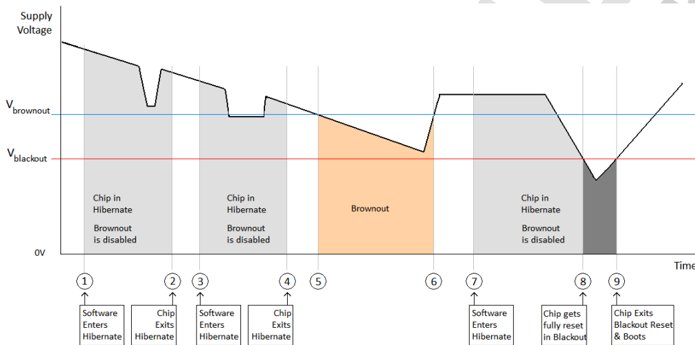
Figure 5-4. Brownout and Blackout Levels (1 of 2)
