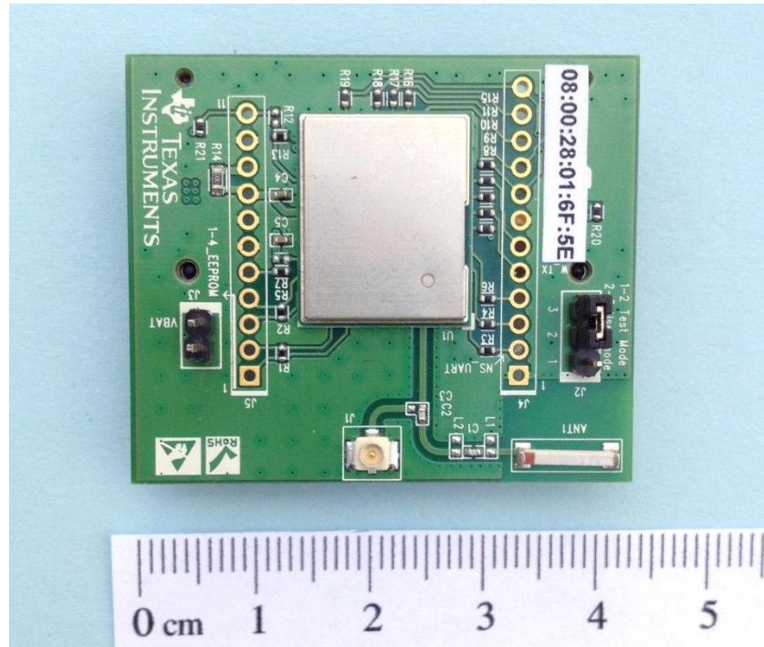
Top side of board
