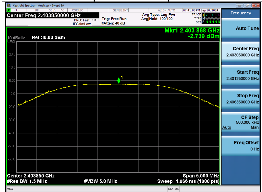
Test_Graph_2.4G_ANT1_2403.85_Peak Power
