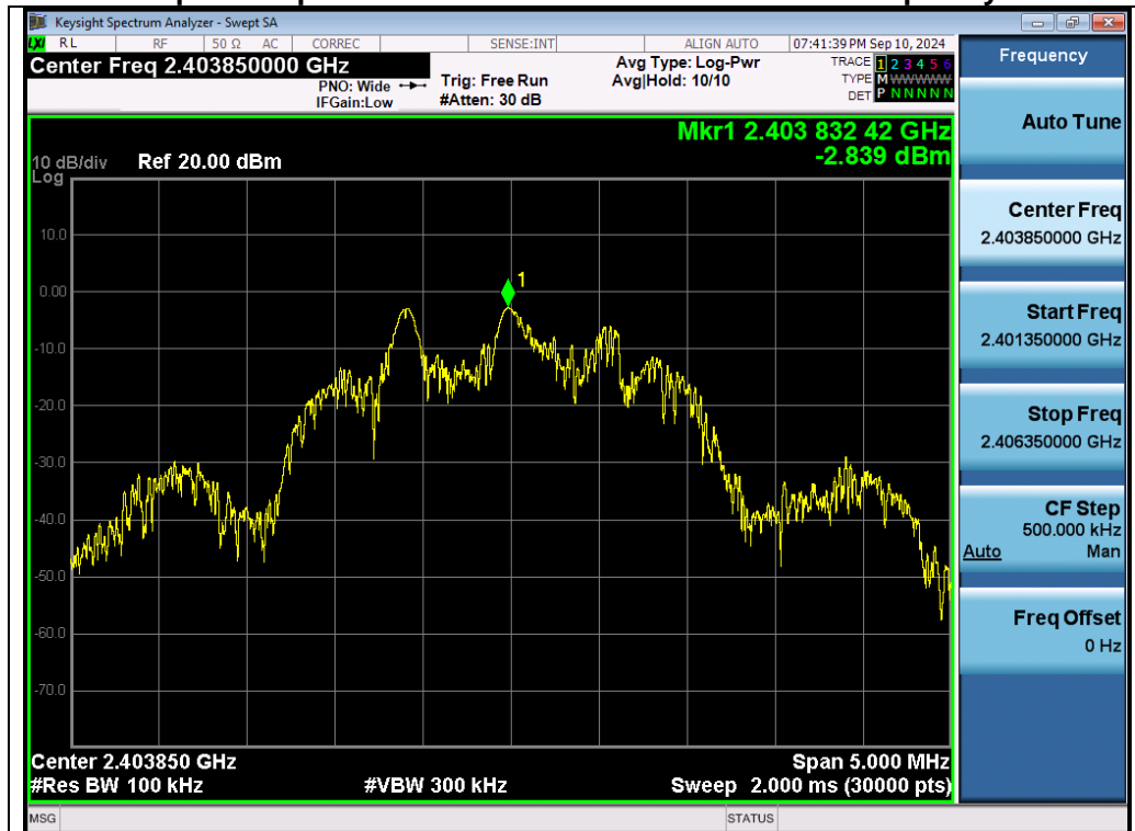
Test_Graph_2.4G_ANT1_2403.85_Reference Level
