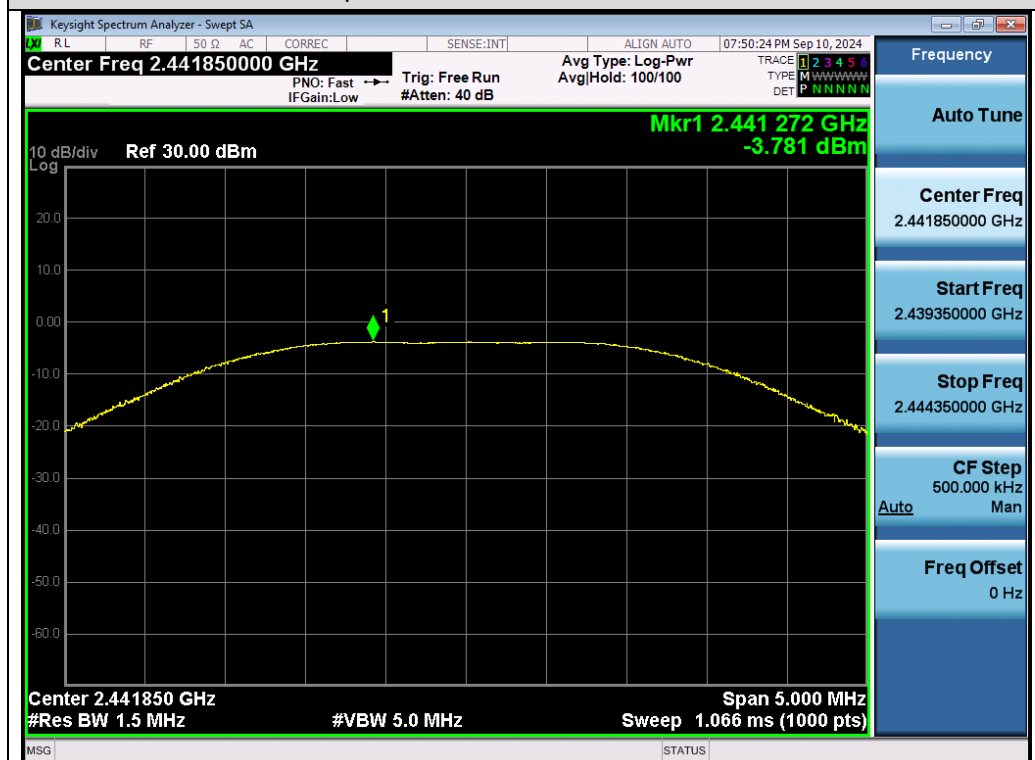
Test_Graph_2.4G_ANT1_2441.85_Peak Power
