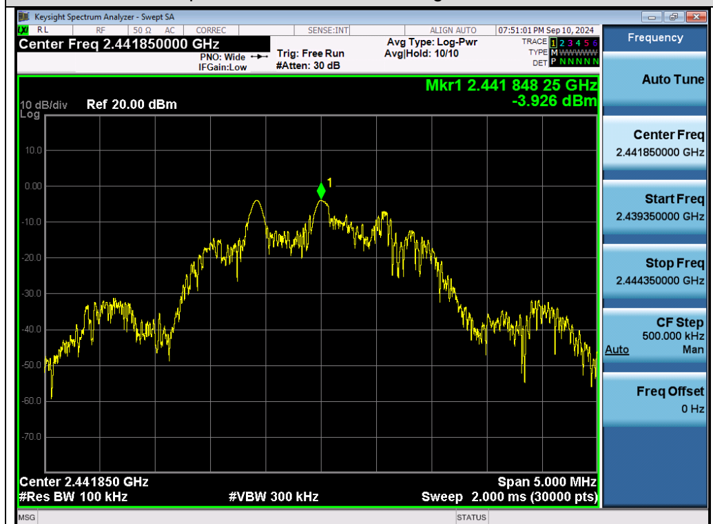
Test_Graph_2.4G_ANT1_2441.85_Reference Level
