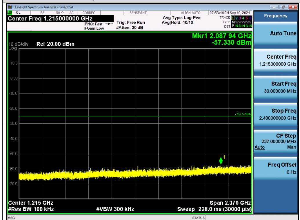
Test_Graph_2.4G_ANT1_2480.85_Lower Band Emissions
