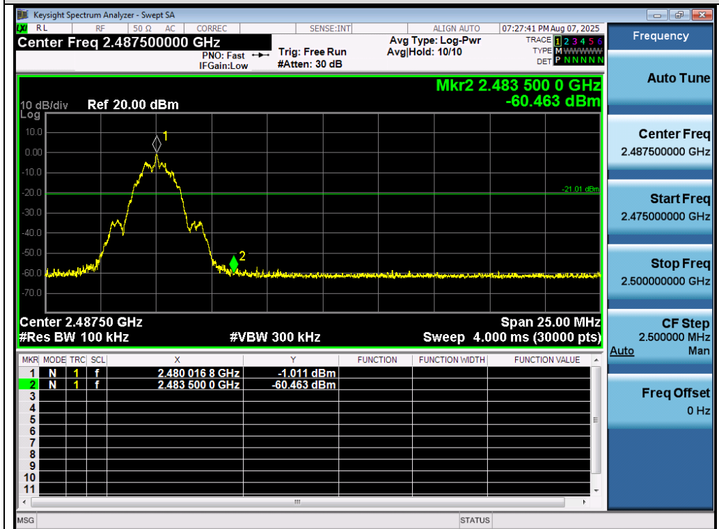
Test_Graph_SRD 2.4G_2480_2Mbps_Higher Band Edge Emissions
