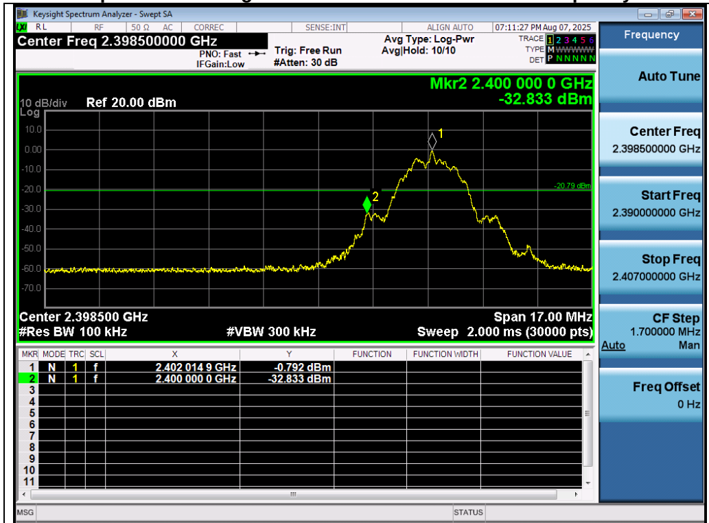
Test_Graph_SRD 2.4G_2402_2Mbps_Lower Band Edge Emissions
