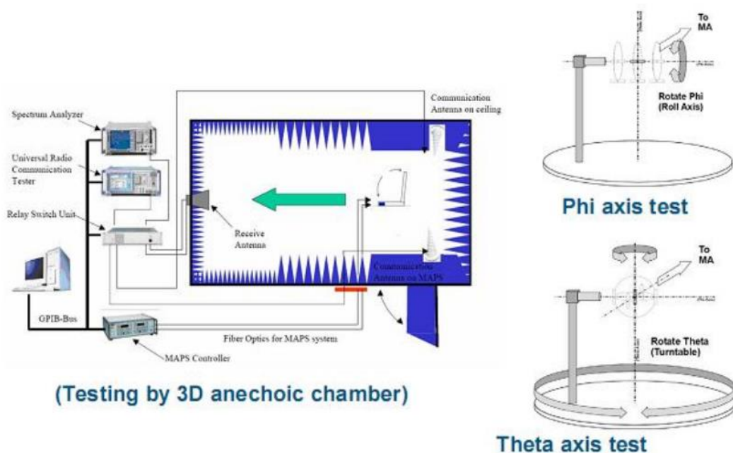
Chart 1 Test topology
