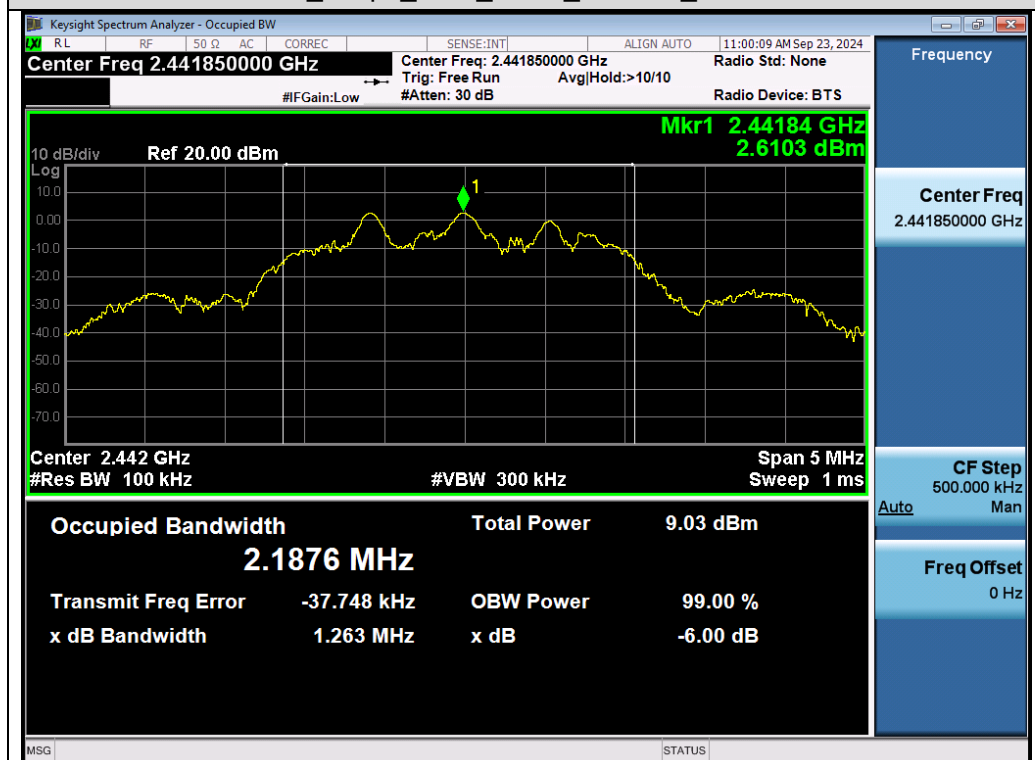
Test_Graph_2.4G_ANT1_2441.85_DTSBW
