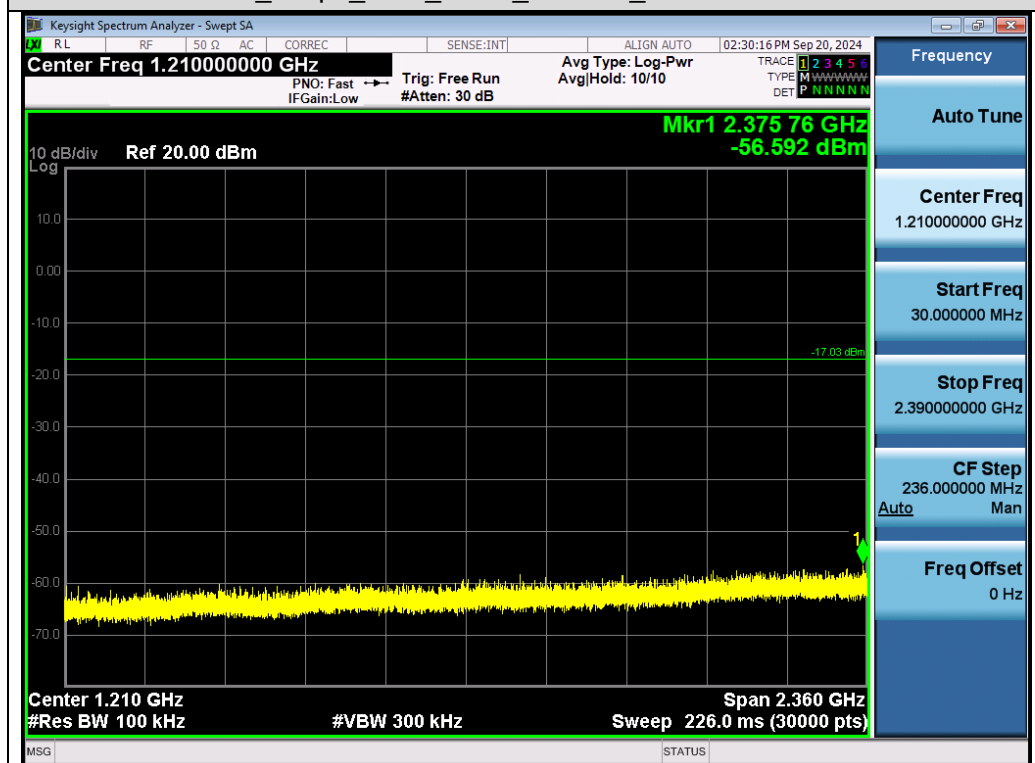
Test_Graph_2.4G_ANT1_2403.85_Lower Band Emissions
