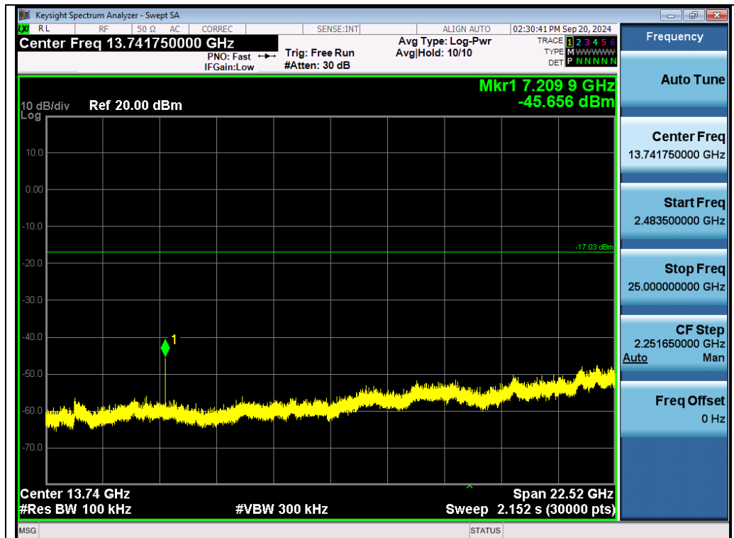
Test_Graph_2.4G_ANT1_2403.85_Higher Band Emissions
