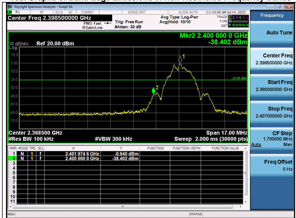
Test_Graph_SRD 2.4G_2402_Lower Band Edge Emissions
