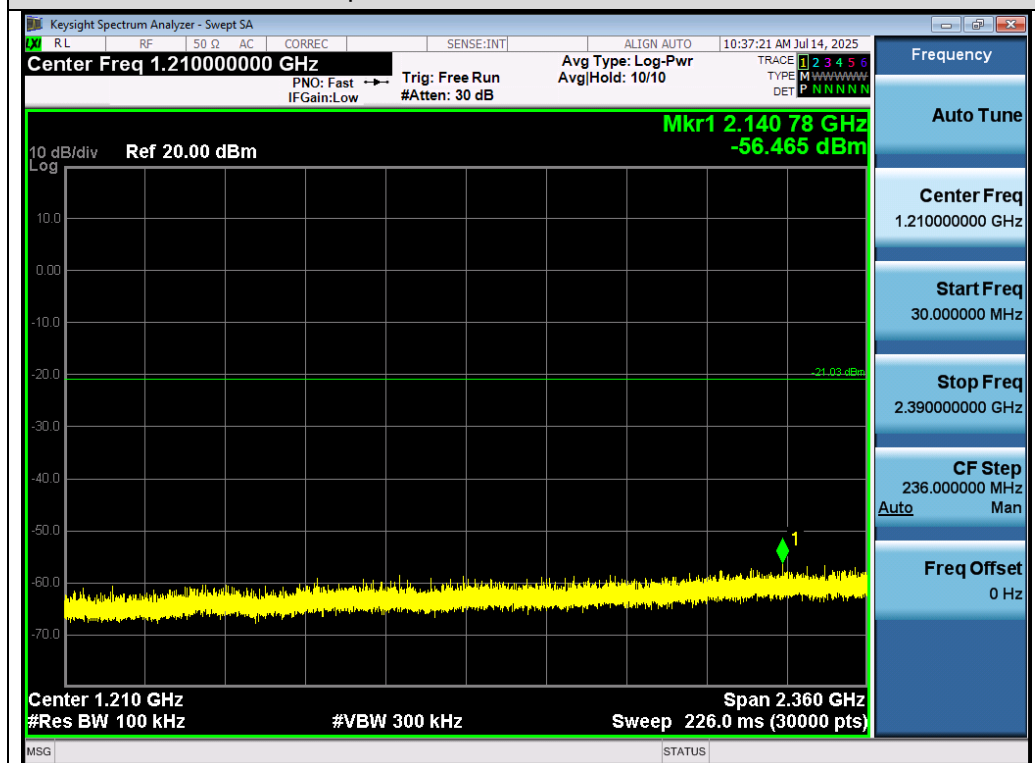
Test_Graph_SRD 2.4G_2402_Lower Band Emissions
