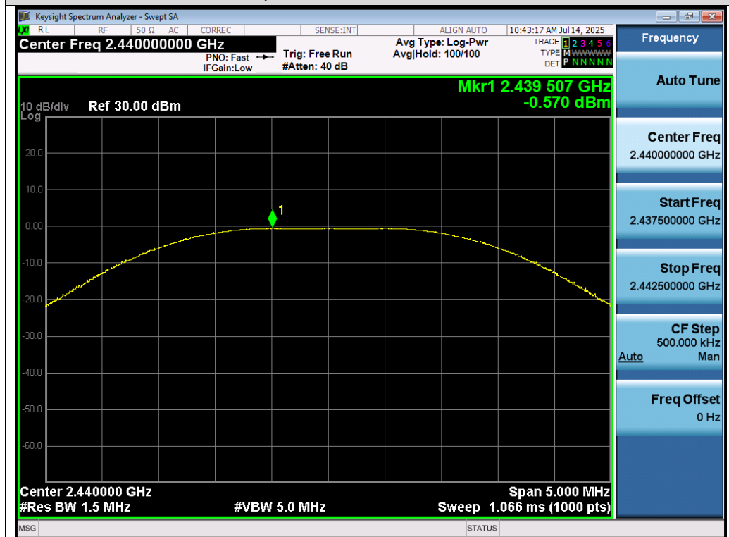
Test_Graph_SRD 2.4G_2440_Peak Power
