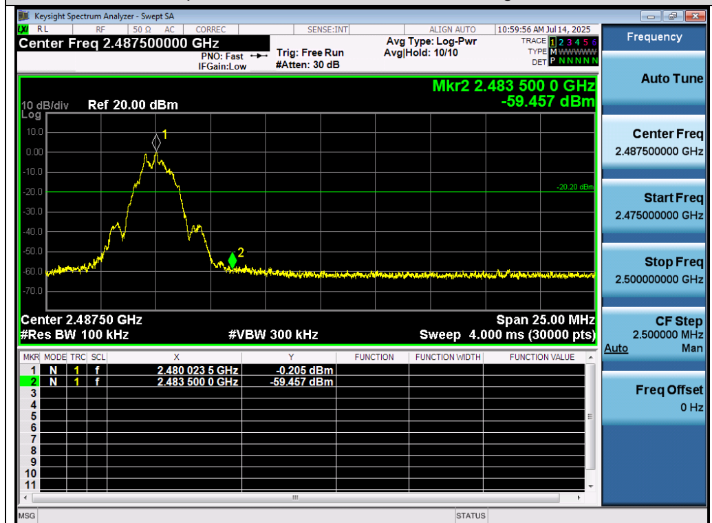
Test_Graph_SRD 2.4G_2480_Higher Band Edge Emissions
