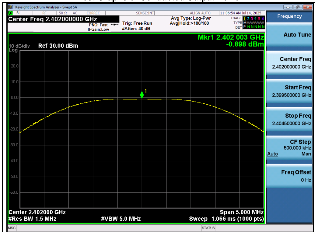
Test_Graph_SRD 2.4G_2402_Peak Power
