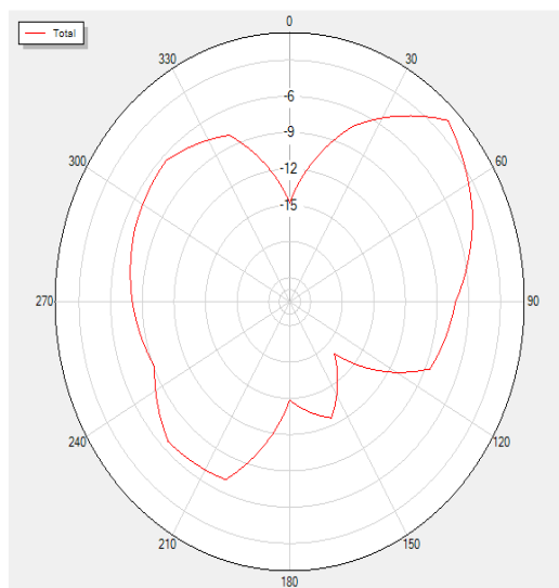
2480P90 Total
