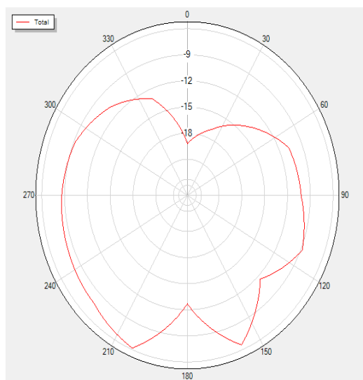
2402P90 Total
