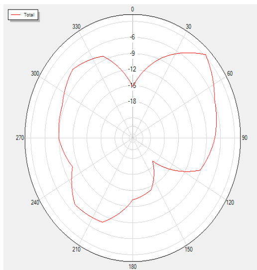
2440P0 Total
