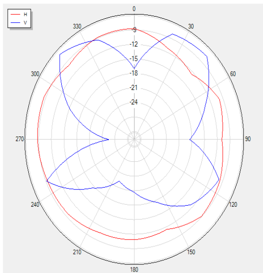
2440P0 Polar
