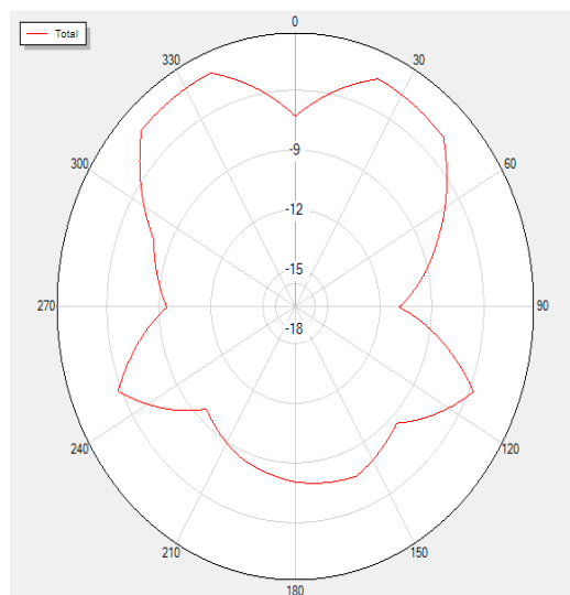
2480T90 Total
