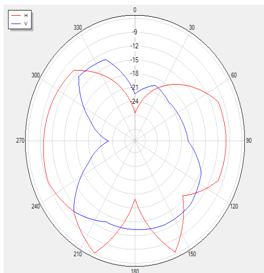
2440T90 Polar
