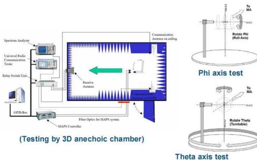
Chart 1 Test topology
