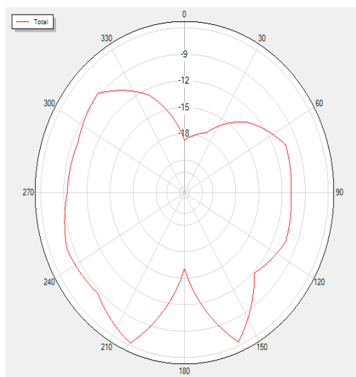
2480P90 Total
