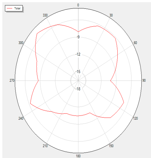
2440P0 Total
