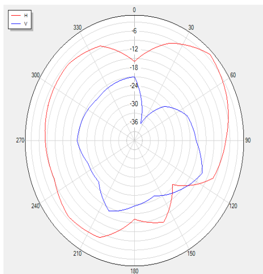
2480P90 Polar
