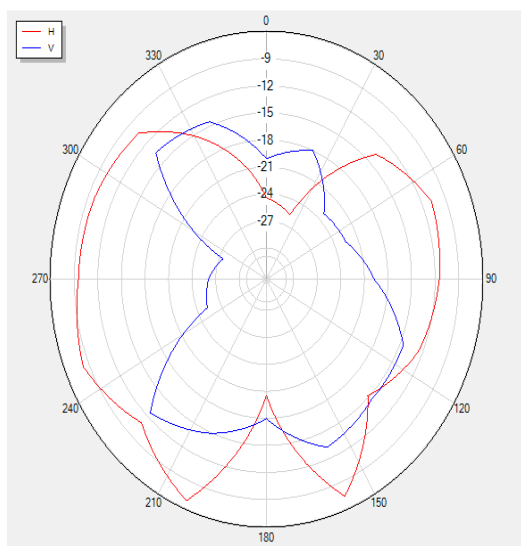
2480P90 Polar
