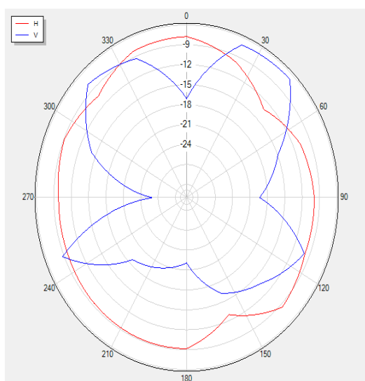
2440T90 Polar
