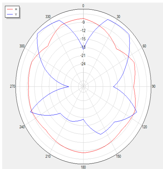
2480T90 Polar
