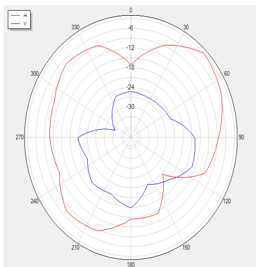
2402P90 Polar
