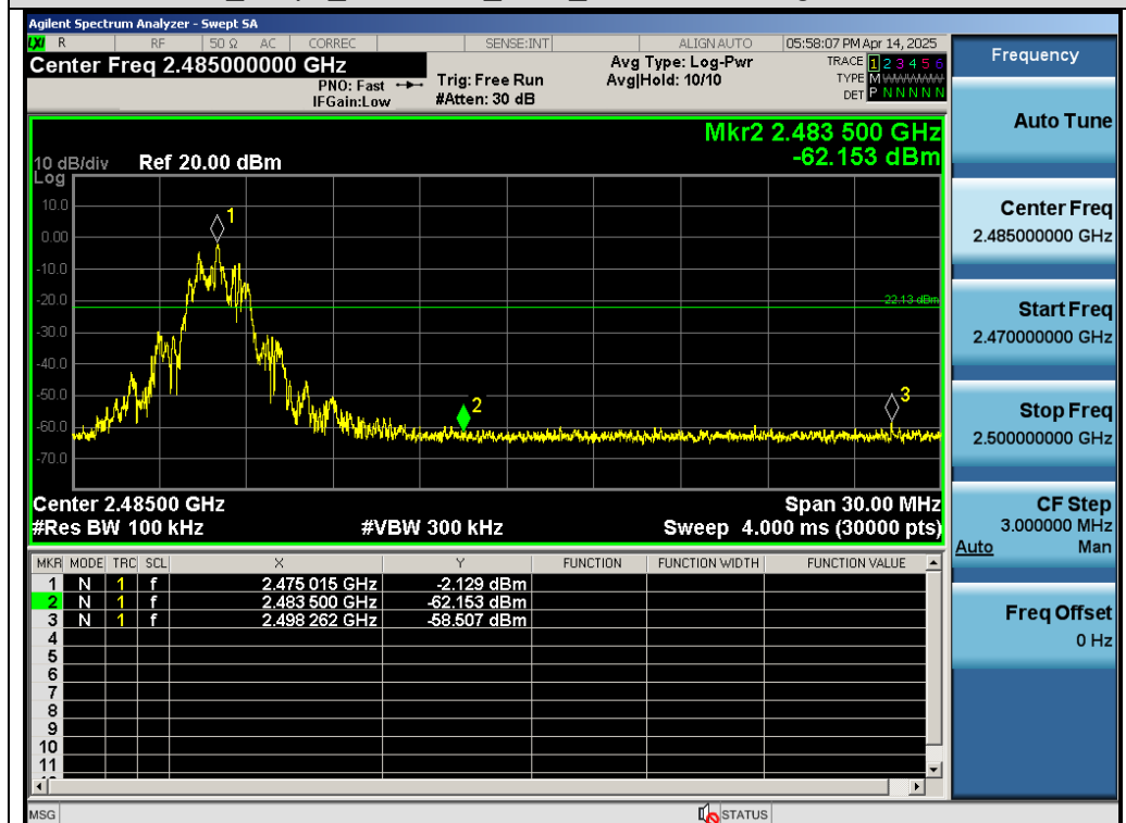
Test_Graph_SRD 2.4G_2475_Higher Band Edge Emissions
