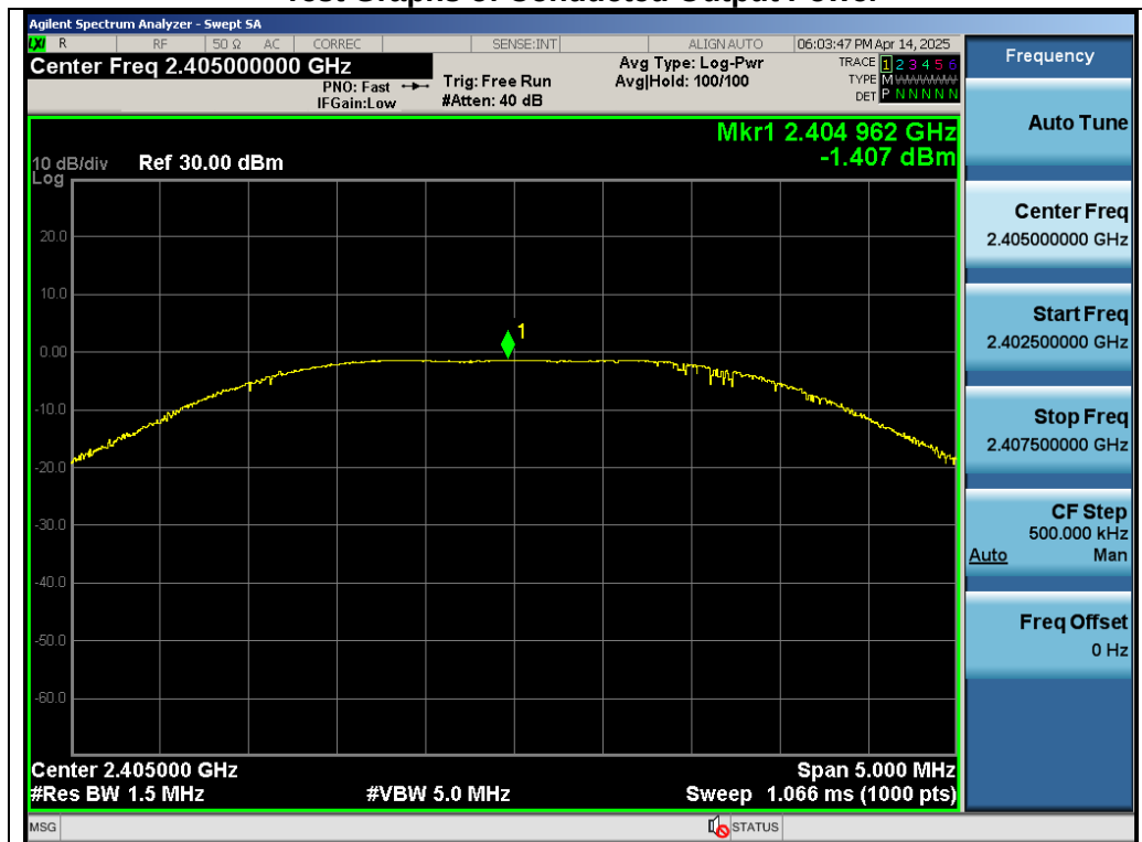
Test_Graph_SRD 2.4G_2405_Peak Power
