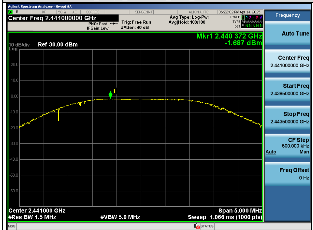
Test_Graph_SRD 2.4G_2441_Peak Power
