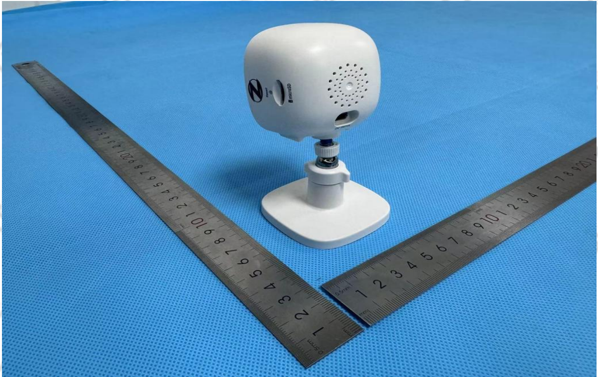
LEFT VIEW OF EUT
