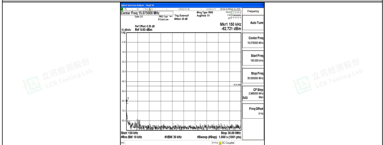
Band41_20MHz_16QAM_39750_1RB#0_0.15~30_0.15~30
