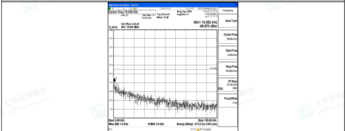
Band41_20MHz_QPSK_39750_1RB#0_0.009~0.15_0.009~0.15
