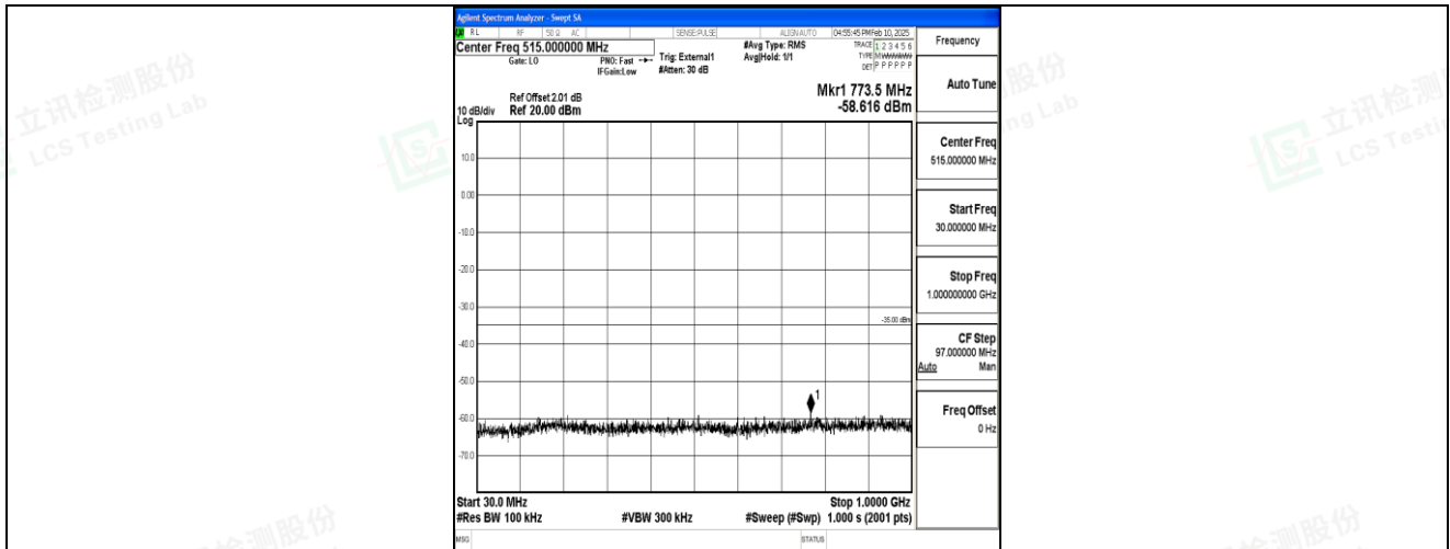
Band41_15MHz_16QAM_39725_1RB#0_30~1000_30~1000
