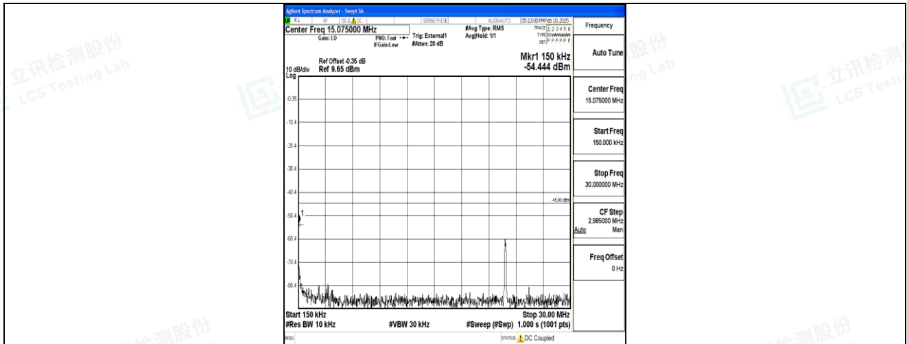
Band41_20MHz_16QAM_40620_1RB#0_0.15~30_0.15~30
