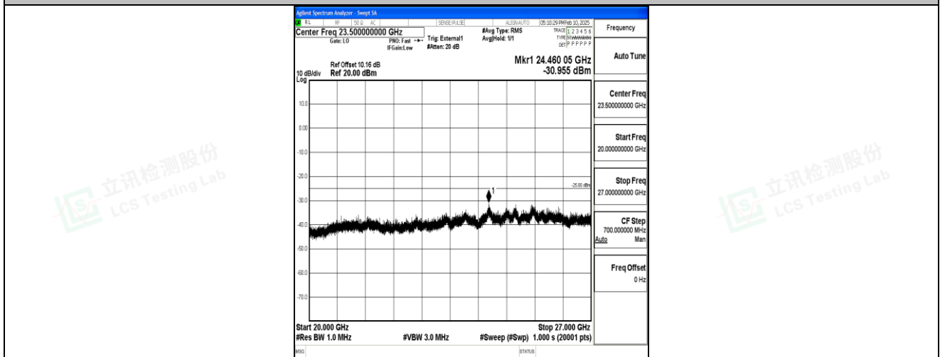
Band41_20MHz_16QAM_39750_1RB#0_20000~27000_20000~27000
