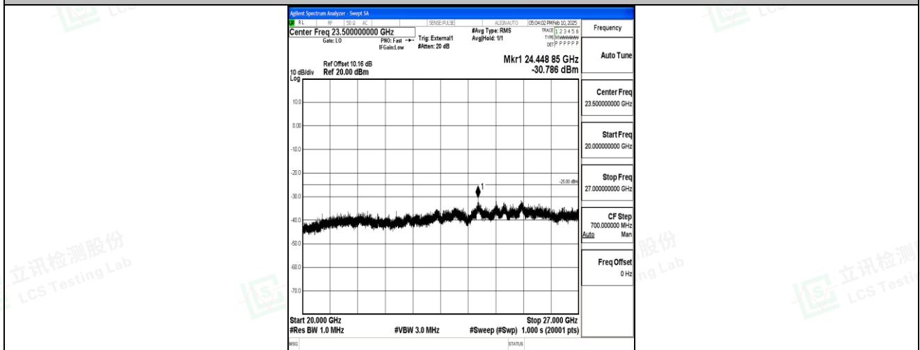
Band41_15MHz_16QAM_41515_1RB#0_20000~27000_20000~27000
