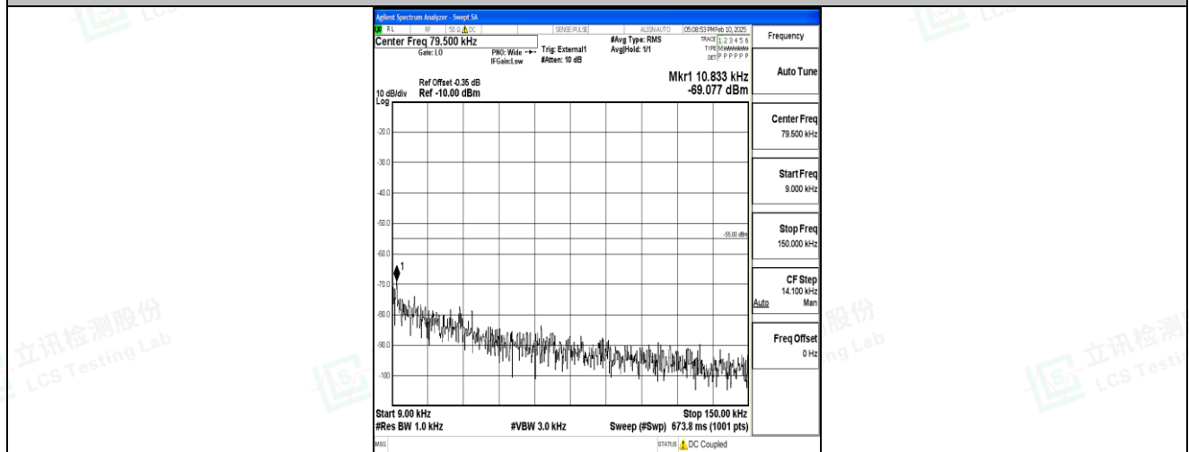
Band41_20MHz_16QAM_39750_1RB#0_0.009~0.15_0.009~0.15
