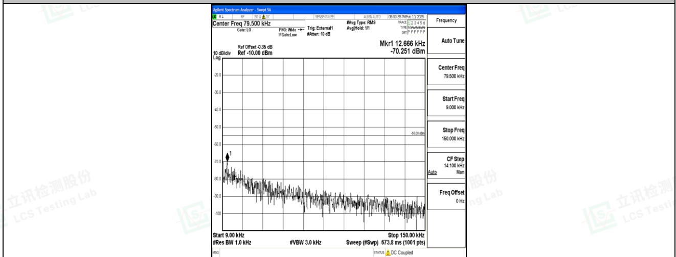
Band41_15MHz_QPSK_41515_1RB#0_0.009-0.15_0.009-0.15
