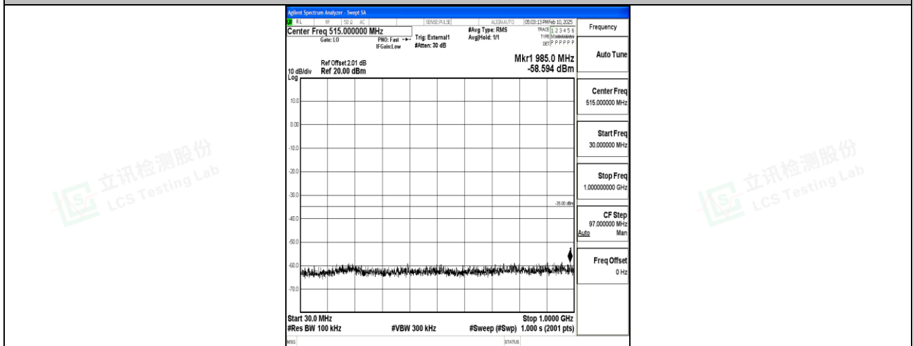
Band41_15MHz_16QAM_41515_1RB#0_30~1000_30~1000
