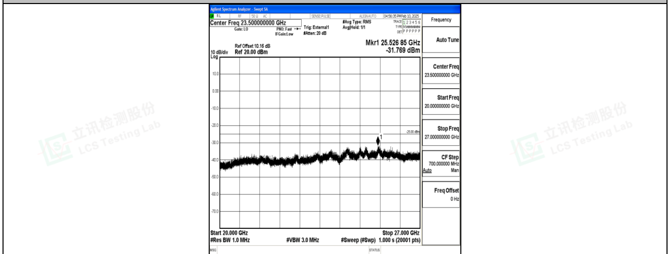
Band41_15MHz_16QAM_39725_1RB#0_20000~27000_20000~27000
