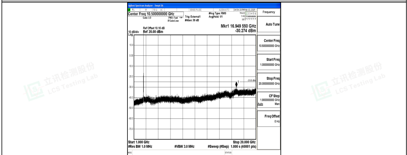
Band41_15MHz_QPSK_39725_1RB#0_1000~20000_1000~20000
