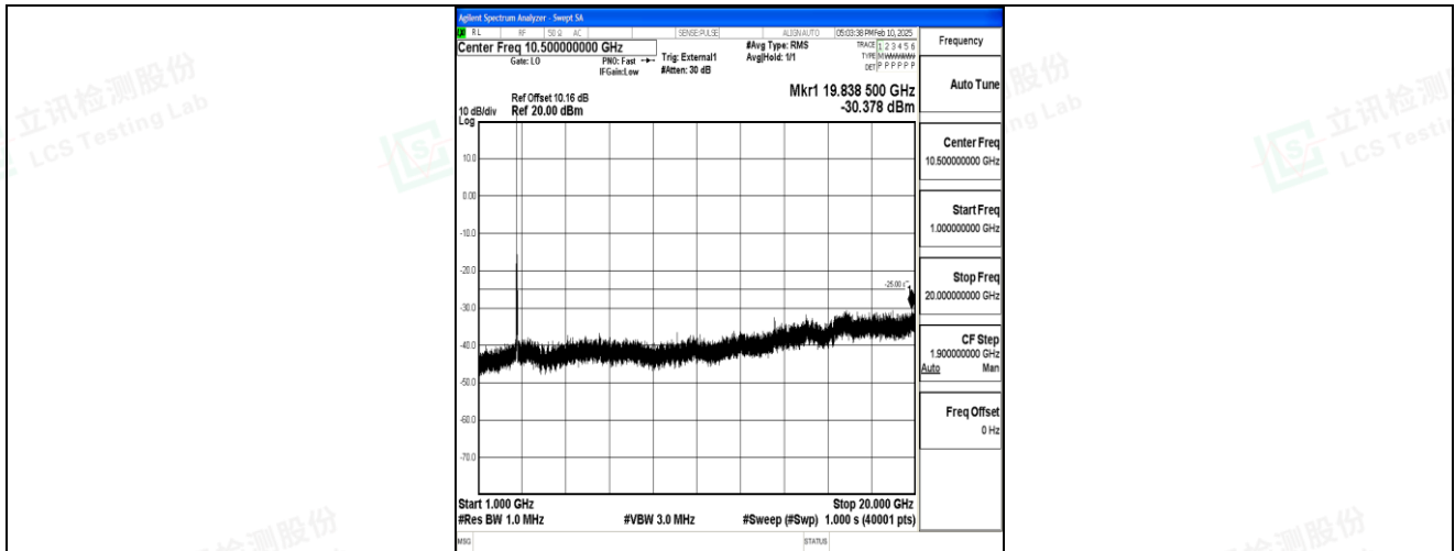
Band41_15MHz_16QAM_41515_1RB#0_1000~20000_1000~20000
