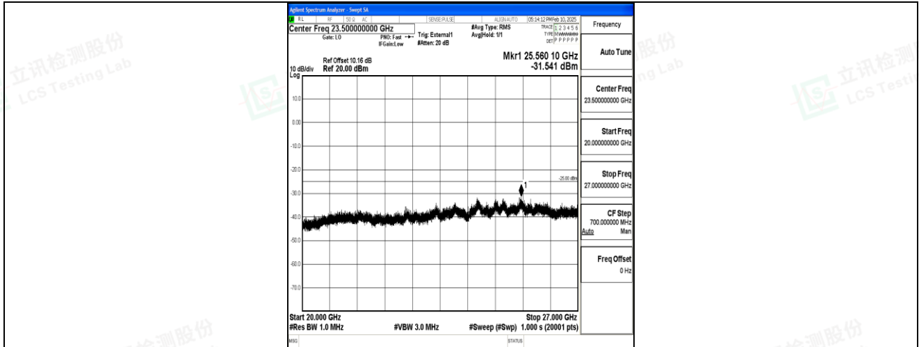
Band41_20MHz_16QAM_40620_1RB#0_20000~27000_20000~27000
