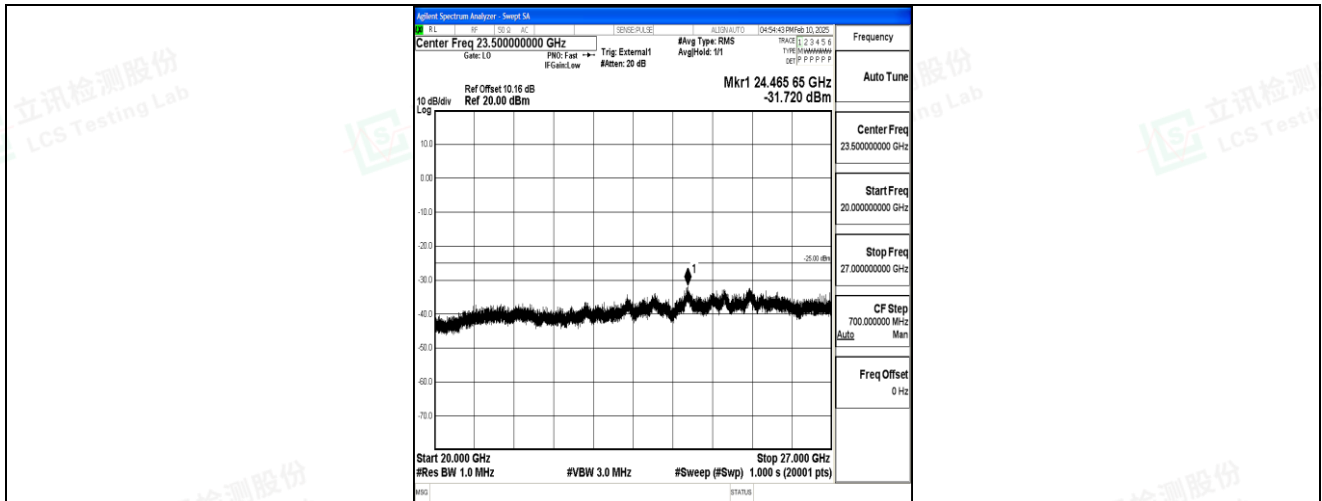
Band41_15MHz_QPSK_39725_1RB#0_20000~27000_20000~27000
