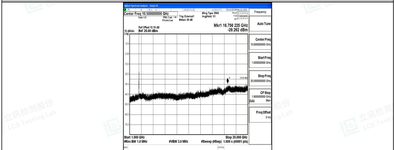
Band41_20MHz_16QAM_39750_1RB#0_1000~20000_1000~20000
