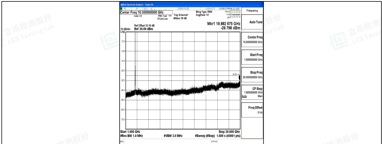
Band41_15MHz_QPSK_40620_1RB#0_1000~20000_1000~20000
