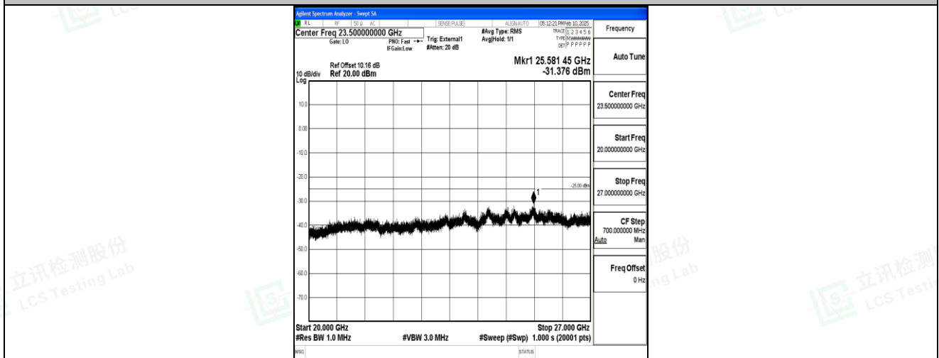
Band41_20MHz_QPSK_40620_1RB#0_20000~27000_20000~27000
