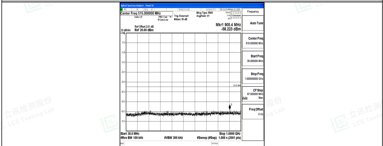
Band41_20MHz_16QAM_40620_1RB#0_30~1000_30~1000
