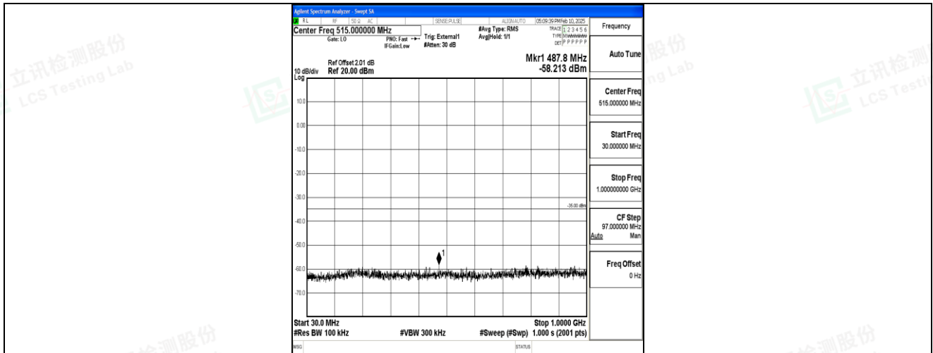
Band41_20MHz_16QAM_39750_1RB#0_30~1000_30~1000
