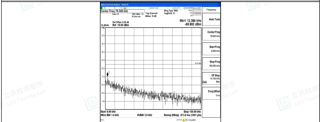
Band41_15MHz_16QAM_39725_1RB#0_0.009~0.15_0.009~0.15
