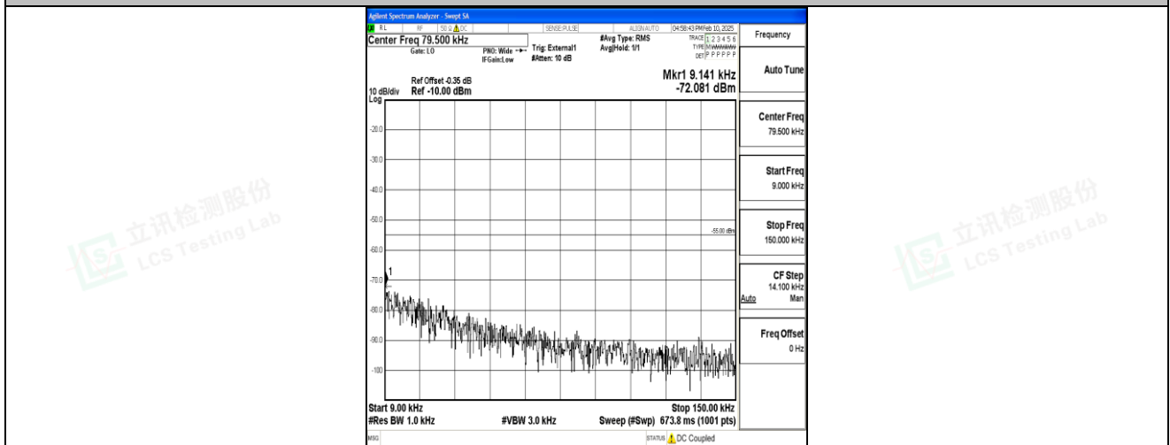
Band41_15MHz_16QAM_40620_1RB#0_0.009~0.15_0.009~0.15
