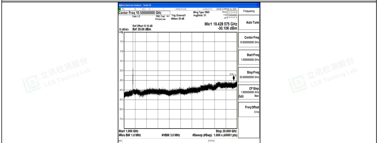
Band41_20MHz_QPSK_39750_1RB#0_1000~20000_1000~20000
