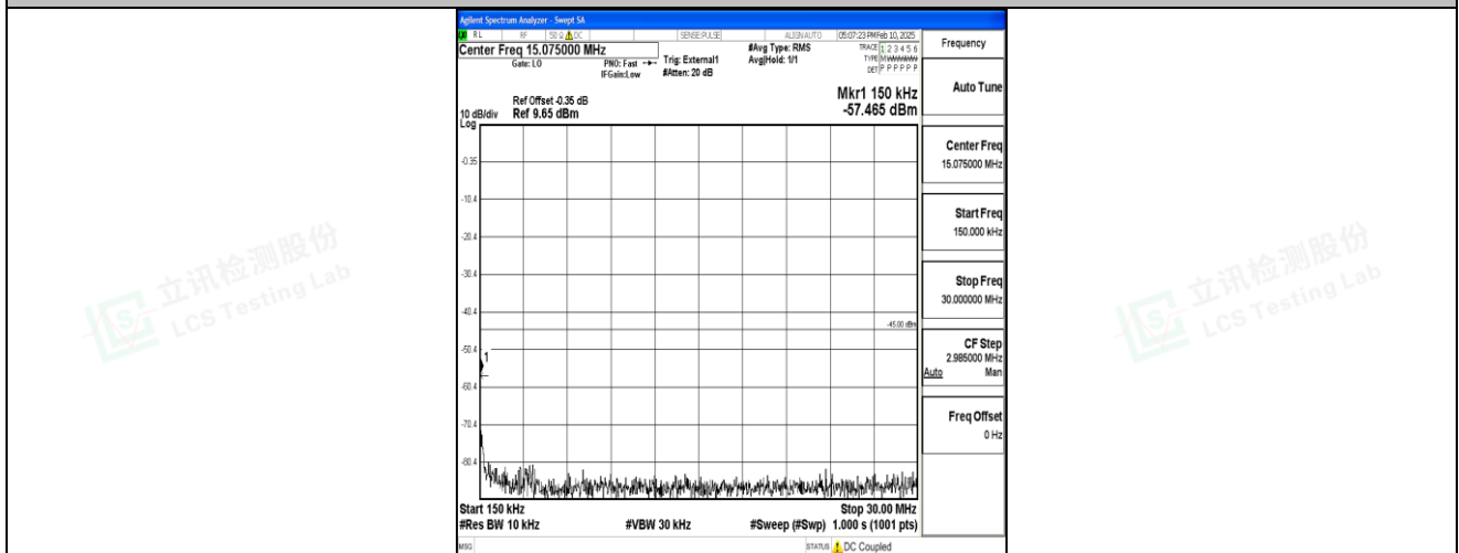
Band41_20MHz_QPSK_39750_1RB#0_0.15~30_0.15~30
