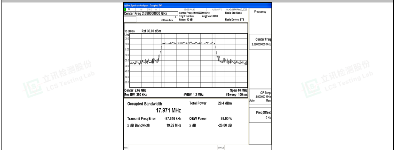
Band41-20MHz-16QAM-41490-100RB#0-PASS
