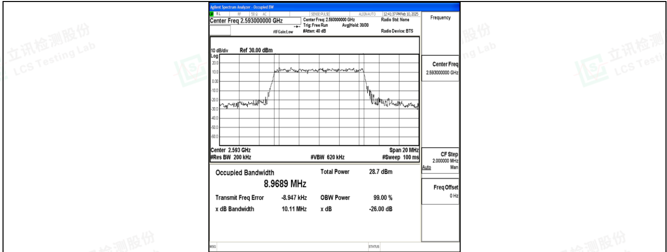
Band41-10MHz-16QAM-40620-50RB#0-PASS
