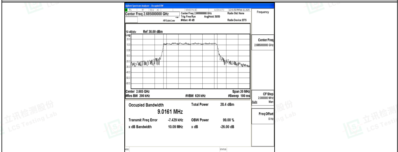
Band41-10MHz-QPSK-41540-50RB#0-PASS
