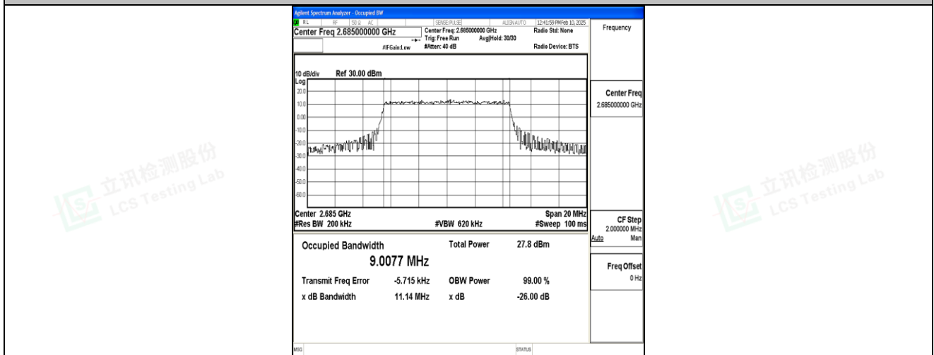
Band41-10MHz-16QAM-41540-50RB#0-PASS
