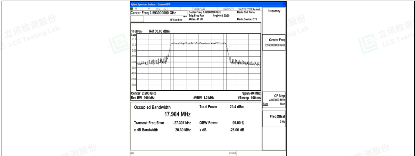
Band41-20MHz-16QAM-40620-100RB#0-PASS
