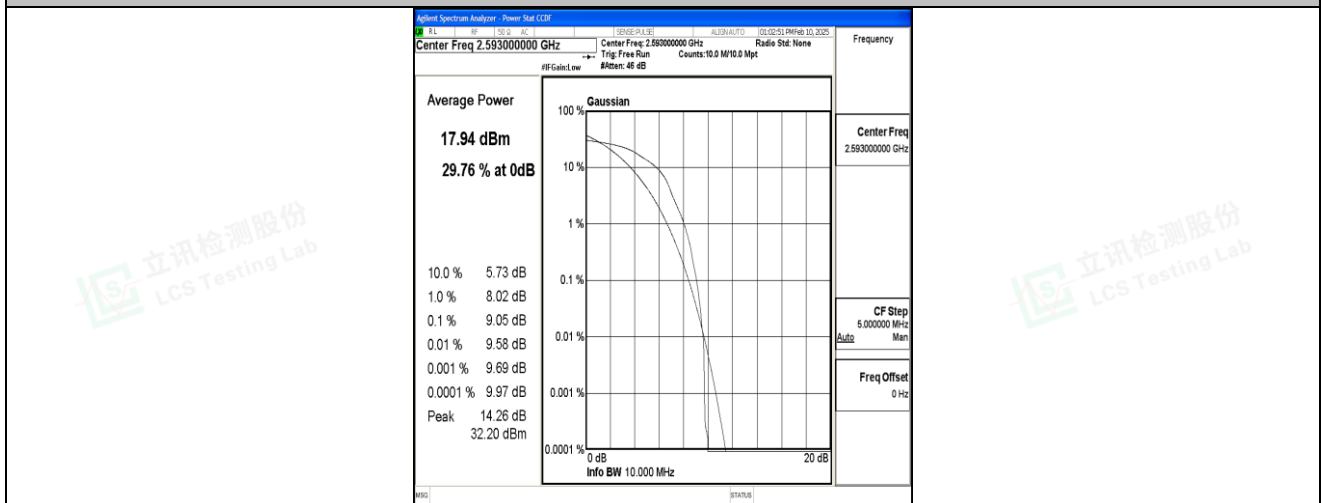
Band41-10MHz-16QAM-40620-1RB#0-PASS
