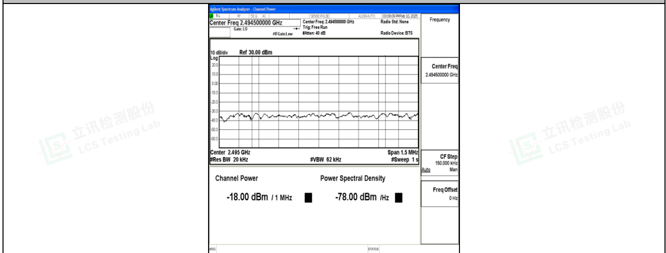
Band41_5MHz_16QAM_39675_25RB#0_Final2
