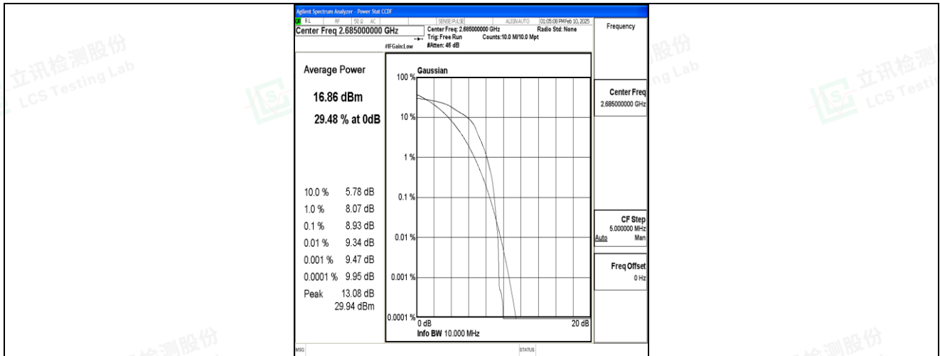
Band41-10MHz-16QAM-41540-1RB#0-PASS
