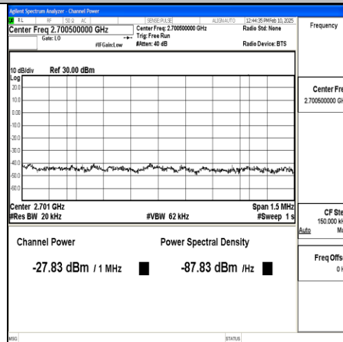
Band41_10MHz_QPSK_41540_50RB#0_Final1
