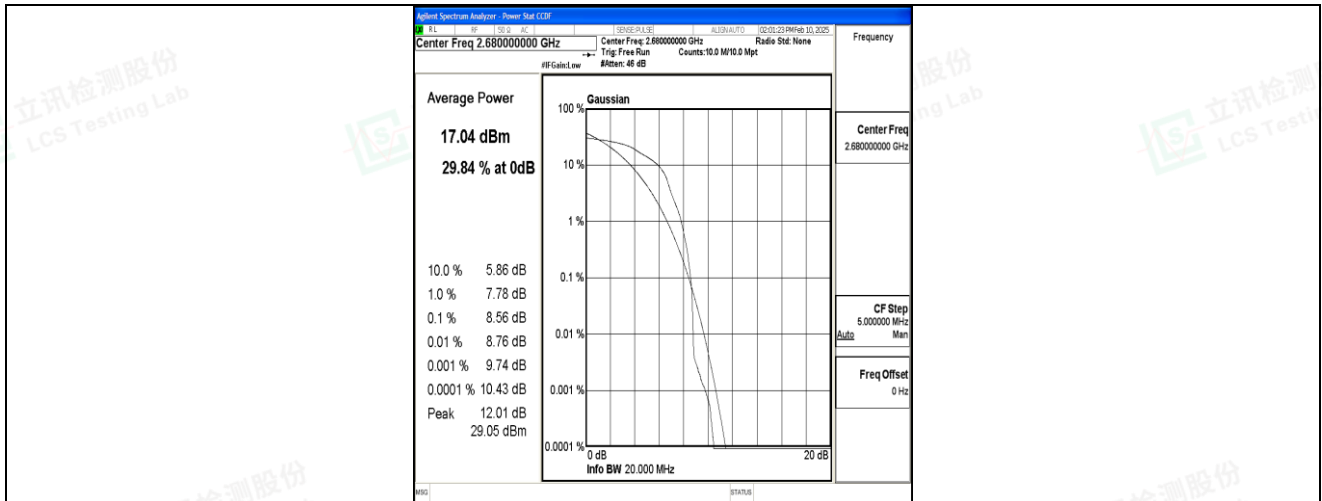
Band41-20MHz-16QAM-41490-1RB#0-PASS
