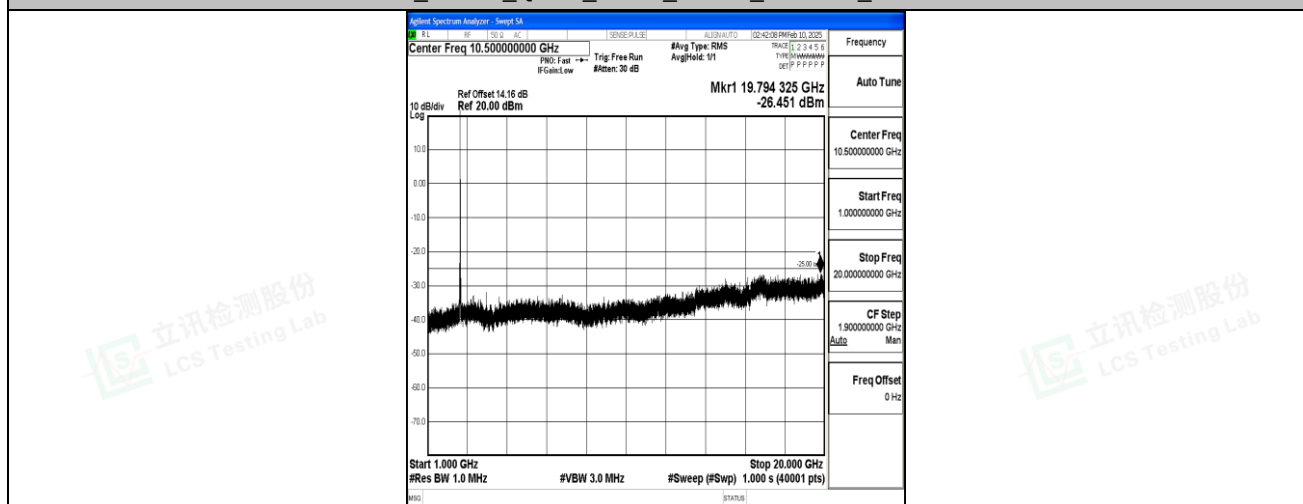
Band7_20MHz_QPSK_21350_1RB#0_1000~20000_1000~20000
