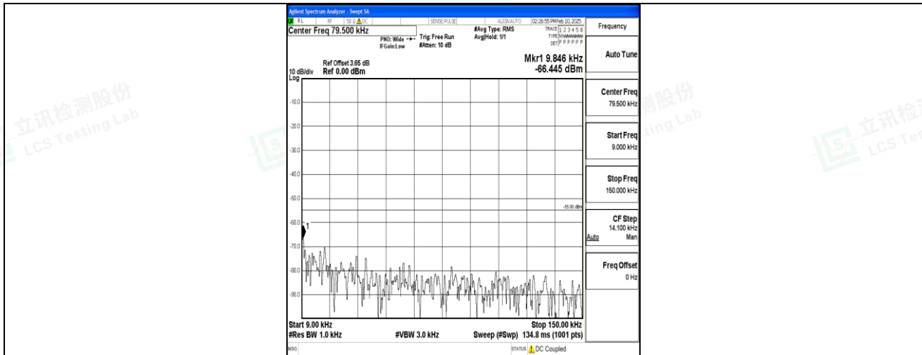
Band7_15MHz_QPSK_20825_1RB#0_0.009~0.15_0.009~0.15
