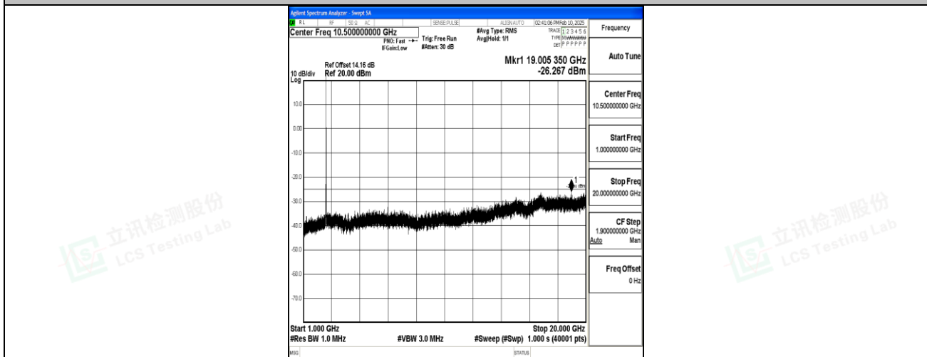
Band7_20MHz_QPSK_21100_1RB#0_1000~20000_1000~20000
