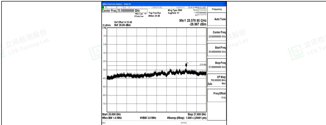
Band7_20MHz_QPSK_21350_1RB#0_20000~27000_20000~27000
