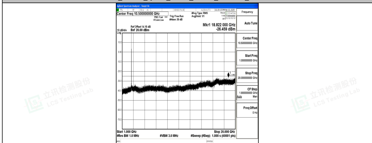
Band7_15MHz_QPSK_21375_1RB#0_1000~20000_1000~20000
