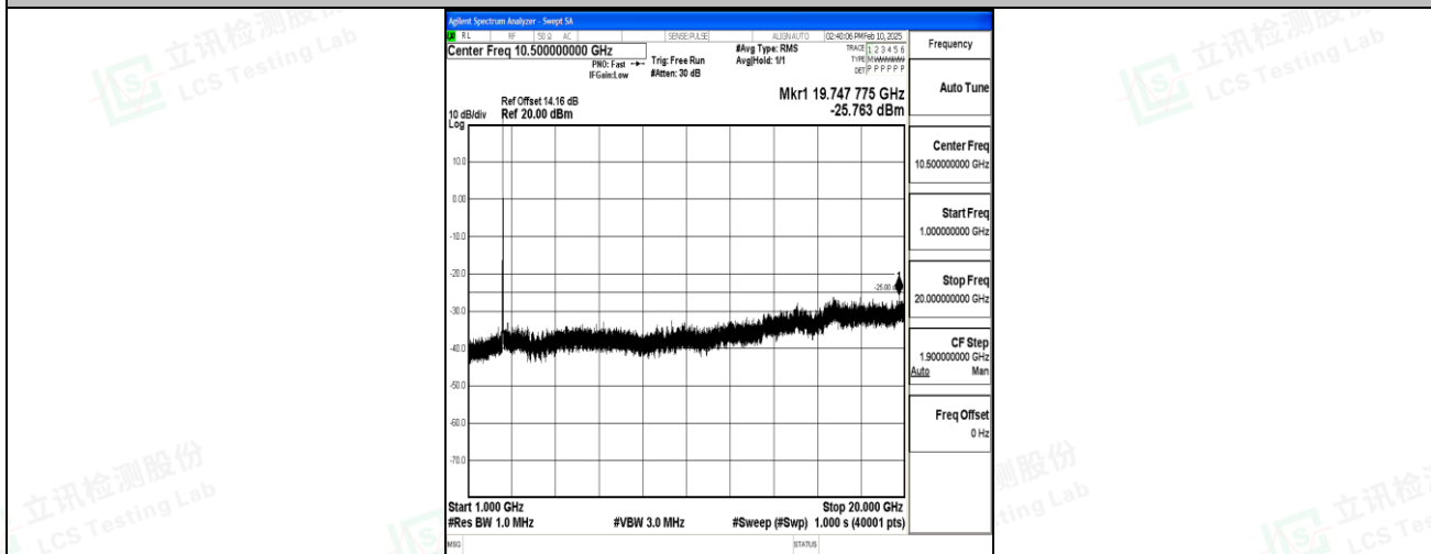
Band7_20MHz_QPSK_20850_1RB#0_1000~20000_1000~20000
