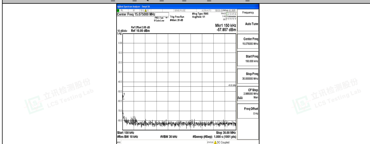
Band7_5MHz_16QAM_21100_1RB#0_0.15~30_0.15~30
