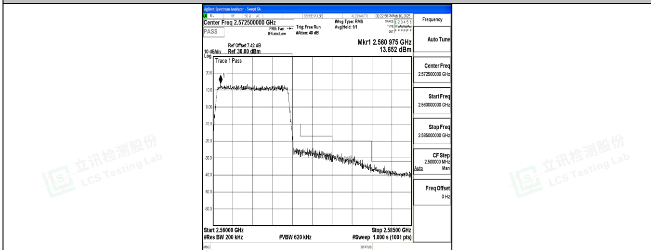
Band7_10MHz_QPSK_21400_50RB#0
