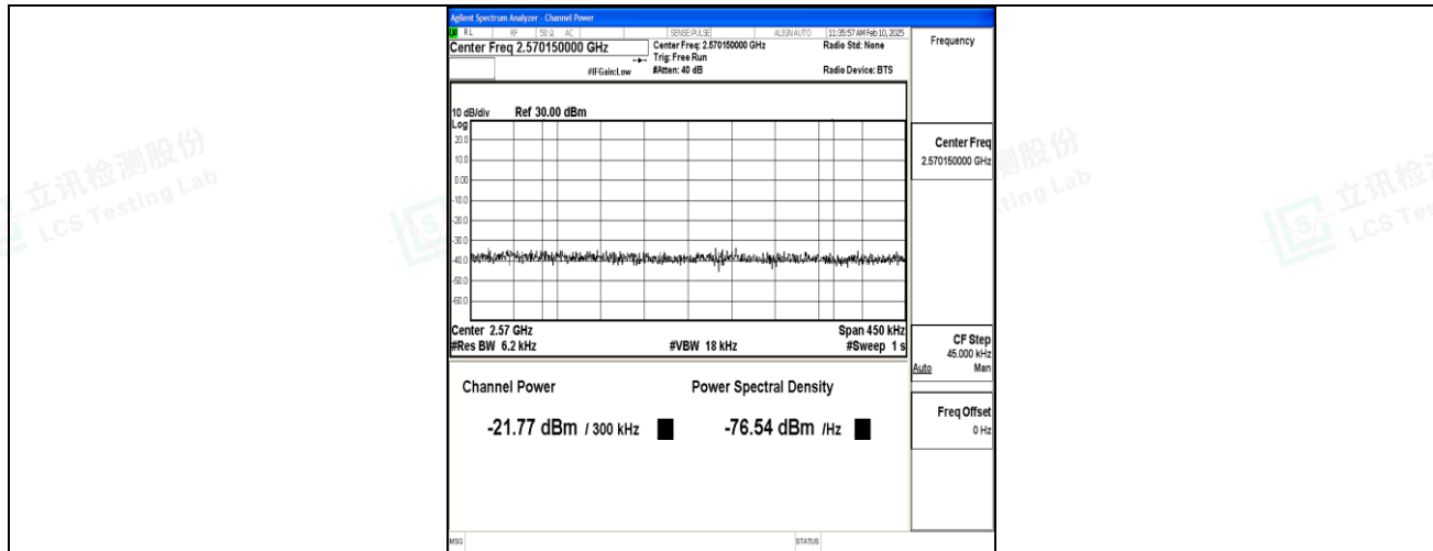
Band7_15MHz_16QAM_21375_75RB#0_Final1
