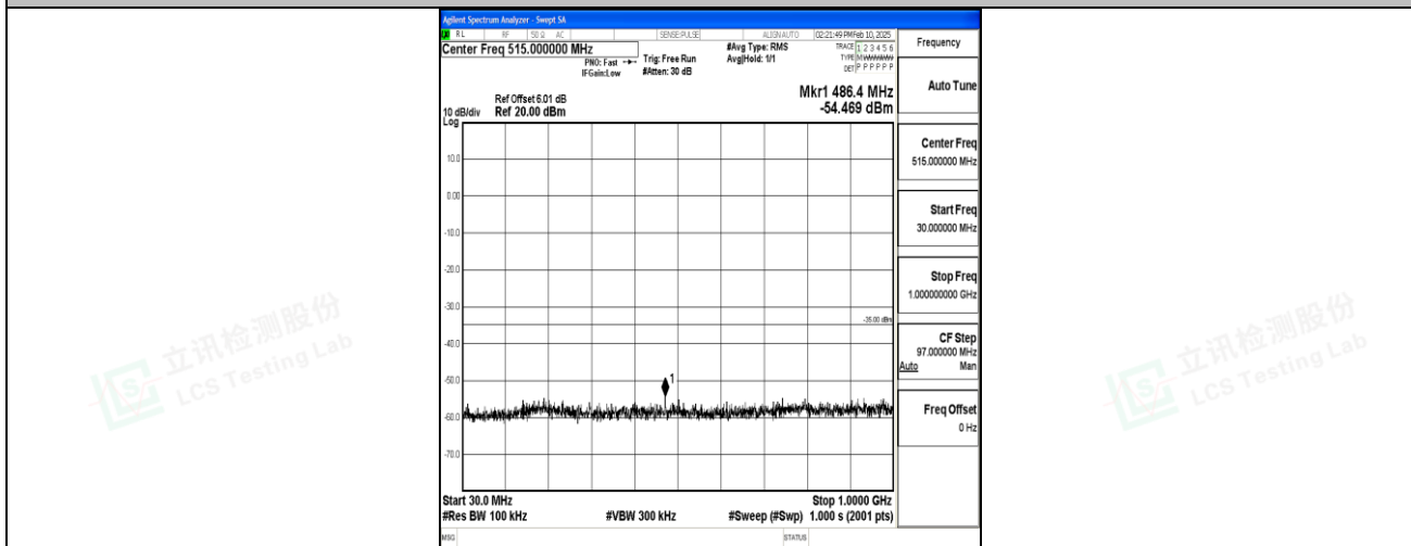
Band7_5MHz_QPSK_21425_1RB#0_30~1000_30~1000
