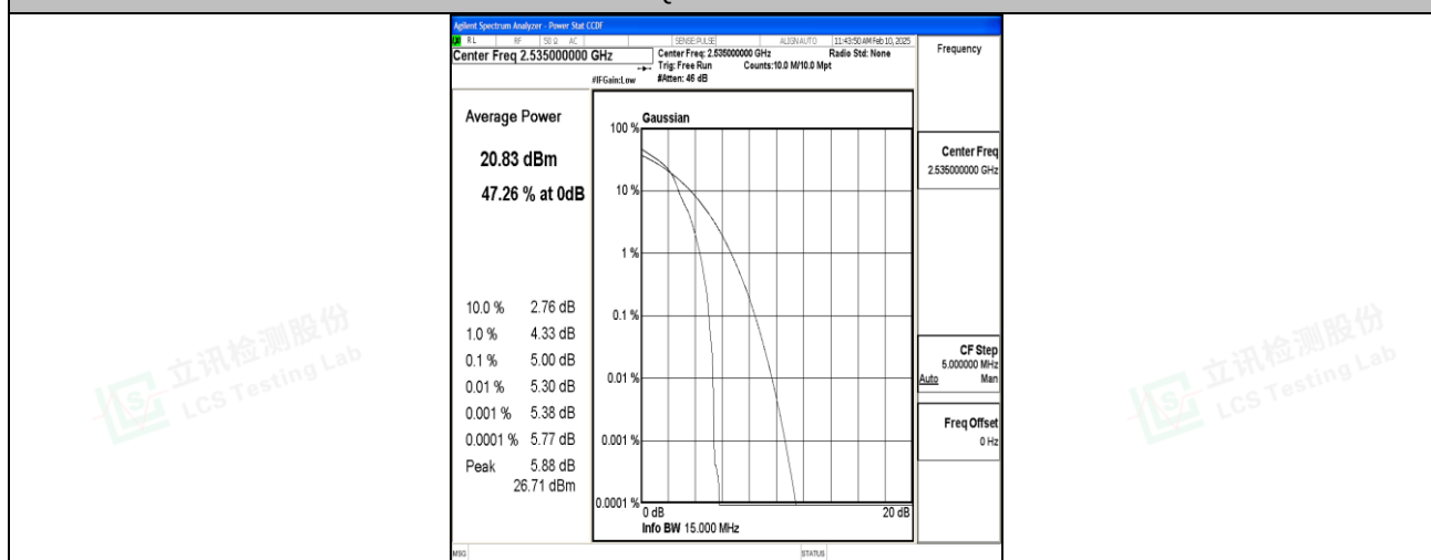
Band7-15MHz-16QAM-21100-1RB#0-PASS
