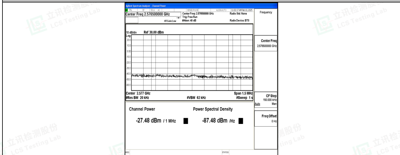
Band7_5MHz_16QAM_21425_25RB#0_Final3
