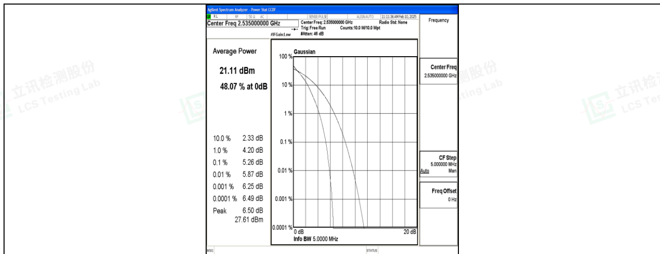
Band7-5MHz-QPSK-21100-25RB#0-PASS
