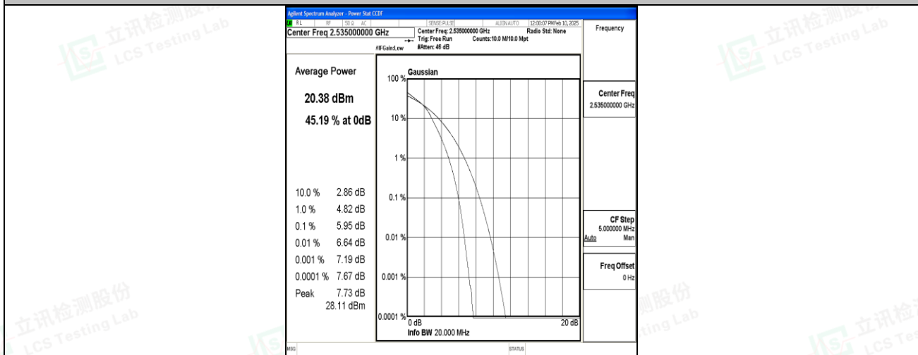
Band7-20MHz-16QAM-21100-100RB#0-PASS
