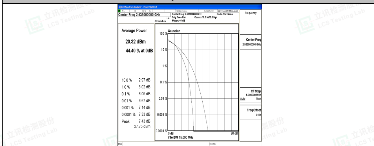
Band7-15MHz-16QAM-21100-75RB#0-PASS
