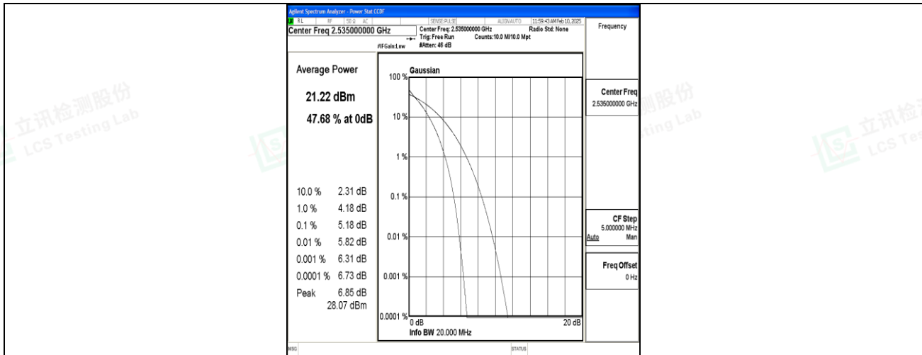
Band7-20MHz-QPSK-21100-100RB#0-PASS
