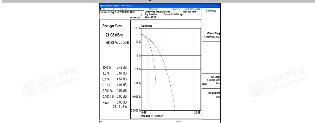
Band7-15MHz-QPSK-21375-1RB#0-PASS
