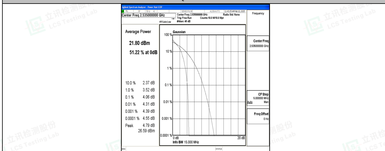
Band7-15MHz-QPSK-21100-1RB#0-PASS
