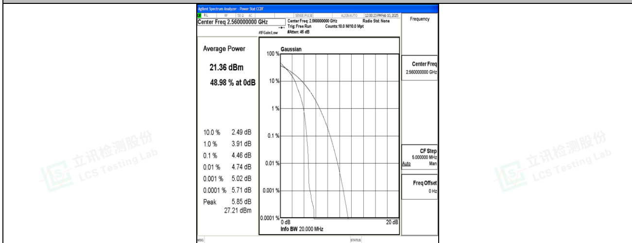
Band7-20MHz-QPSK-21350-1RB#0-PASS
