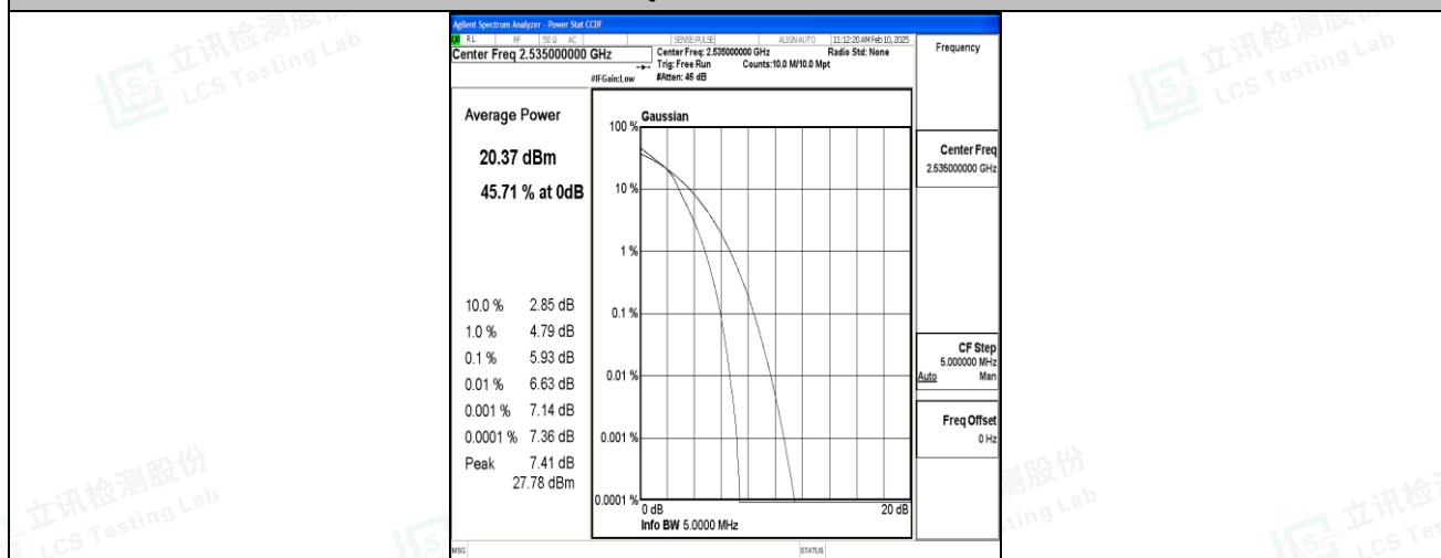
Band7-5MHz-16QAM-21100-25RB#0-PASS
