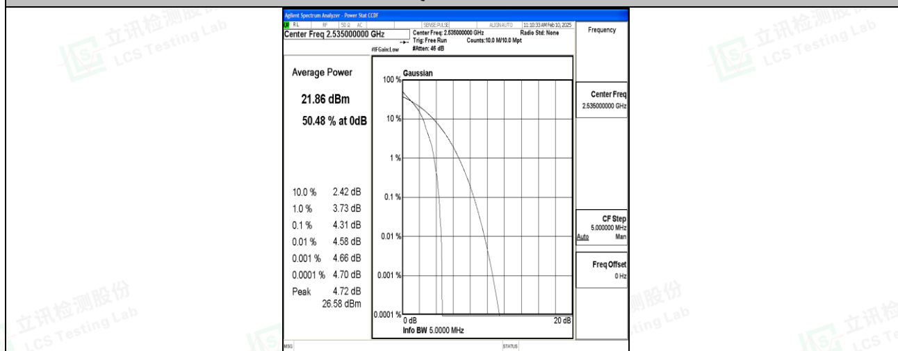
Band7-5MHz-QPSK-21100-1RB#0-PASS
