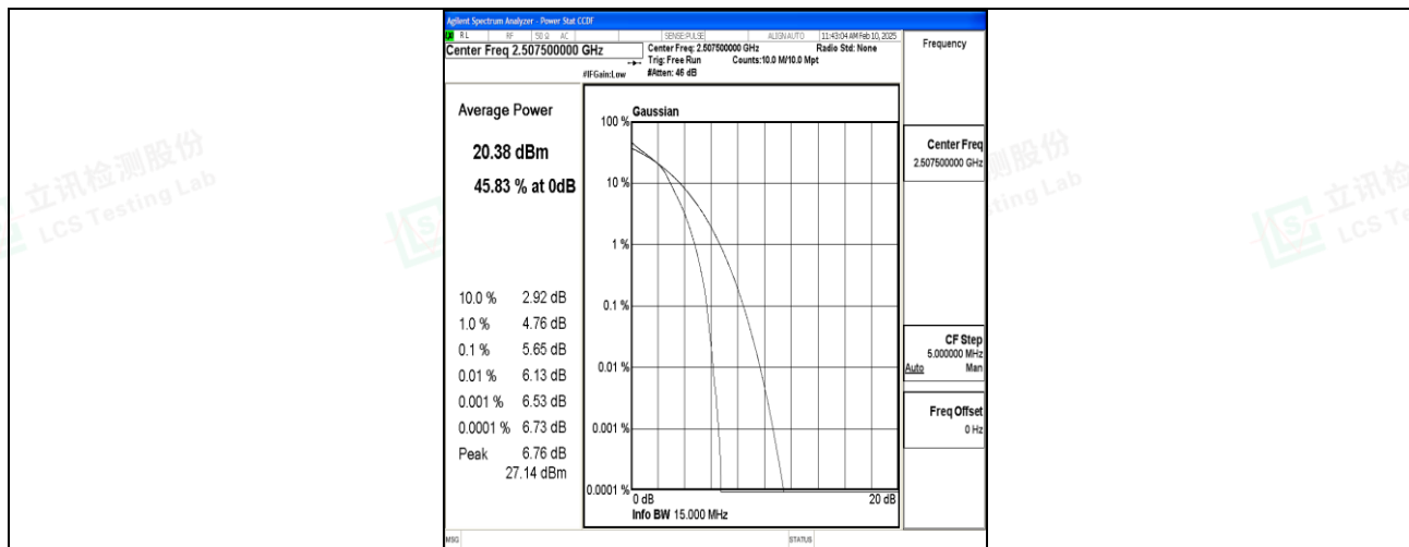
Band7-15MHz-16QAM-20825-75RB#0-PASS
