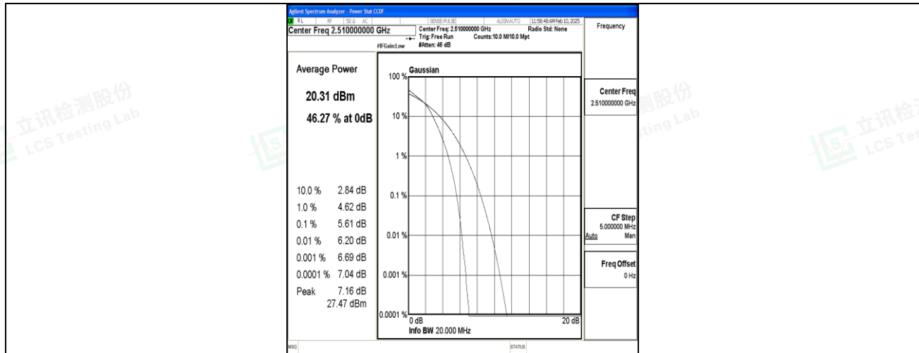
Band7-20MHz-16QAM-20850-100RB#0-PASS
