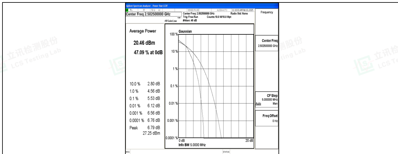
Band7-5MHz-16QAM-20775-25RB#0-PASS
