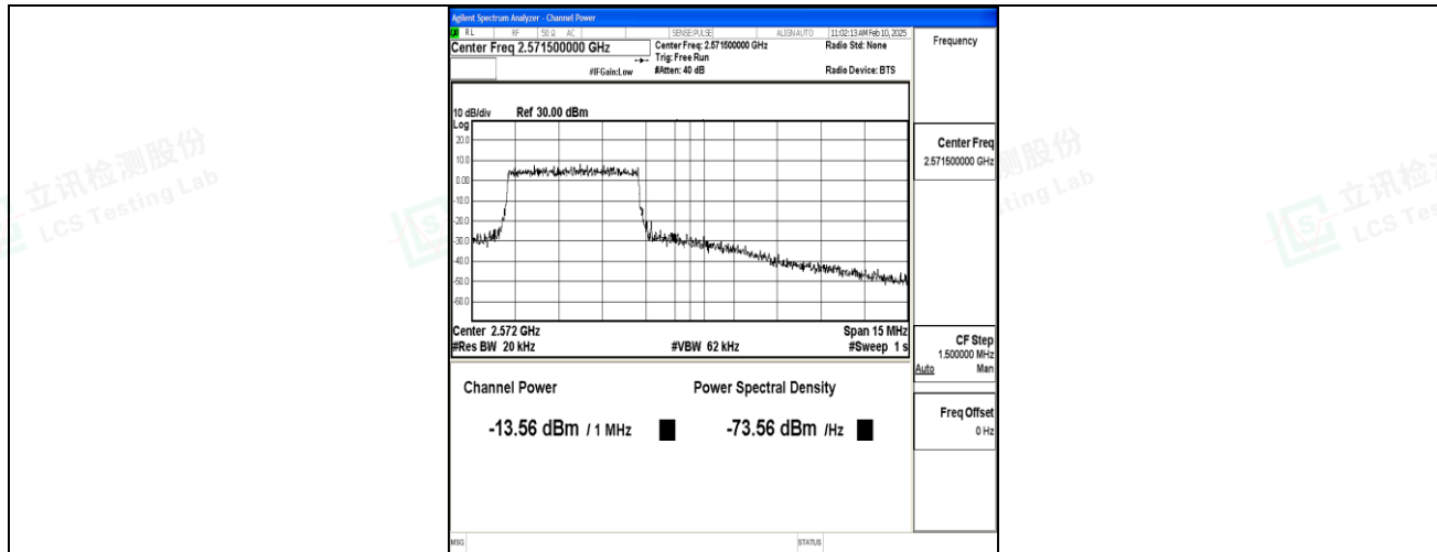
Band7_5MHz_16QAM_21425_25RB#0_Final2
