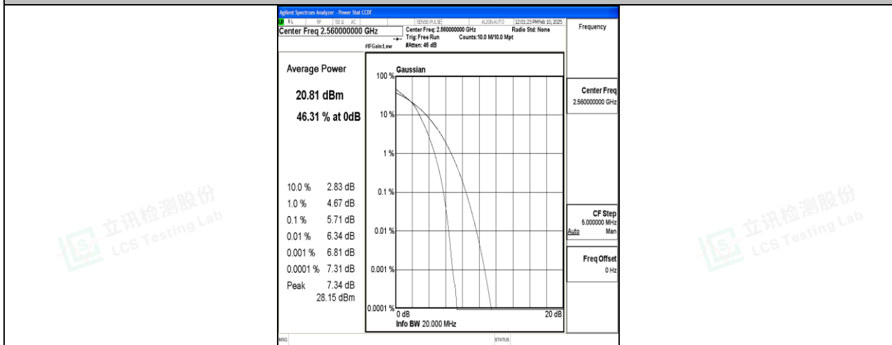
Band7-20MHz-16QAM-21350-100RB#0-PASS
