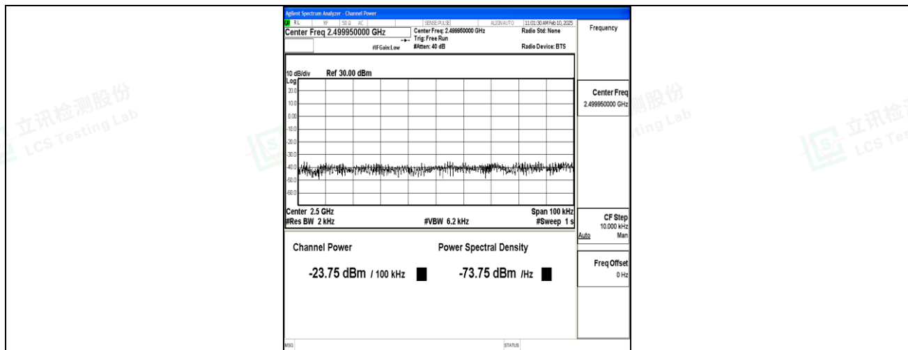
Band7_5MHz_QPSK_20775_25RB#0_Final2
