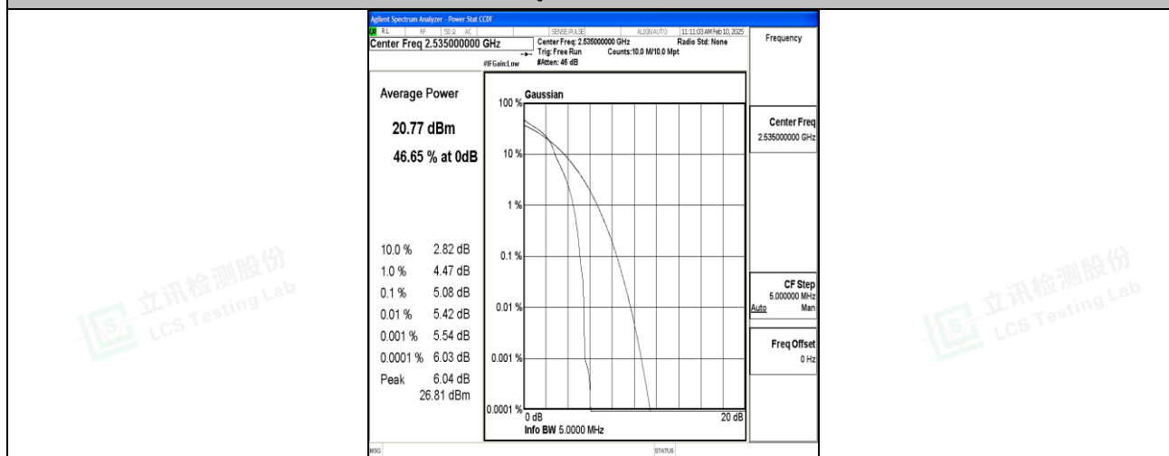
Band7-5MHz-16QAM-21100-1RB#0-PASS
