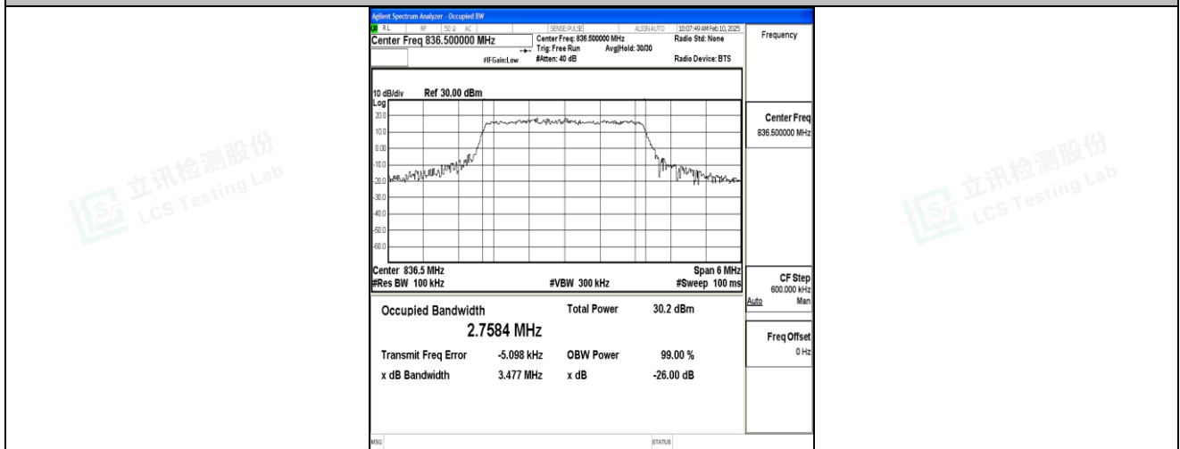
Band5-3MHz-QPSK-20525-15RB#0-PASS
