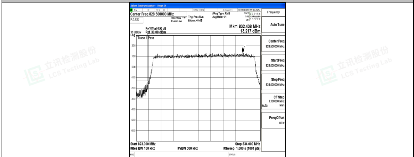
Band5_10MHz_QPSK_20450_50RB#0
