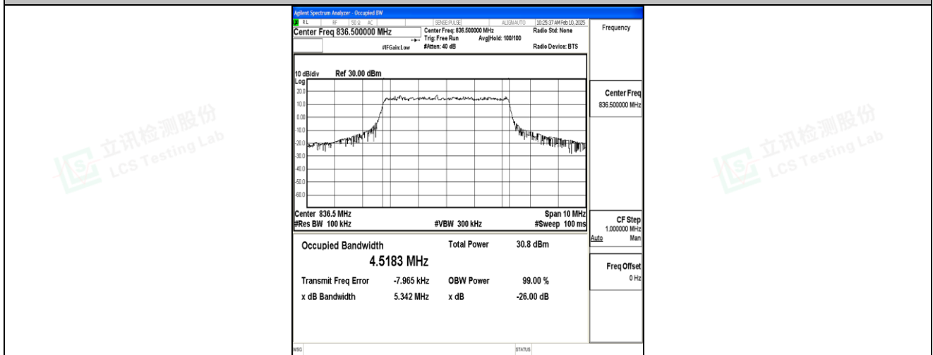
Band5-5MHz-QPSK-20525-25RB#0-PASS
