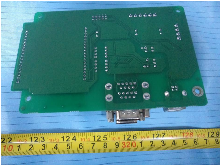
EUT – RF Module Board 1 Bottom View
