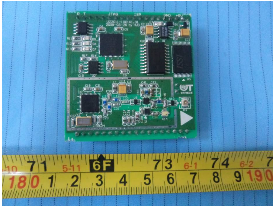
EUT – RF Module Board 2 Top View
