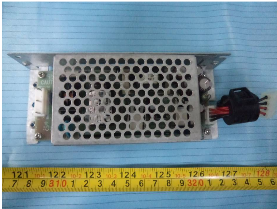
EUT –Power Board with Shielding View
