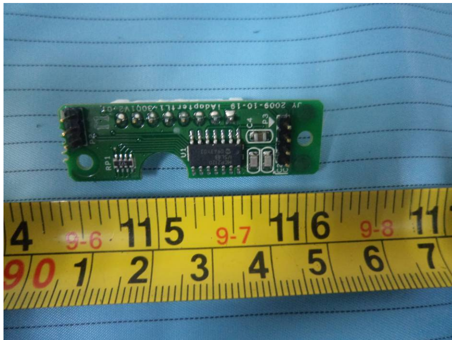
EUT – E2044060-1 Board Bottom View
