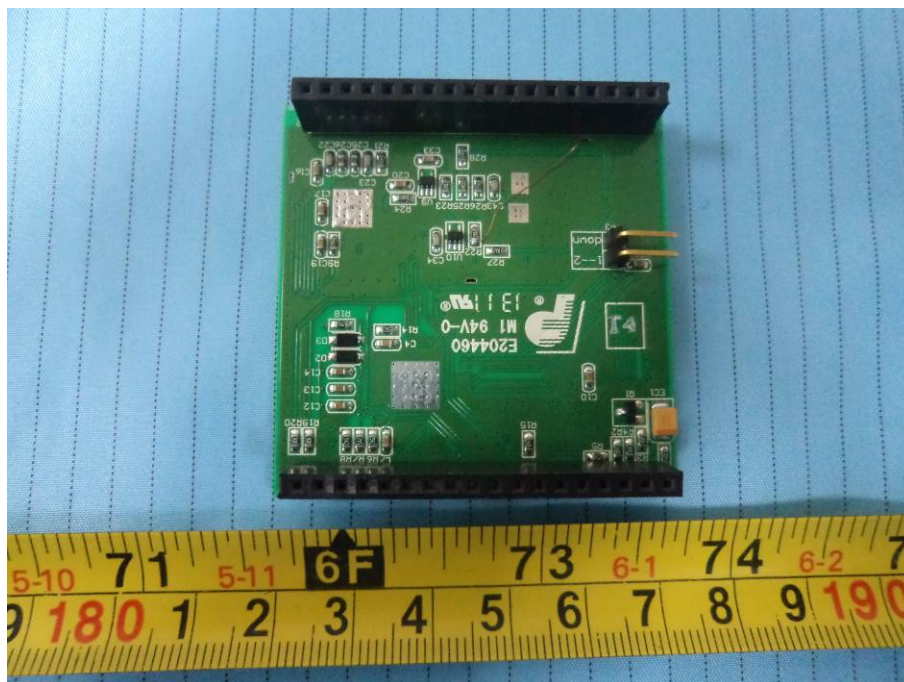
EUT – RF Module Board 2 Bottom View
