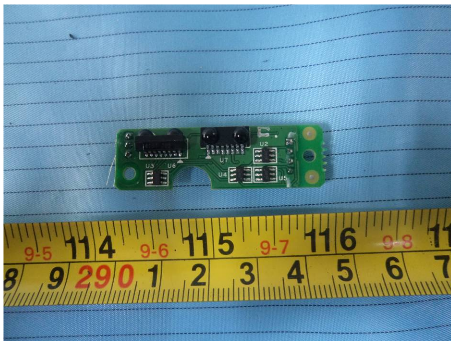
EUT – E2044060-2 Board Bottom View
