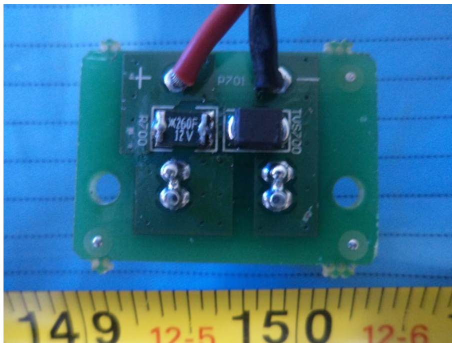
EUT – Charging Interface Board bottom View
