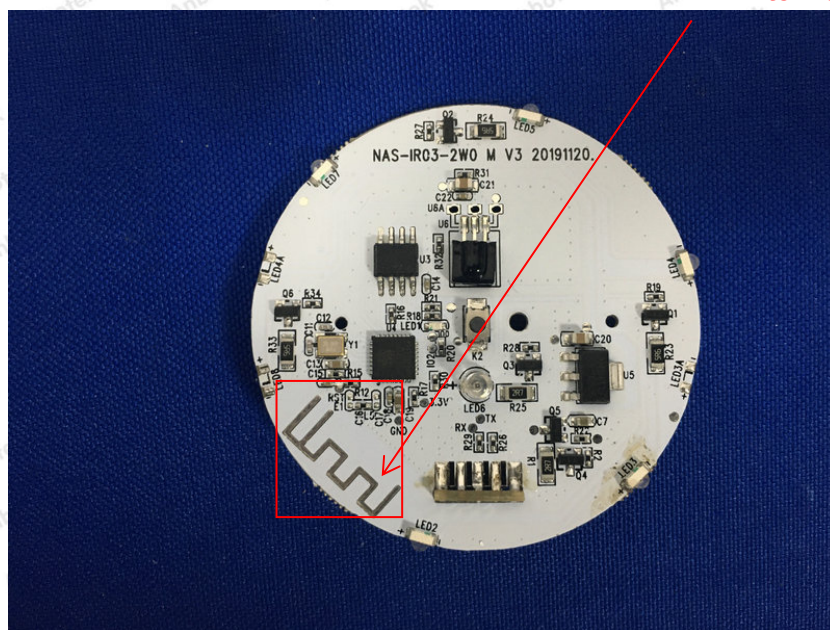
WIFI Antenna
