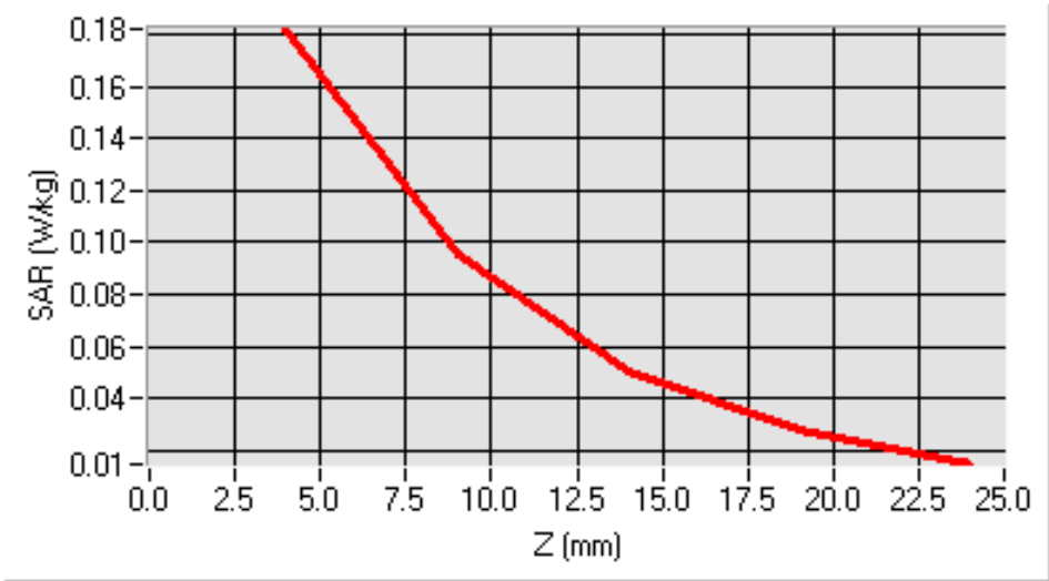
SAR, Z Axis Scan (X = -47, Y = -42)
