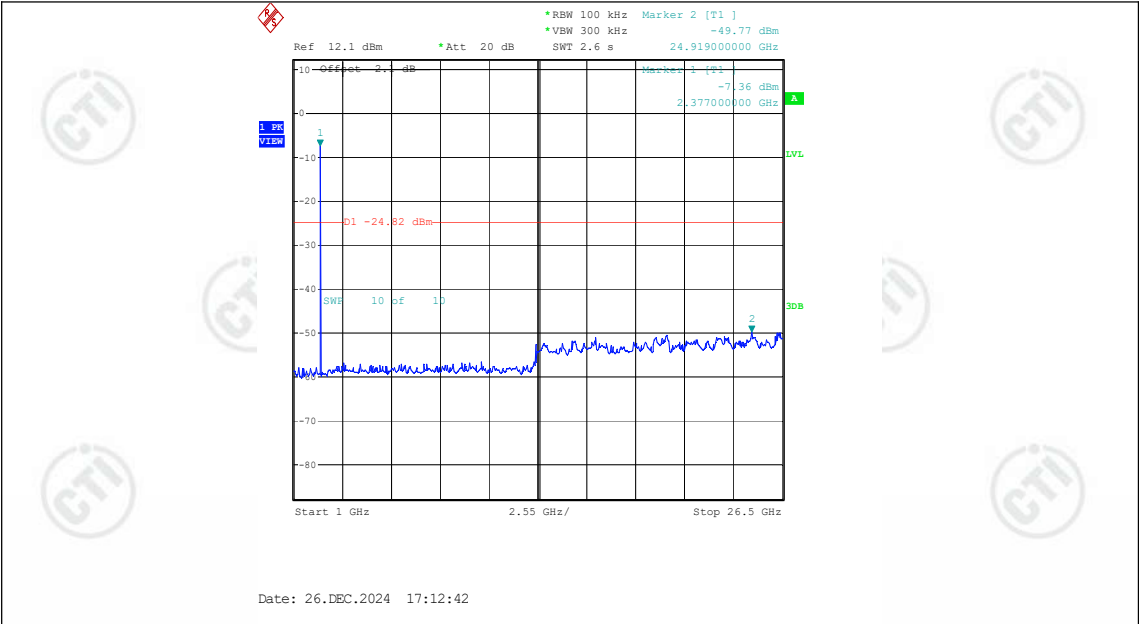
Zigbee-Ant1-2405-1000~26500-PASS
