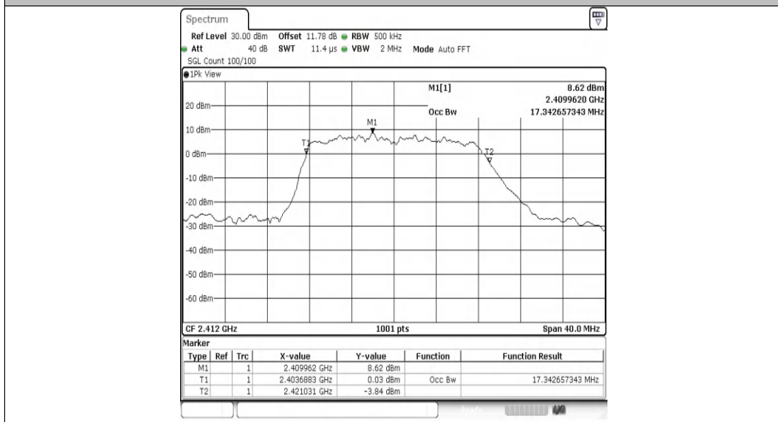
11G-Ant1-2412
